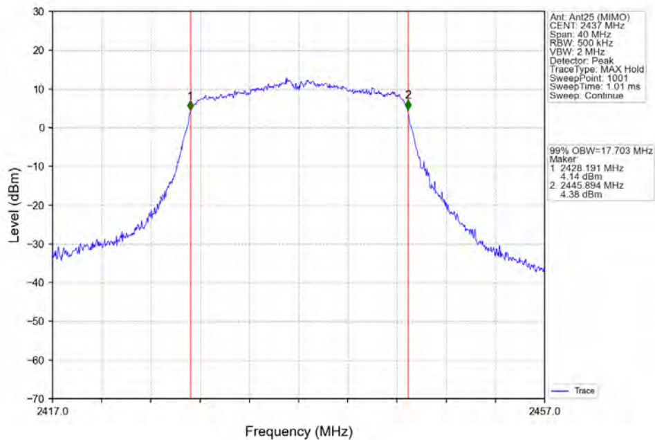
802.11ac(VHT20) MCH 2437MHz Ant25 (MIMO) NTN
