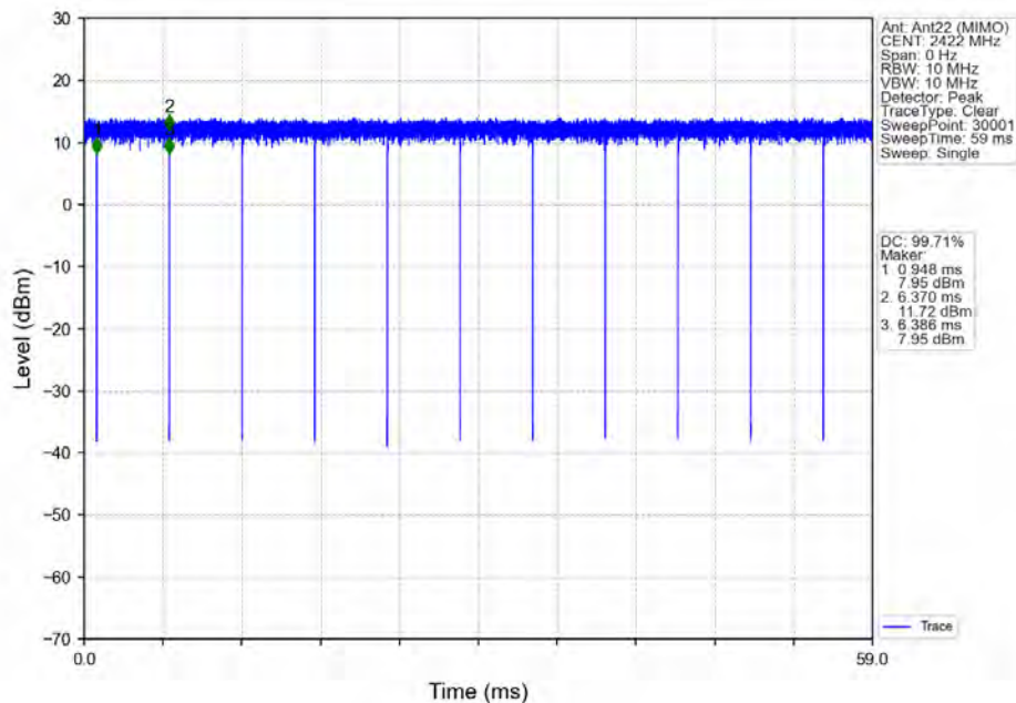
802.11n(HT40)_LCH_2422MHz_Ant22 (MIMO)_NTNV
