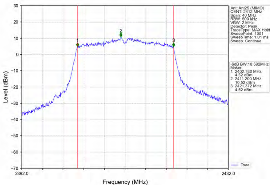
802.11ax(HEW20) LCH 2412MHz RU242 Left Ant25 (MIMO) NTN
