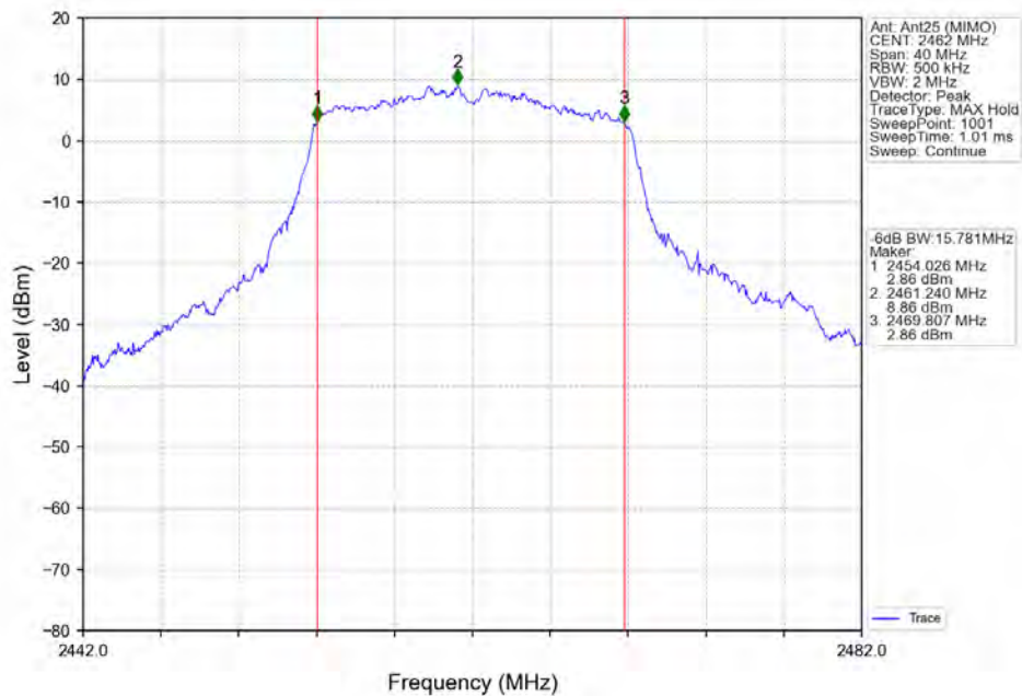
802.11g_HCH_2462MHz_Ant25 (MIMO)_NTNV
