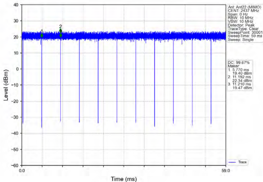
802.11ac(VHT20)_MCH_2437MHz_Ant22 (MIMO)_NTNV
