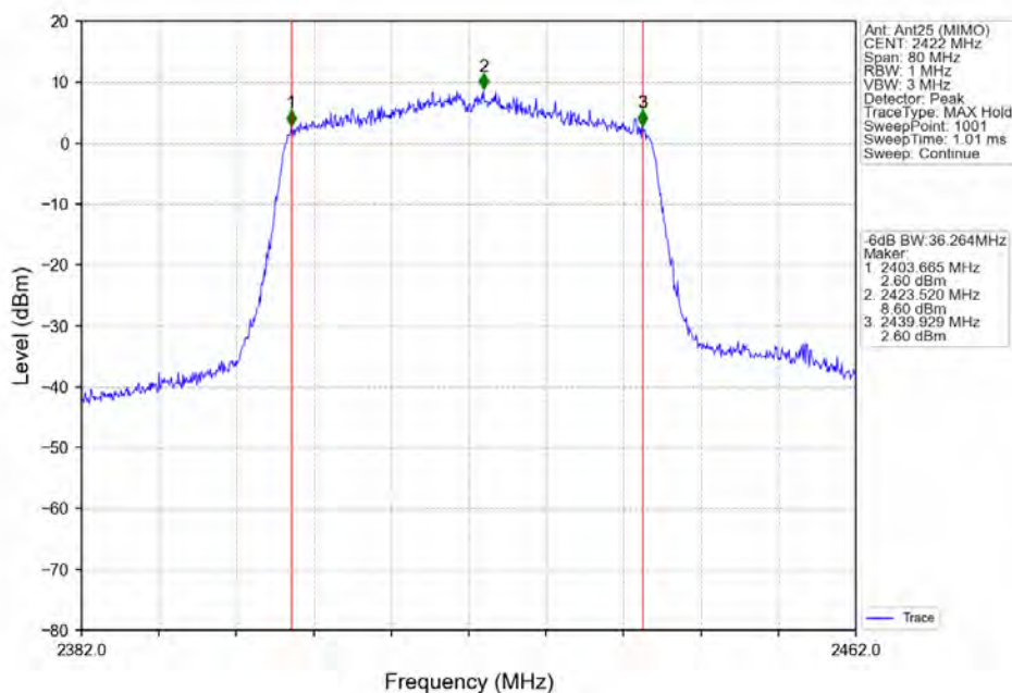
802.11ax(HEW40) LCH 2422MHz RU484 Left Ant25 (MIMO) NTN
