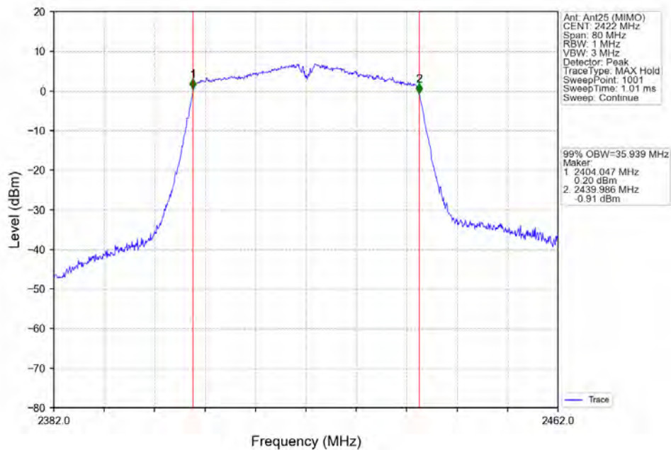
802.11ac(VHT40)_LCH_2422MHz_Ant25 (MIMO)_NTNV
