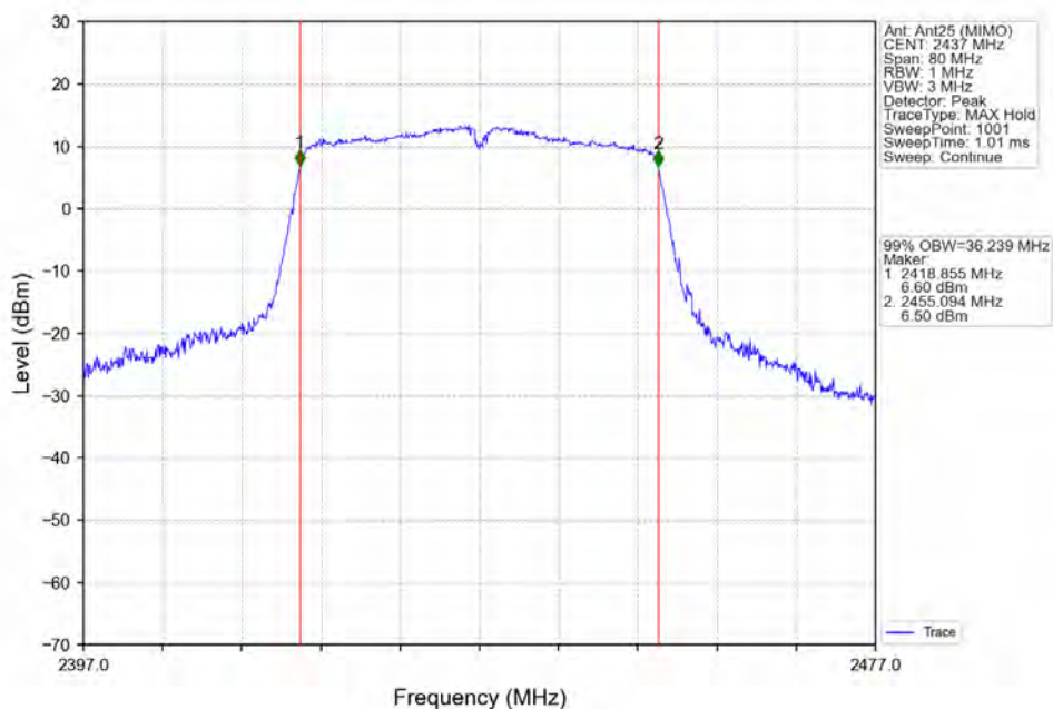
802.11ac(VHT40)_MCH_2437MHz_Ant25 (MIMO)_NTNV
