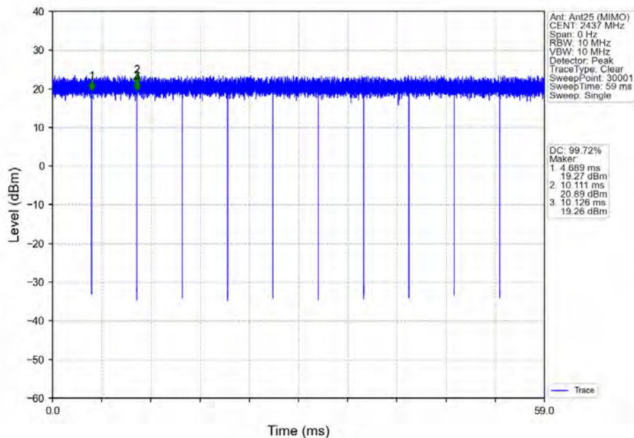
802.11ac(VHT20)_MCH_2437MHz_Ant25 (MIMO)_NTNV
