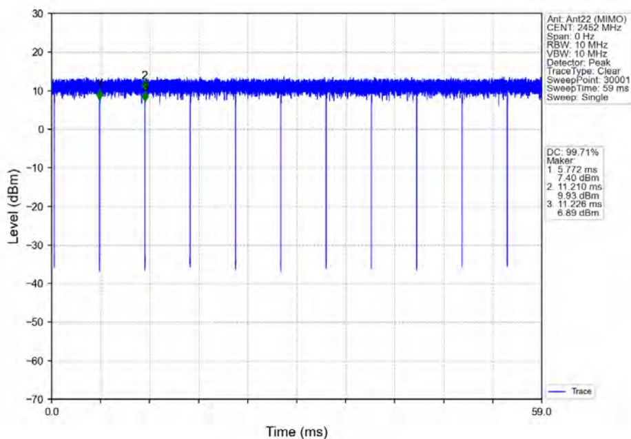
802.11ax(HEW40) HCH 2452MHz RU484 Left Ant22 (MIMO) NTN
