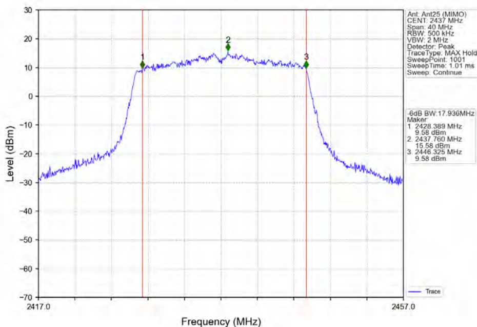
802.11ax(HEW20) MCH 2437MHz RU242 Left Ant25 (MIMO) NTN
