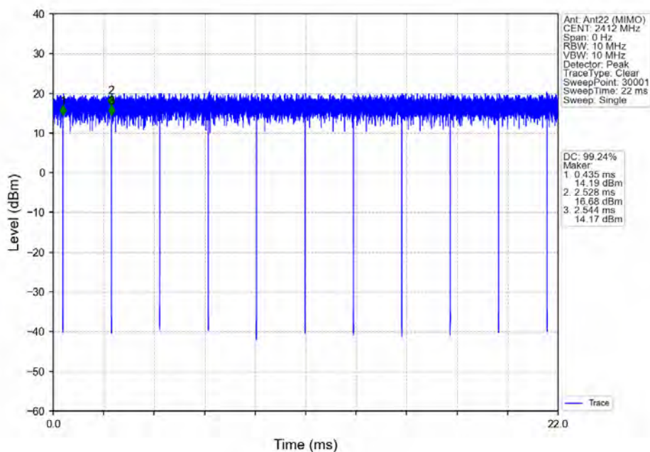
802.11g_LCH_2412MHz_Ant22 (MIMO) NTN
