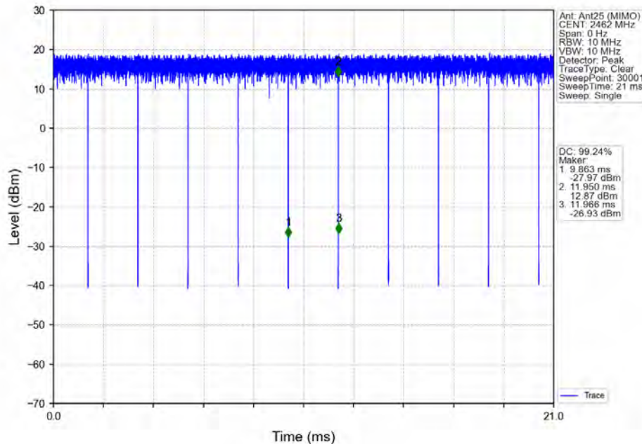
802.11g_HCH_2462MHz_Ant25 (MIMO)_NTNV
