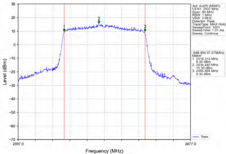
802.11ax(HEW40) MCH 2437MHz RU484 Left Ant25 (MIMO) NTN
