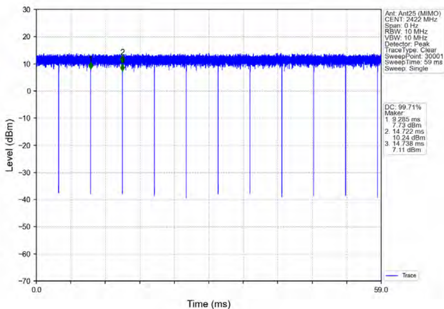
802.11ax(HEW40) LCH 2422MHz RU484 Left Ant25 (MIMO) NTN
