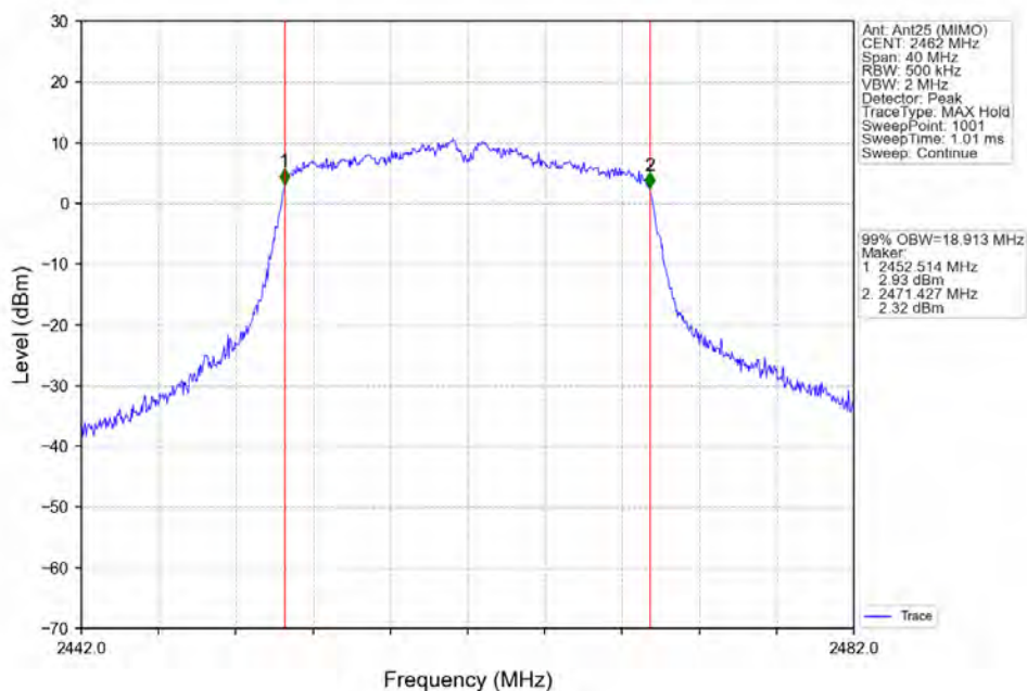
802.11ax(HEW20) HCH 2462MHz RU242 Left Ant25 (MIMO) NTN
