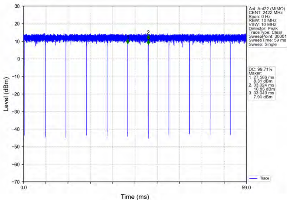
802.11ax(HEW40) LCH 2422MHz RU484 Left Ant22 (MIMO) NTN
