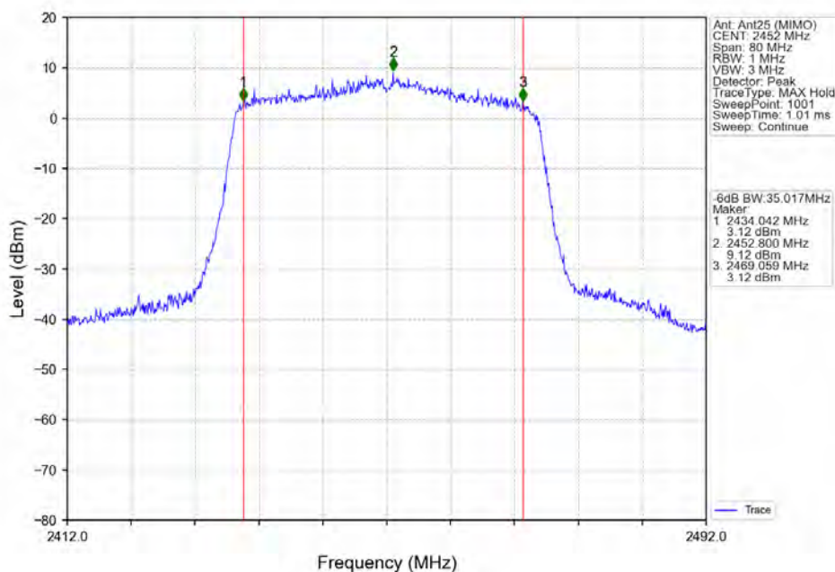
802.11ax(HEW40) HCH 2452MHz RU484 Left Ant25 (MIMO) NTN
