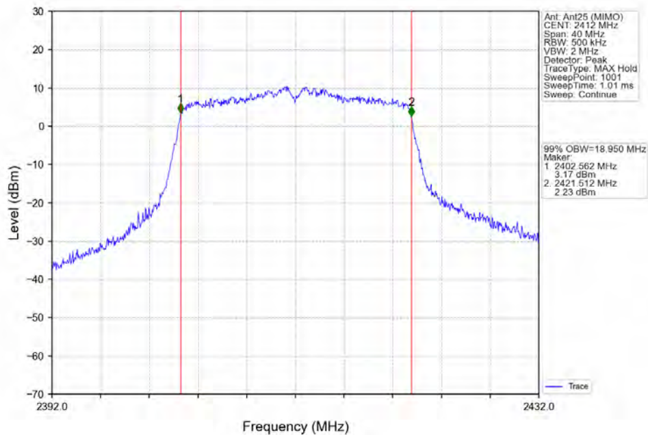
802.11ax(HEW20) LCH_2412MHz_RU242_Left_Ant25 (MIMO) NTN
