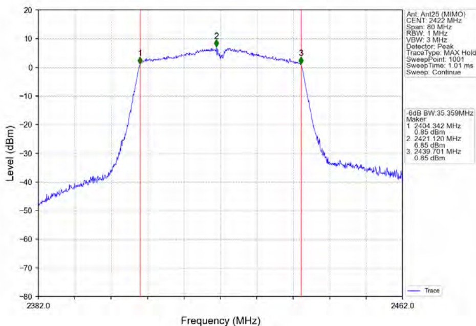
802.11ac(VHT40)_LCH_2422MHz_Ant25 (MIMO)_NTNV
