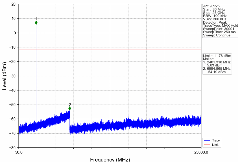
2M_LCH_2402MHz_Ant25_NTNV
