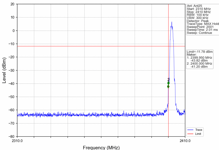
2M_LCH_2402MHz_Ant25_NTNV
