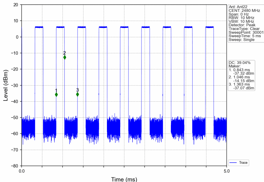
2M_HCH_2480MHz_Ant22_NTNV
