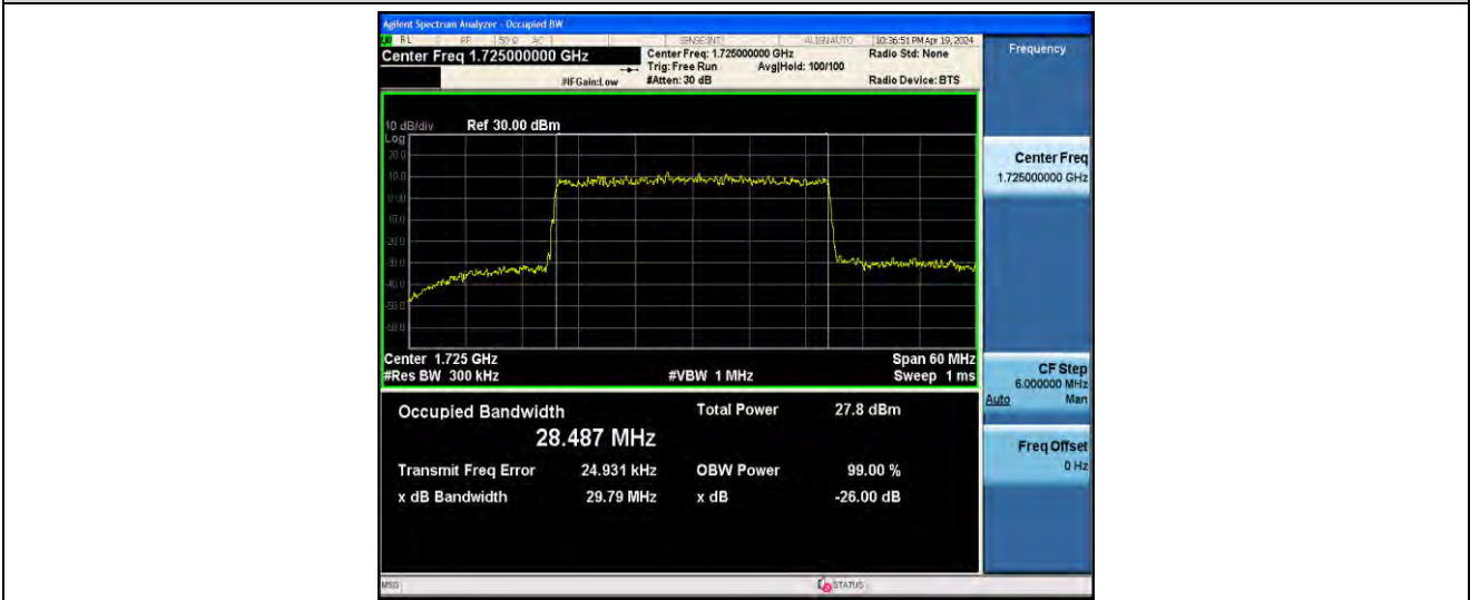
1-N66-PC3-15-30-L-5-DFT-256QAM-Outer_Full-160@0-ANT41-28.487-29.79-≤30-PASS
