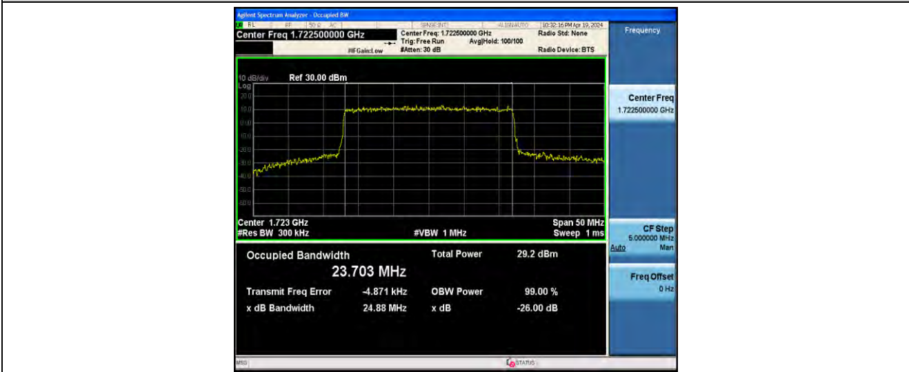
1-N66-PC3-15-25-L-6-CP-QPSK-Outer_Full-133@0-ANT41-23.703-24.88-<=25-PASS
