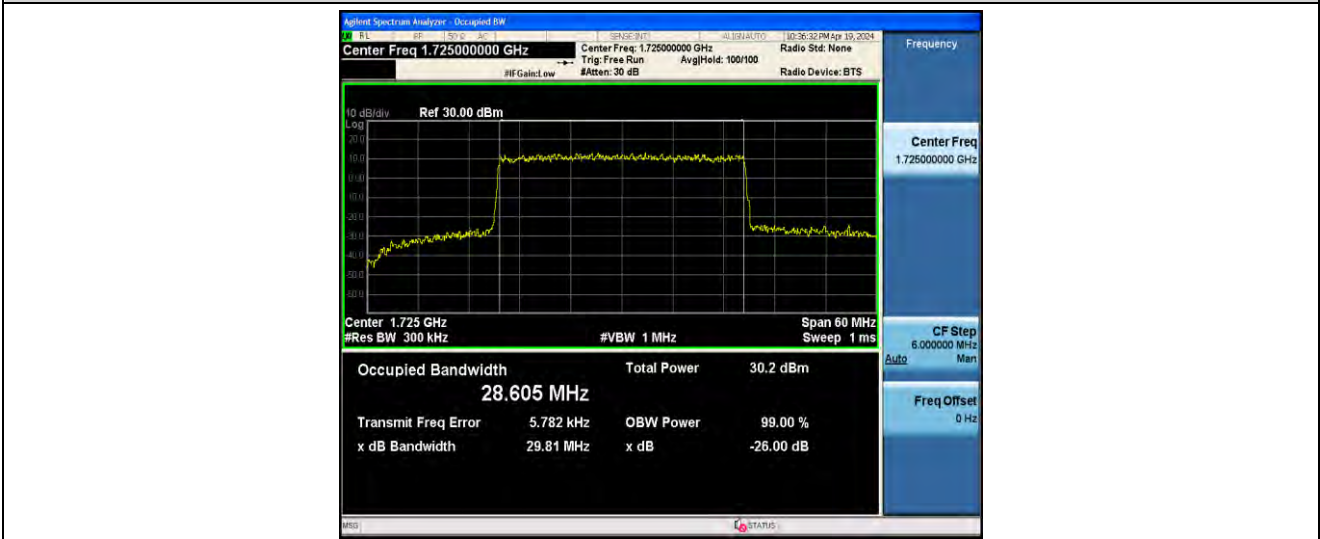
1-N66-PC3-15-30-L-3-DFT-16QAM-Outer_Full-160@0-ANT41-28.605-29.81-≤30-PASS
