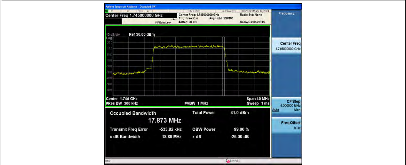
1-N66-PC3-15-20-M-2-DFT-PI2BPSK-Outer_Full-100@0-ANT41-17.873-18.89-≤20-PASS
