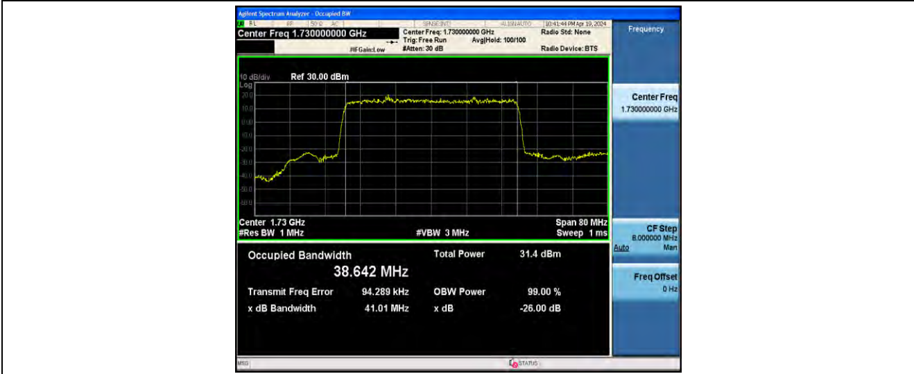
1-N66-PC3-15-40-L-2-DFT-PI2BPSK-Outer_Full-216@0-ANT41-38.642-41.01-≤40-PASS
