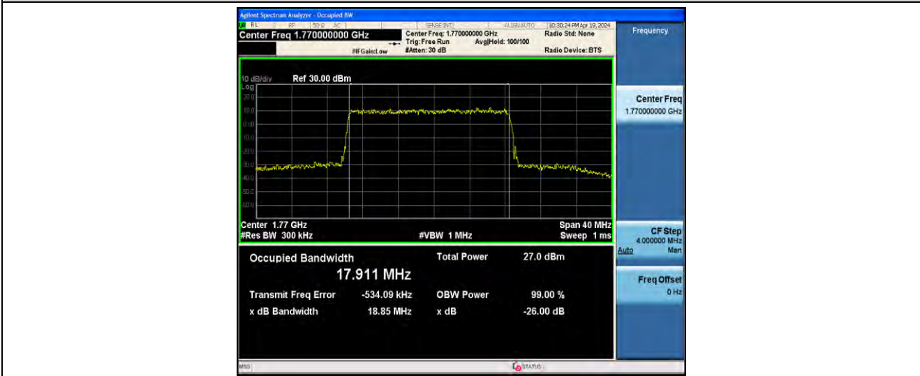
1-N66-PC3-15-20-H-5-DFT-256QAM-Outer_Full-100@0-ANT41-17.911-18.85-≤20-PASS
