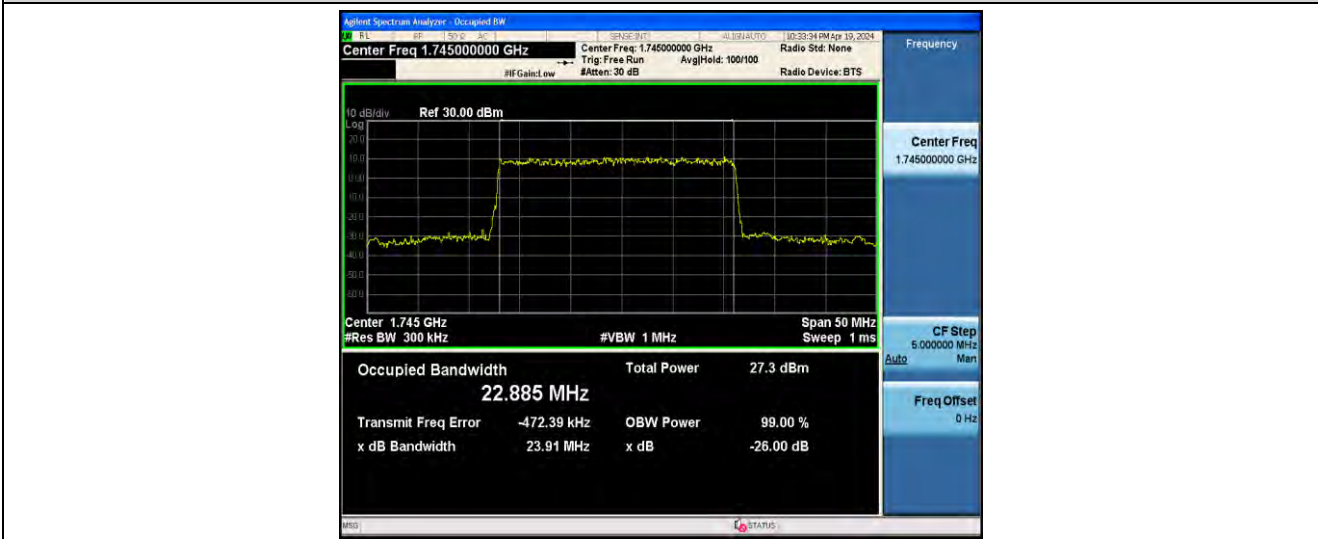
1-N66-PC3-15-25-M-5-DFT-256QAM-Outer_Full-128@0-ANT41-22.885-23.91-≤25-PASS
