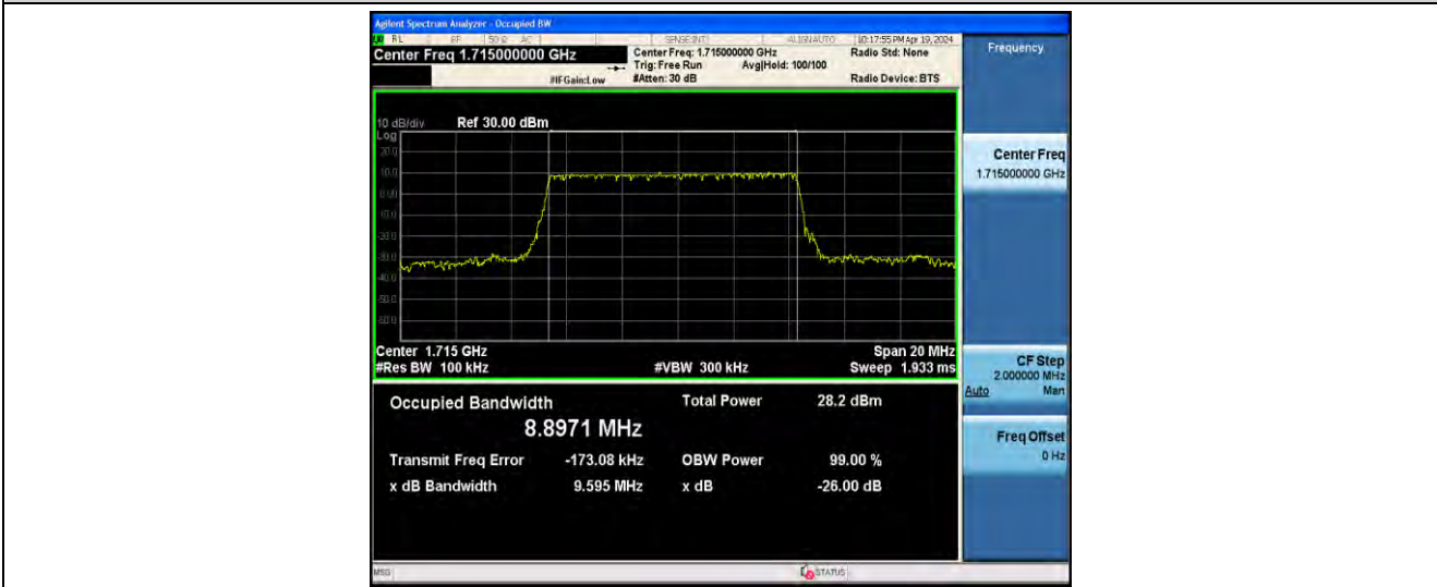
1-N66-PC3-15-10-L-5-DFT-256QAM-Outer_Full-50@0-ANT41-8.8971-9.595-≤10-PASS
