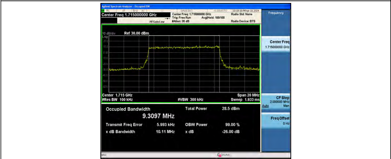
1-N66-PC3-15-10-L-7-CP-16QAM-Outer_Full-52@0-ANT41-9.3097-10.11-≤10-PASS
