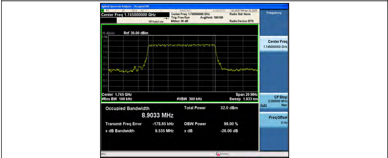
1-N66-PC3-15-10-M-2-DFT-PI2BPSK-Outer_Full-50@0-ANT41-8.9033-9.535-≤10-PASS
