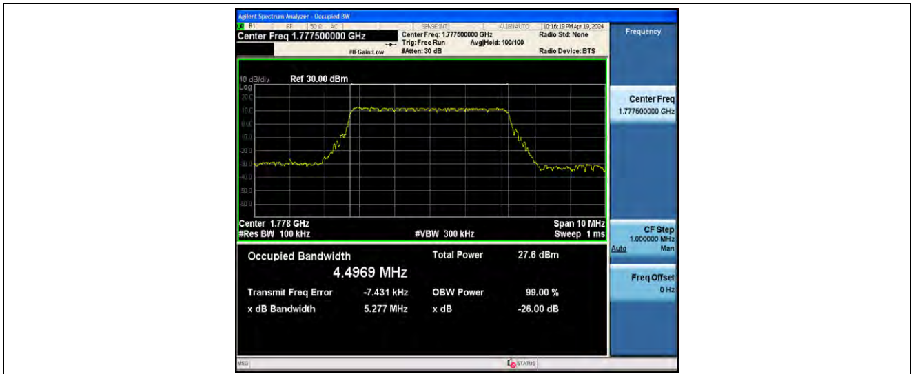
1-N66-PC3-15-5-H-5-DFT-256QAM-Outer_Full-25@0-ANT41-4.4969-5.277-≤5-PASS
