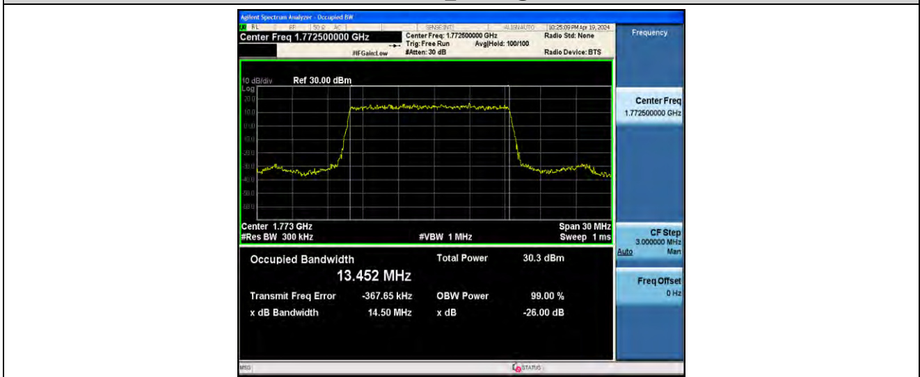
1-N66-PC3-15-15-H-2-DFT-PI2BPSK-Outter_Full-75@0-ANT41-13.452-14.50-≤15-PASS
