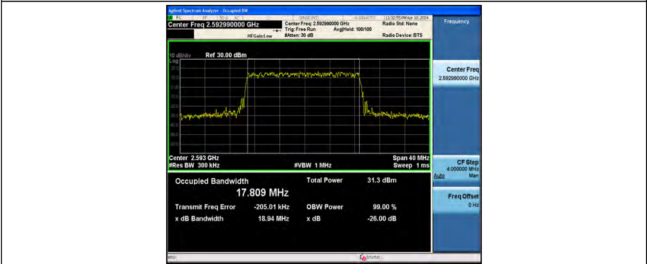
1-N41-PC2-30-20-M-1-DFT-QPSK-Outer_Full-50@0-ANT41-17.809-18.94-<math>\leq 20</math>-PASS
