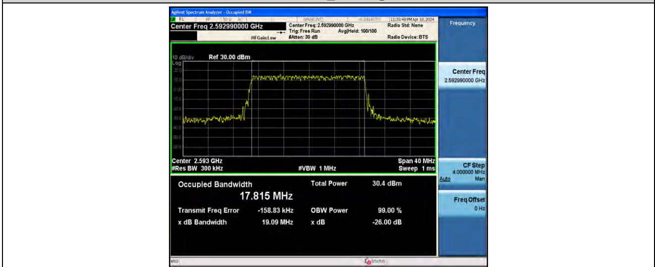
1-N41-PC2-30-20-M-3-DFT-16QAM-Outer_Full-50@0-ANT41-17.815-19.09-≤20-PASS
