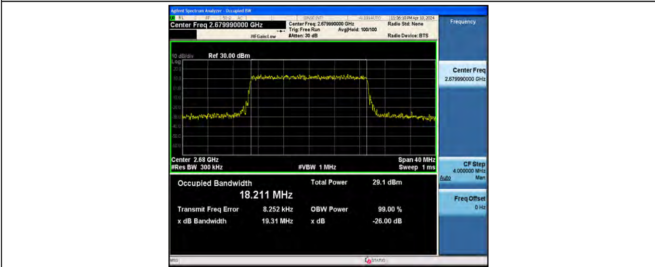
1-N41-PC2-30-20-H-6-CP-QPSK-Outer_Full-51@0-ANT41-18.211-19.31-<20-PASS
