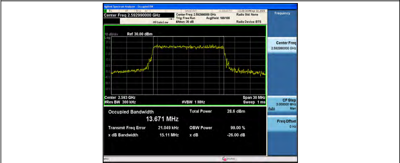
1-N41-PC2-30-15-M-8-CP-64QAM-Outer_Full-38@0-ANT41-13.671-15.11-≤15-PASS
