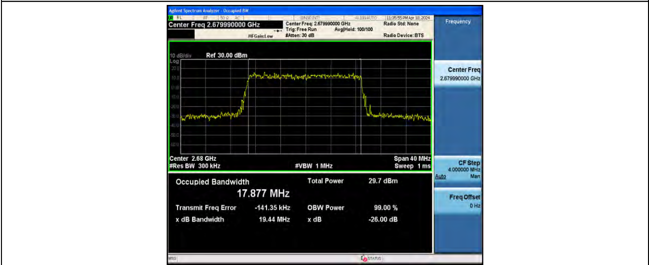
1-N41-PC2-30-20-H-4-DFT-64QAM-Outer_Full-50@0-ANT41-17.877-19.44-≤20-PASS
