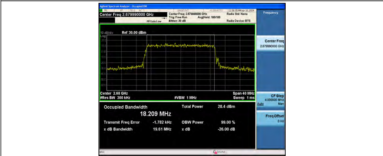
1-N41-PC2-30-20-H-8-CP-64QAM-Outer_Full-51@0-ANT41-18.209-19.61-<20-PASS
