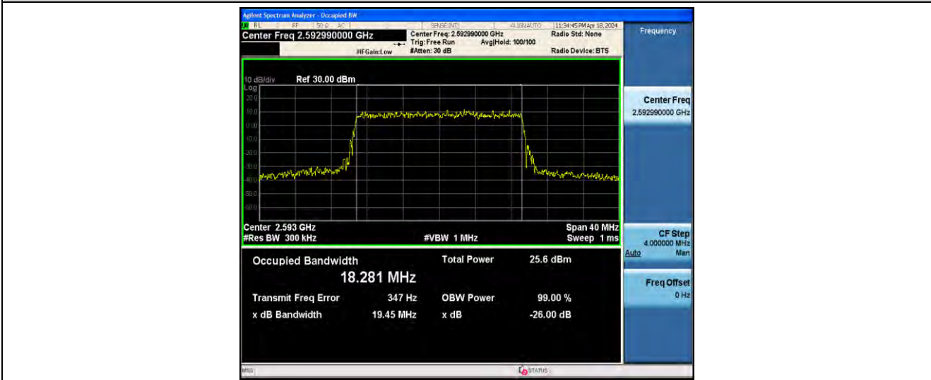
1-N41-PC2-30-20-M-9-CP-256QAM-Outer_Full-51@0-ANT41-18.281-19.45-≤20-PASS
