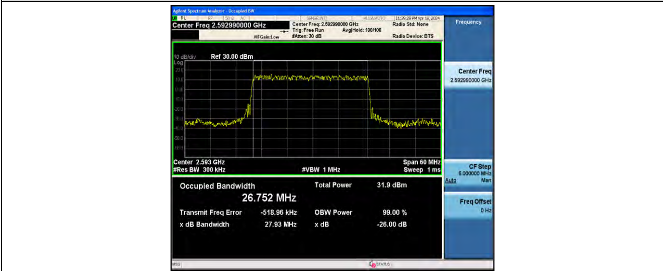
1-N41-PC2-30-30-M-2-DFT-PI2BPSK-Outer_Full-75@0-ANT41-26.752-27.93-≤30-PASS
