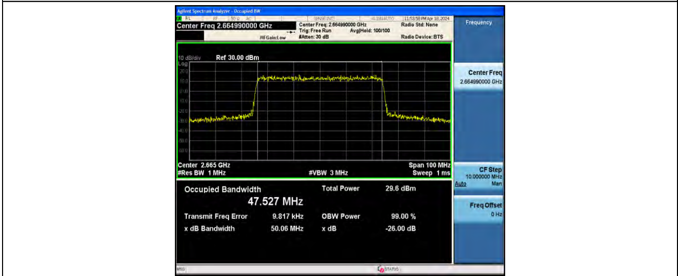
1-N41-PC2-30-50-H-7-CP-16QAM-Outer_Full-133@0-ANT41-47.527-50.06-≤50-PASS
