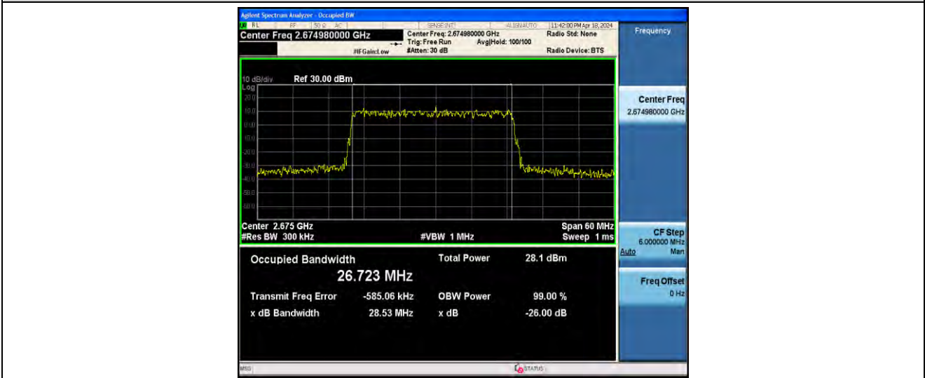
1-N41-PC2-30-30-H-5-DFT-256QAM-Outer_Full-75@0-ANT41-26.723-28.53-<30-PASS
