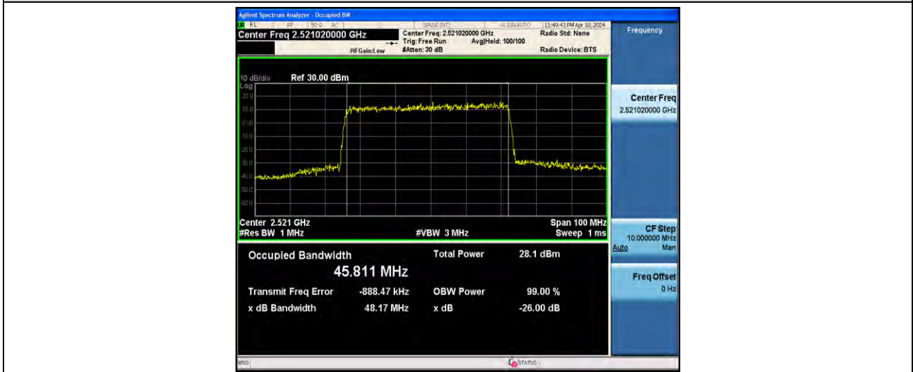
1-N41-PC2-30-50-L-5-DFT-256QAM-Outer_Full-128@0-ANT41-45.811-48.17-≤50-PASS
