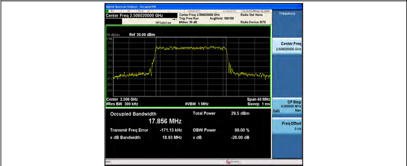
1-N41-PC2-30-20-L-4-DFT-64QAM-Outer_Full-50@0-ANT41-17.856-18.93-≤20-PASS
