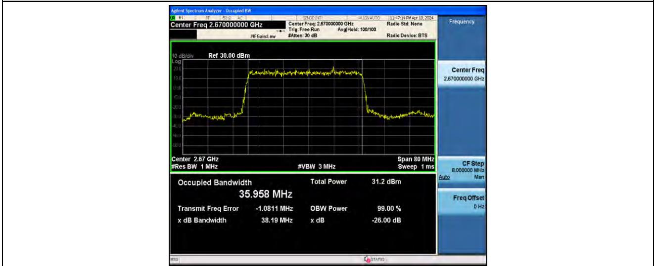
1-N41-PC2-30-40-H-2-DFT-PI2BPSK-Outer_Full-100@0-ANT41-35.958-38.19-<40-PASS
