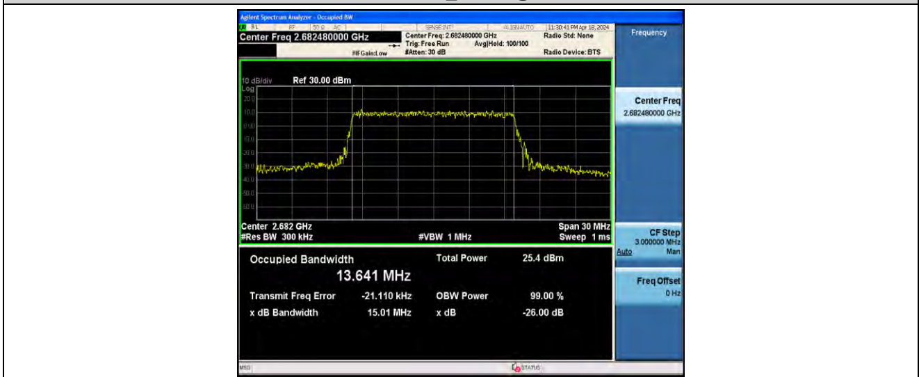
1-N41-PC2-30-15-H-9-CP-256QAM-Outer_Full-38@0-ANT41-13.641-15.01-≤15-PASS
