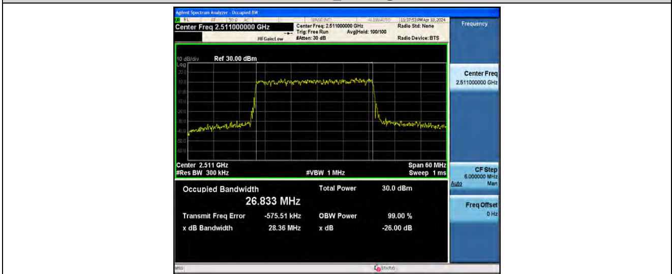
1-N41-PC2-30-30-L-3-DFT-16QAM-Outer_Full-75@0-ANT41-26.833-28.36-<30-PASS
