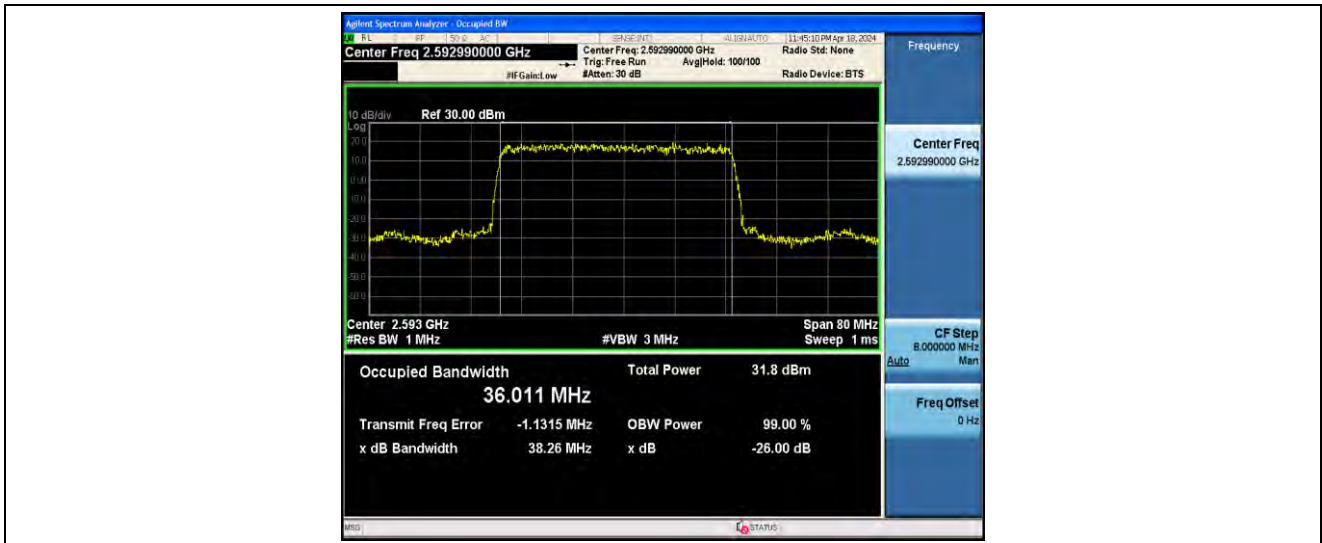
1-N41-PC2-30-40-M-2-DFT-PI2BPSK-Outer_Full-100@0-ANT41-36.011-38.26-<40-PASS
