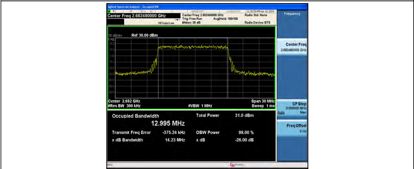
1-N41-PC2-30-15-H-1-DFT-QPSK-Outer_Full-36@0-ANT41-12.995-14.23-≤15-PASS
