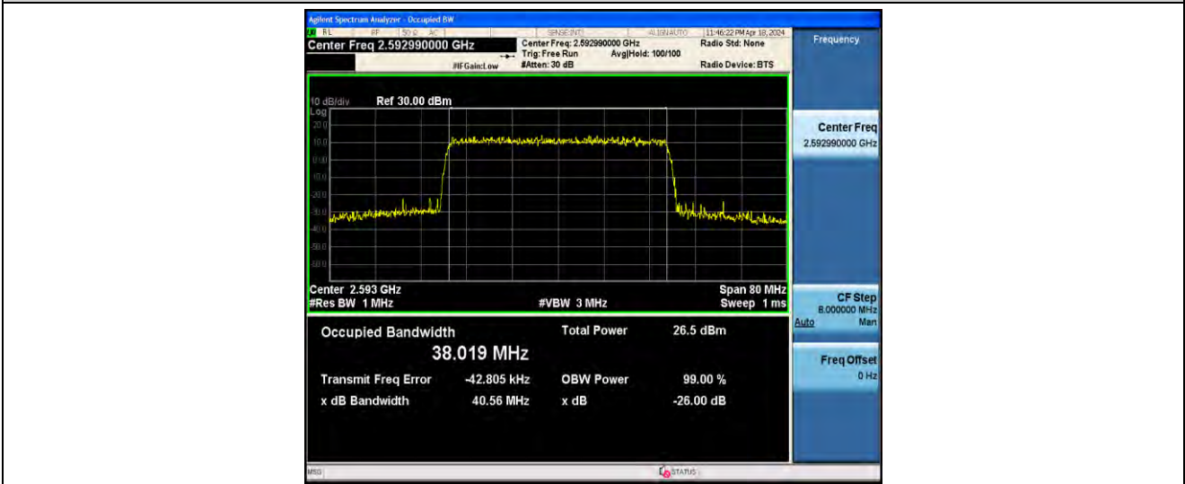
1-N41-PC2-30-40-M-9-CP-256QAM-Outer_Full-106@0-ANT41-38.019-40.56-≤40-PASS
