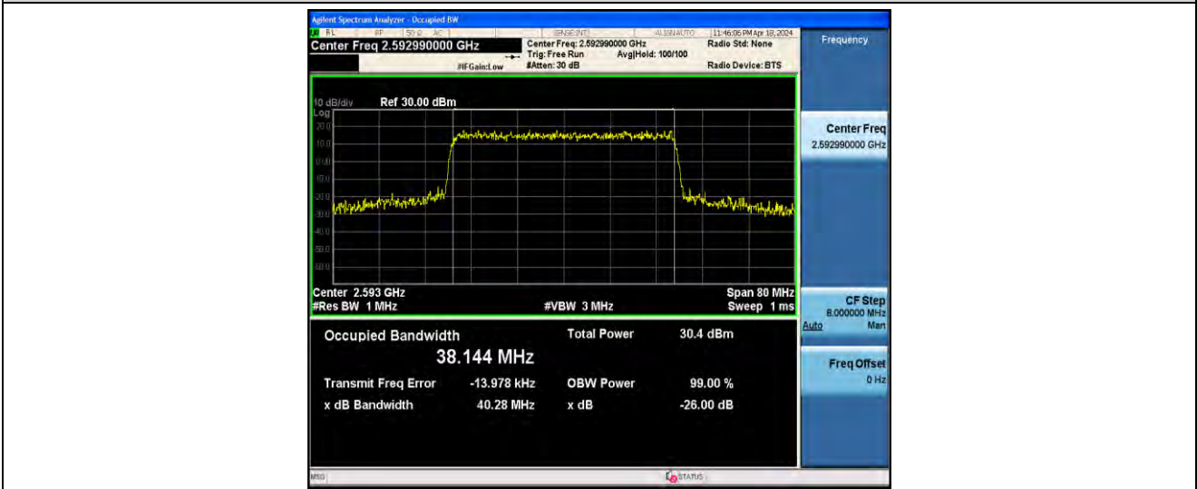
1-N41-PC2-30-40-M-7-CP-16QAM-Outer_Full-106@0-ANT41-38.144-40.28-<40-PASS
