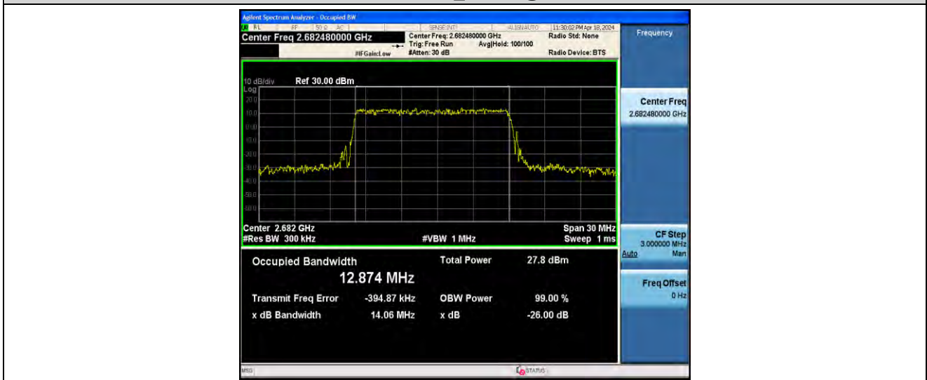
1-N41-PC2-30-15-H-5-DFT-256QAM-Outer_Full-36@0-ANT41-12.874-14.06-<=15-PASS
