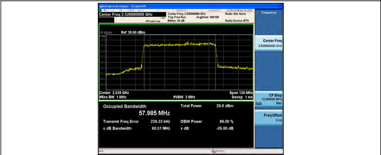
1-N41-PC2-30-60-L-4-DFT-64QAM-Outer_Full-162@0-ANT41-57.985-60.51-≤60-PASS
