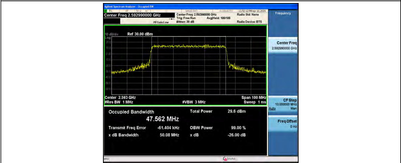
1-N41-PC2-30-50-M-8-CP-64QAM-Outer_Full-133@0-ANT41-47.562-50.08-≤50-PASS
