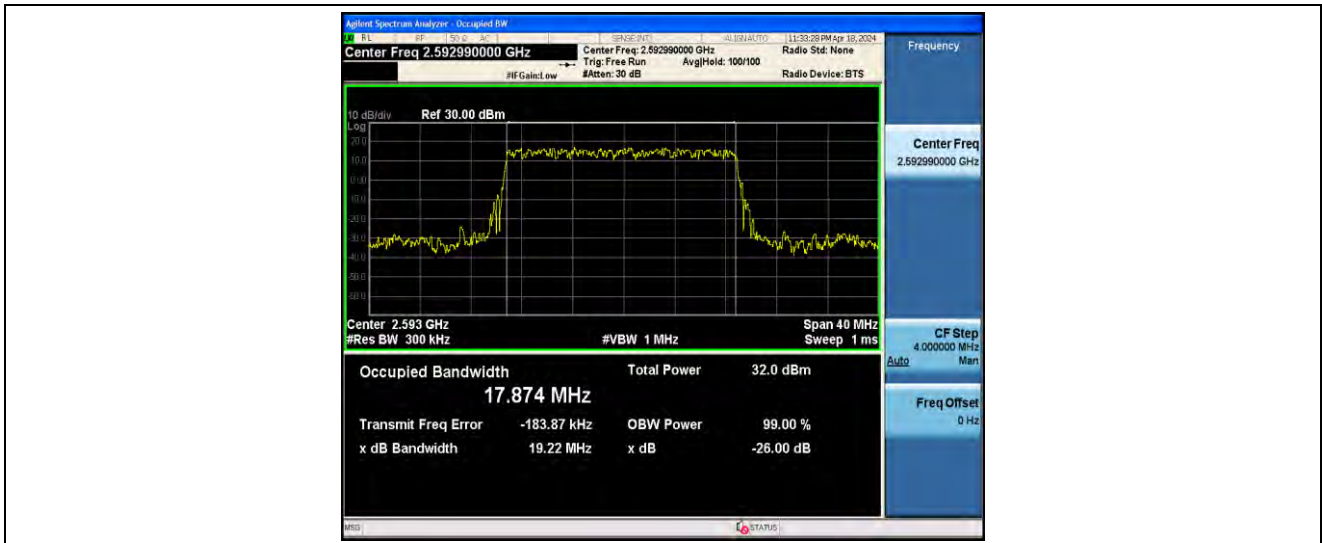
1-N41-PC2-30-20-M-2-DFT-PI2BPSK-Outer_Full-50@0-ANT41-17.874-19.22-≤20-PASS
