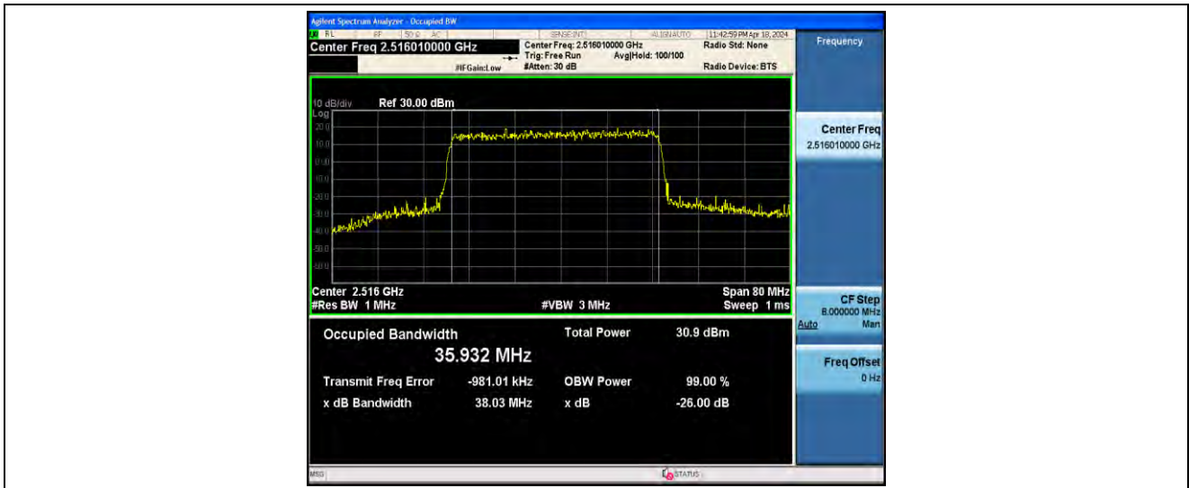
1-N41-PC2-30-40-L-1-DFT-QPSK-Outer_Full-100@0-ANT41-35.932-38.03-≤40-PASS
