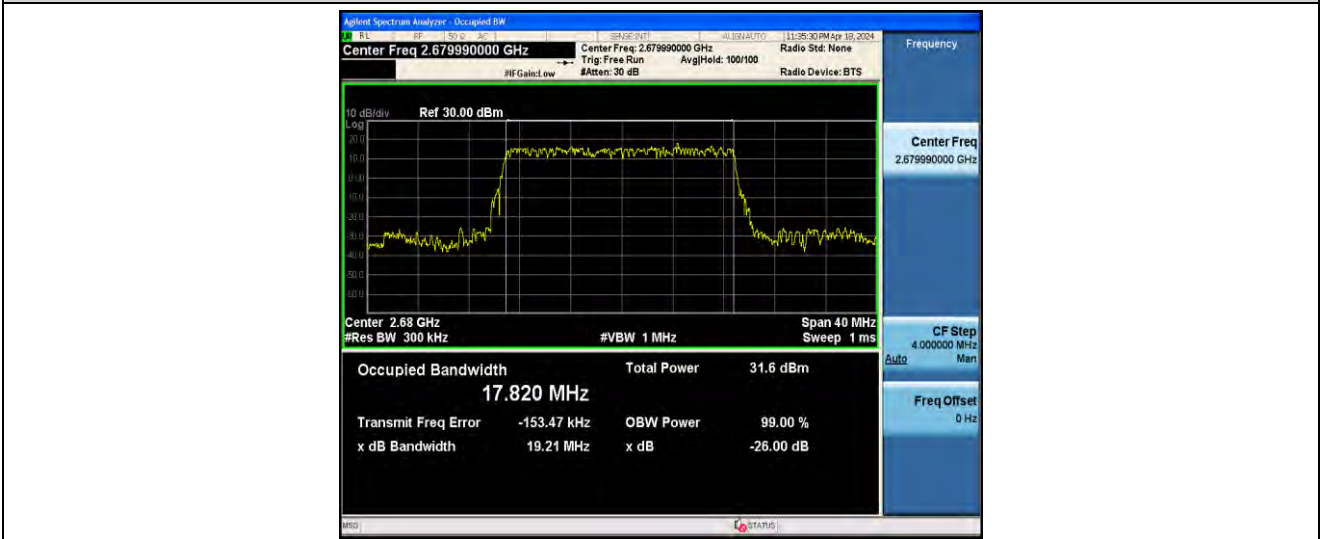
1-N41-PC2-30-20-H-2-DFT-PI2BPSK-Outer_Full-50@0-ANT41-17.820-19.21-<20-PASS
