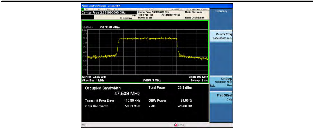
1-N41-PC2-30-50-H-9-CP-256QAM-Outer_Full-133@0-ANT41-47.539-50.01-≤50-PASS
