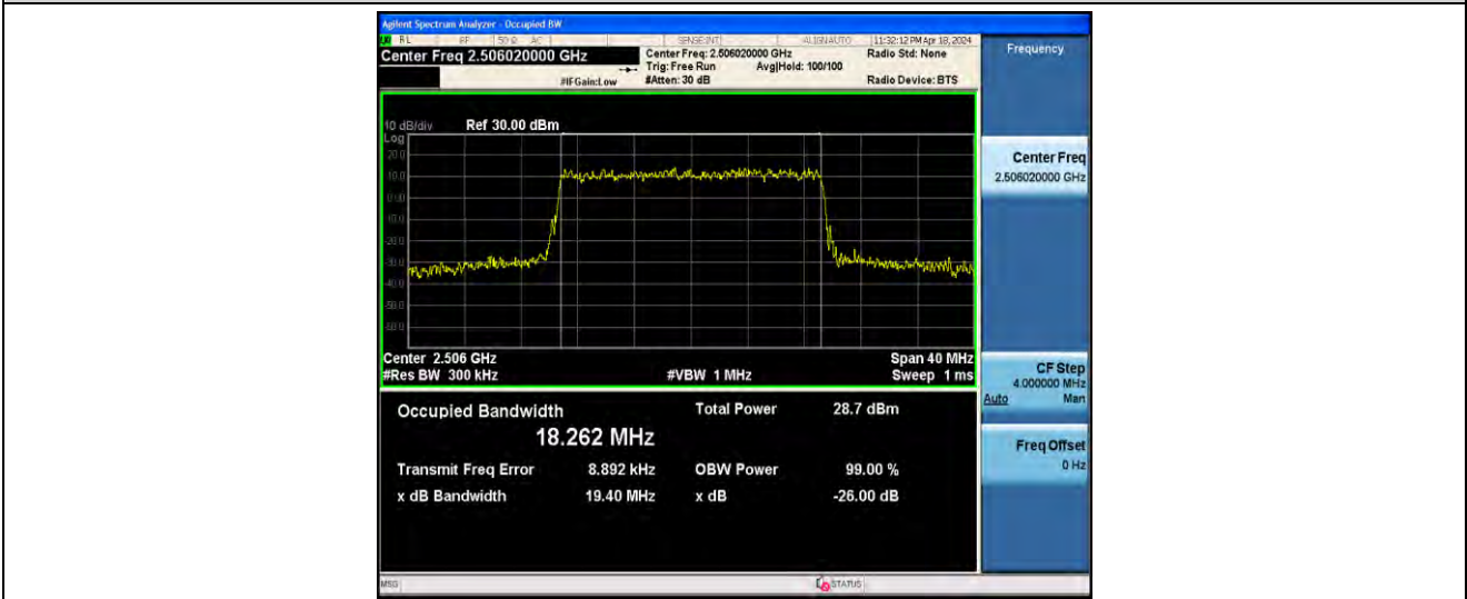
1-N41-PC2-30-20-L-6-CP-QPSK-Outer_Full-51@0-ANT41-18.262-19.40-≤20-PASS
