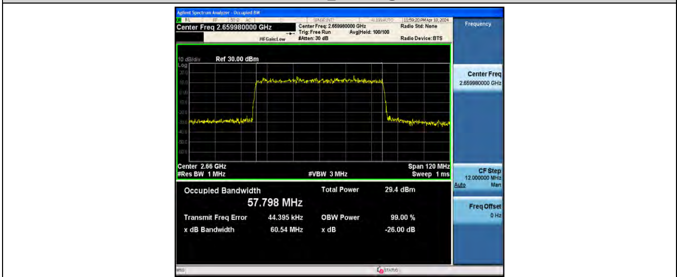
1-N41-PC2-30-60-H-4-DFT-64QAM-Outer_Full-162@0-ANT41-57.798-60.54-≤60-PASS
