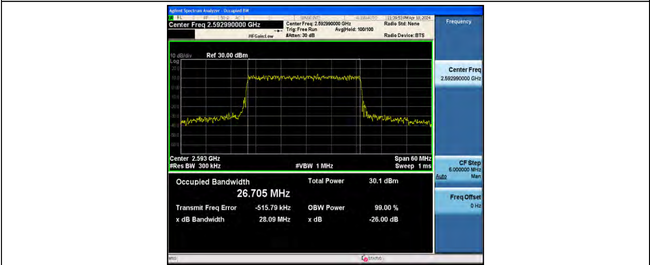
1-N41-PC2-30-30-M-4-DFT-64QAM-Outer_Full-75@0-ANT41-26.705-28.09-≤30-PASS
