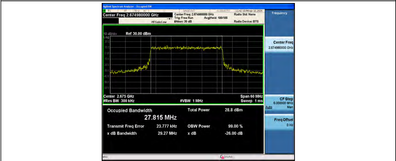
1-N41-PC2-30-30-H-7-CP-16QAM-Outer_Full-78@0-ANT41-27.815-29.27-≤30-PASS
