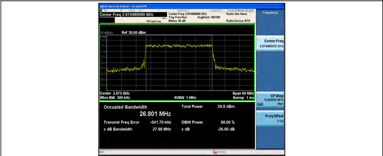
1-N41-PC2-30-30-H-3-DFT-16QAM-Outer_Full-75@0-ANT41-26.801-27.98-≤30-PASS
