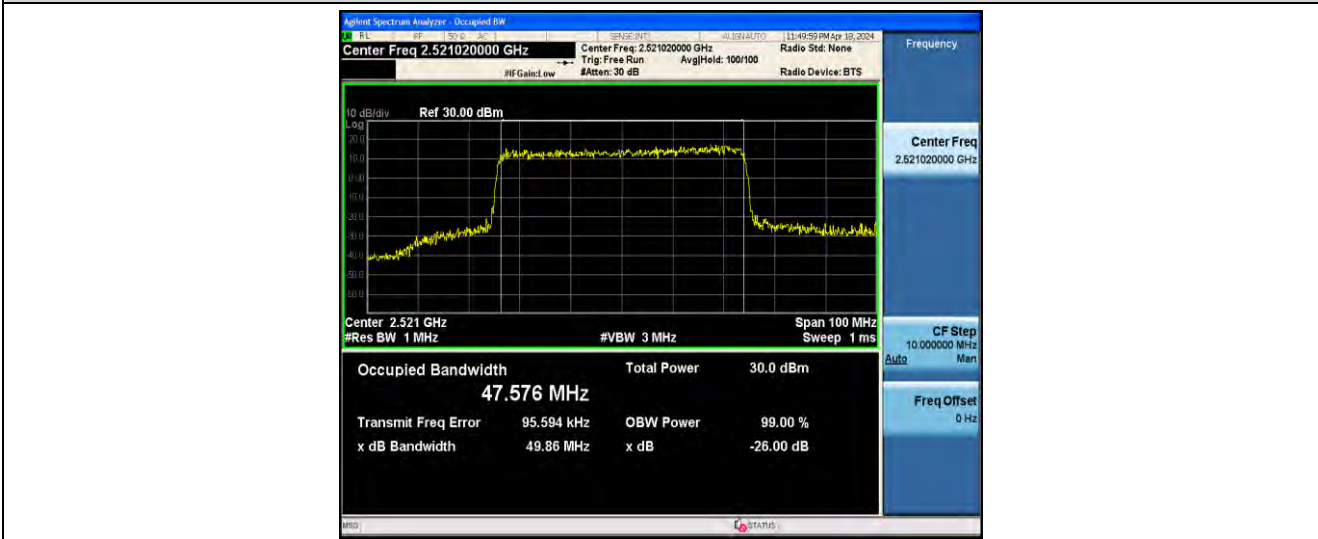
1-N41-PC2-30-50-L-7-CP-16QAM-Outer_Full-133@0-ANT41-47.576-49.86-≤50-PASS
