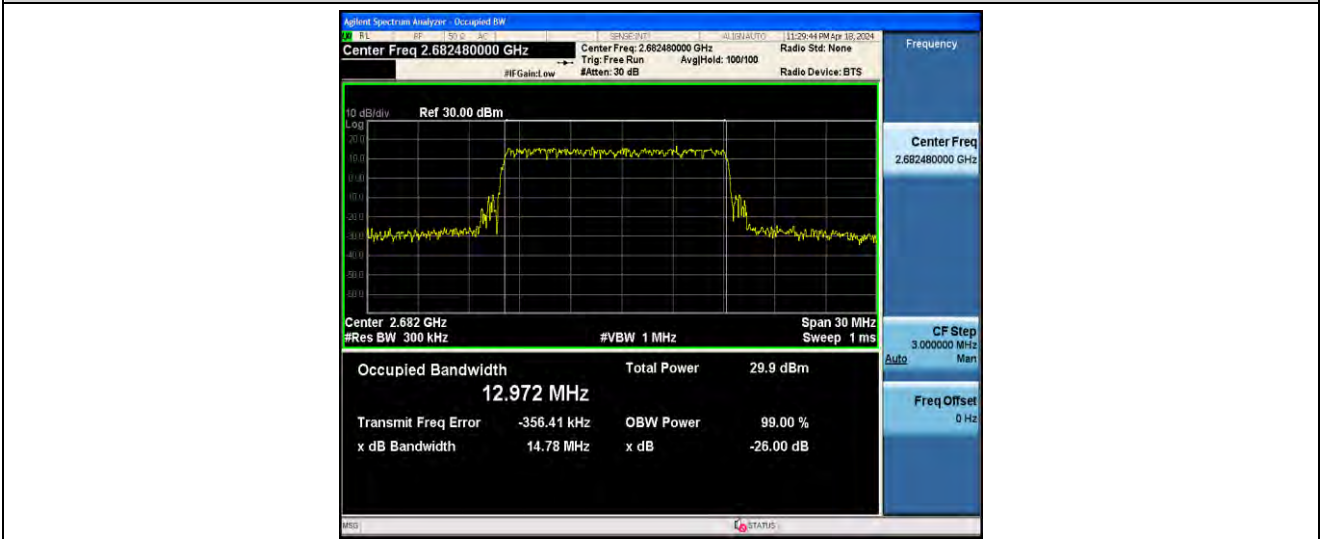
1-N41-PC2-30-15-H-3-DFT-16QAM-Outer_Full-36@0-ANT41-12.972-14.78-<=15-PASS
