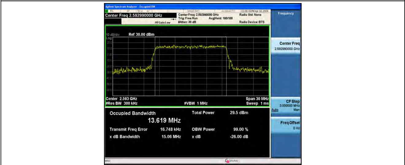
1-N41-PC2-30-15-M-6-CP-QPSK-Outer_Full-38@0-ANT41-13.619-15.06-≤15-PASS
