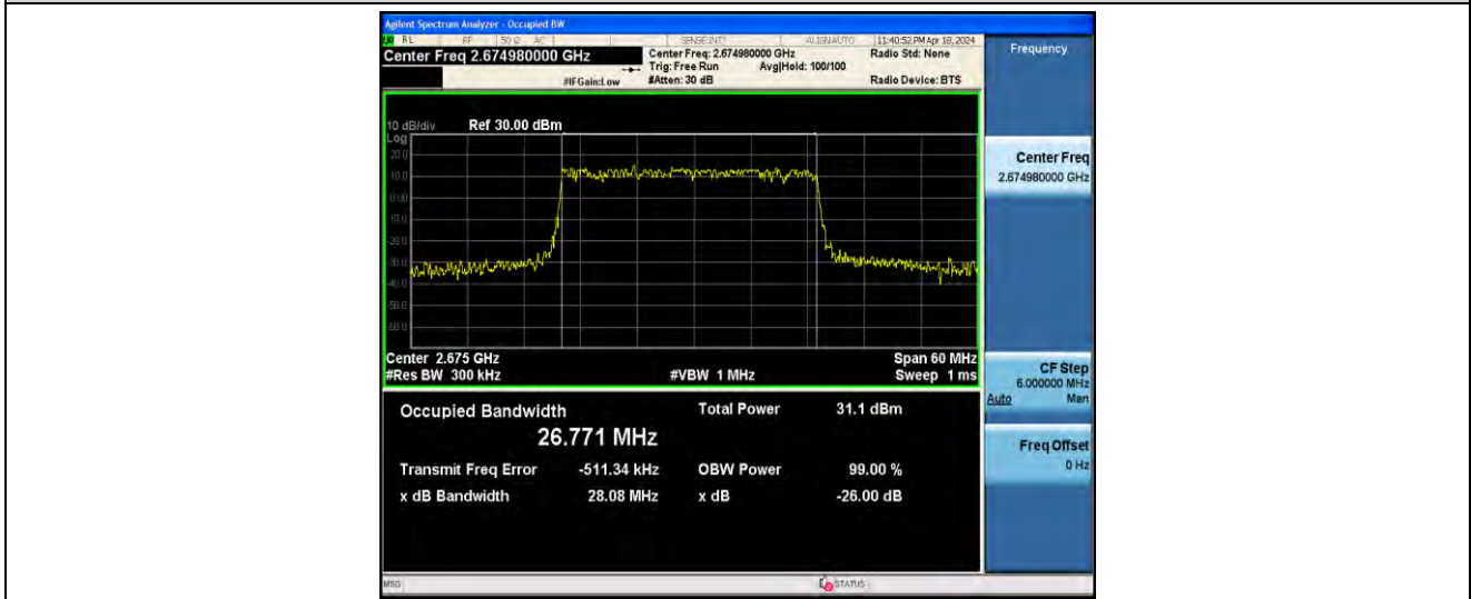
1-N41-PC2-30-30-H-1-DFT-QPSK-Outer_Full-75@0-ANT41-26.771-28.08-≤30-PASS
