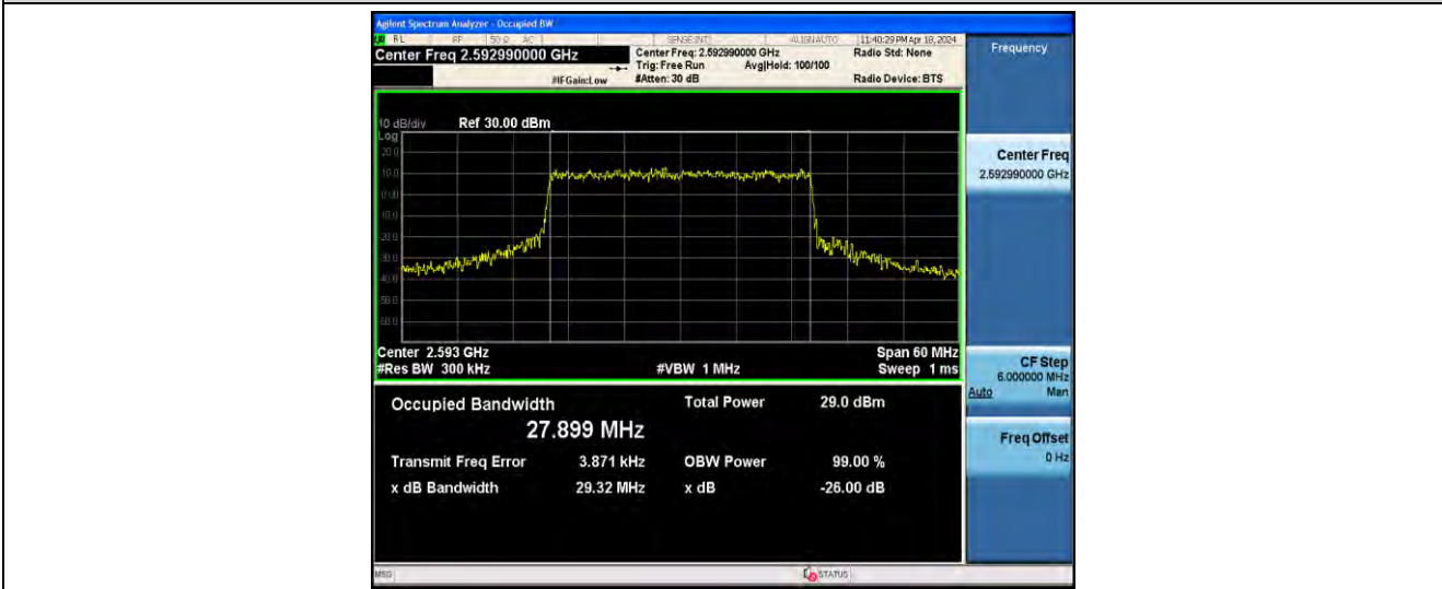
1-N41-PC2-30-30-M-8-CP-64QAM-Outer_Full-78@0-ANT41-27.899-29.32-<30-PASS
