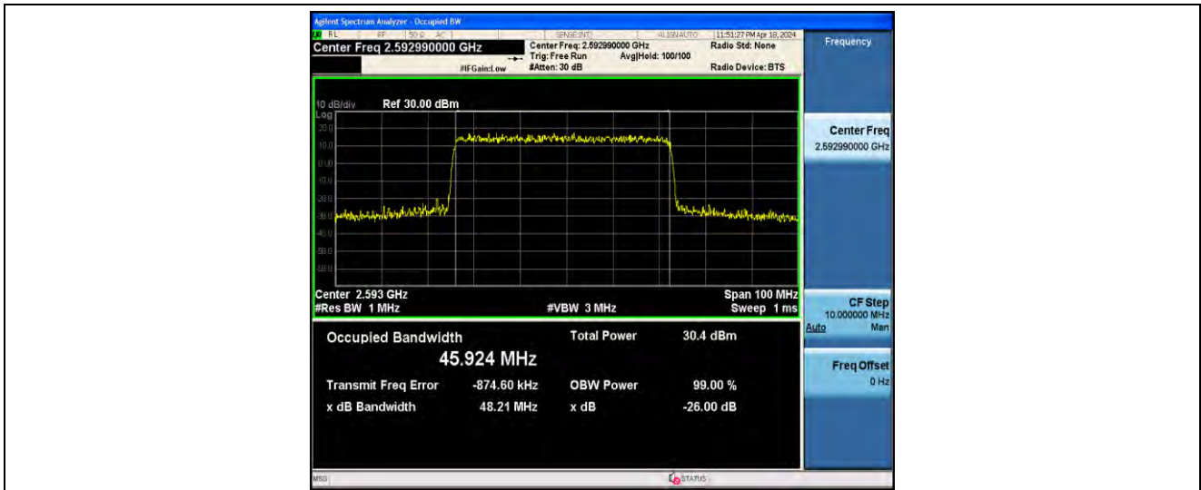
1-N41-PC2-30-50-M-3-DFT-16QAM-Outer_Full-128@0-ANT41-45.924-48.21-<=50-PASS
