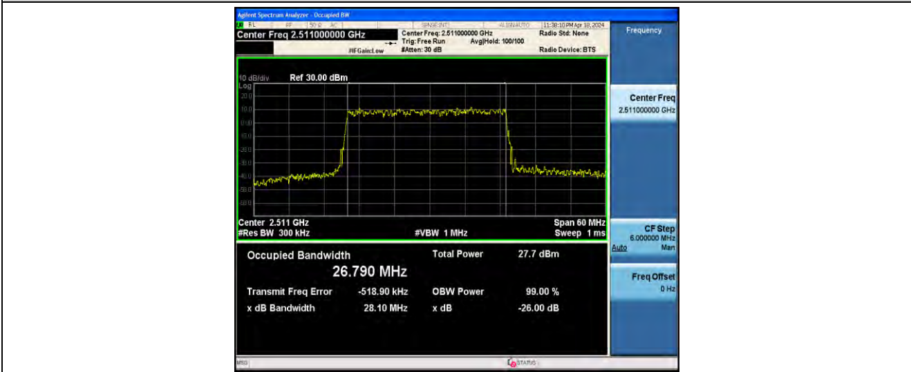
1-N41-PC2-30-30-L-5-DFT-256QAM-Outer_Full-75@0-ANT41-26.790-28.10-<=30-PASS
