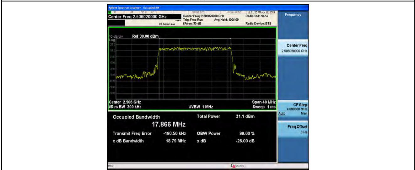
1-N41-PC2-30-20-L-2-DFT-PI2BPSK-Outer_Full-50@0-ANT41-17.866-18.79-<20-PASS
