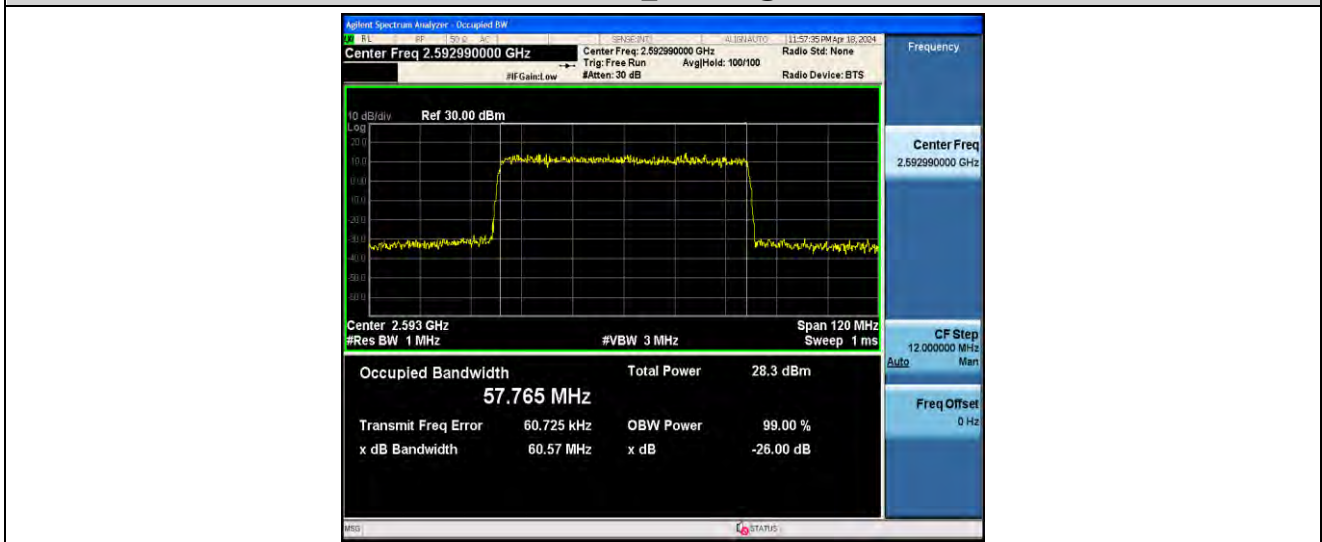
1-N41-PC2-30-60-M-5-DFT-256QAM-Outer_Full-162@0-ANT41-57.765-60.57-≤60-PASS
