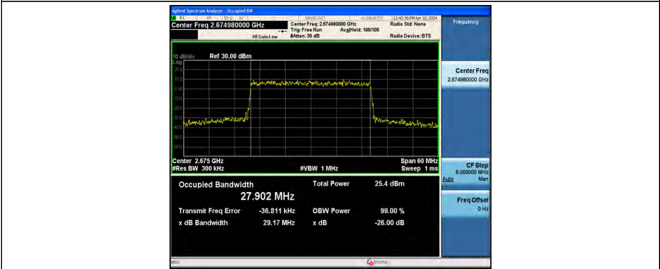
1-N41-PC2-30-30-H-9-CP-256QAM-Outer_Full-78@0-ANT41-27.902-29.17-≤30-PASS
