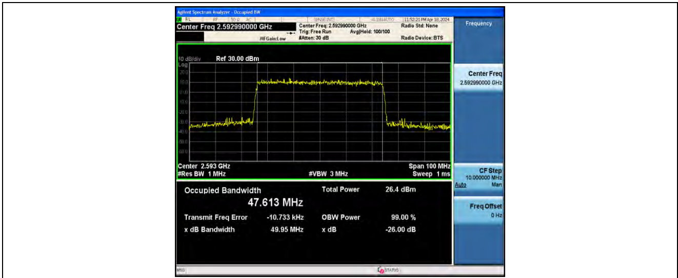
1-N41-PC2-30-50-M-9-CP-256QAM-Outer_Full-133@0-ANT41-47.613-49.95-<math>\leq 50</math>-PASS
