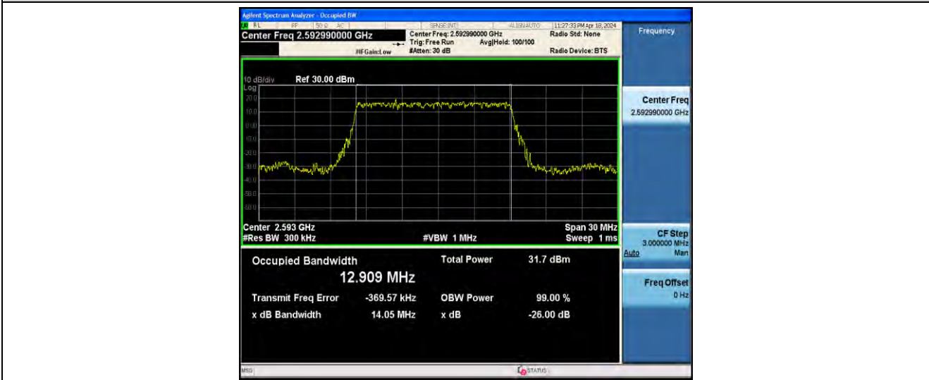
1-N41-PC2-30-15-M-2-DFT-PI2BPSK-Outer_Full-36@0-ANT41-12.909-14.05-≤15-PASS
