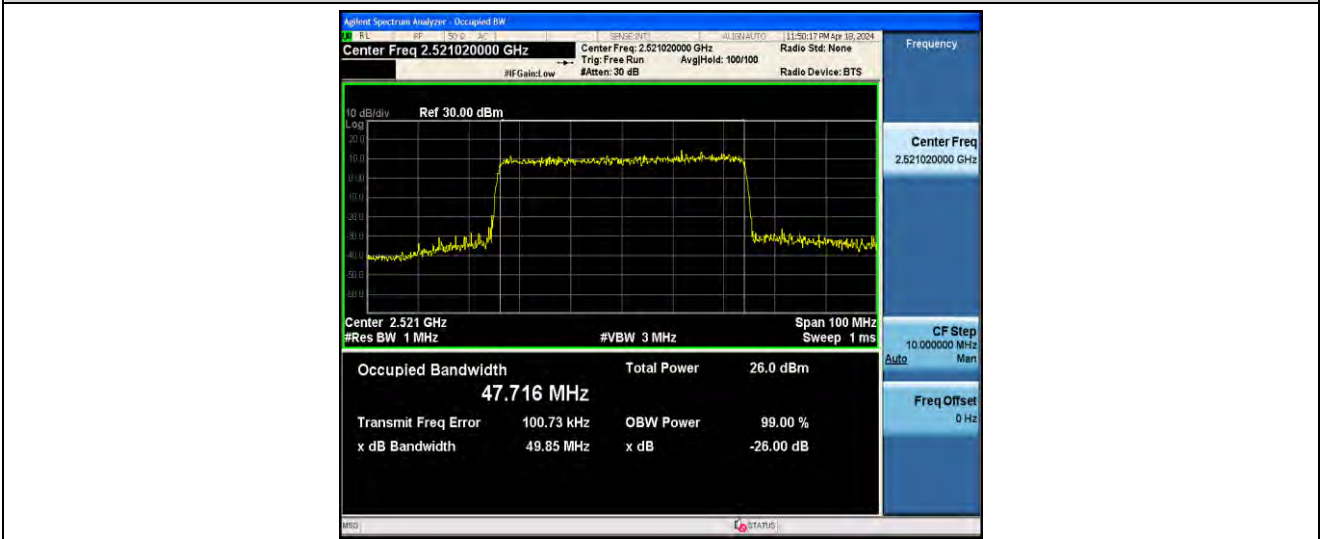
1-N41-PC2-30-50-L-9-CP-256QAM-Outer_Full-133@0-ANT41-47.716-49.85-<=50-PASS
