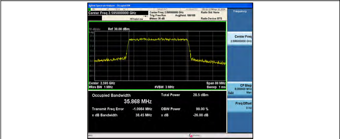
1-N38-PC3-30-40-M-3-DFT-16QAM-Outer_Full-100@0-ANT41-35.868-38.45-≤40-PASS
