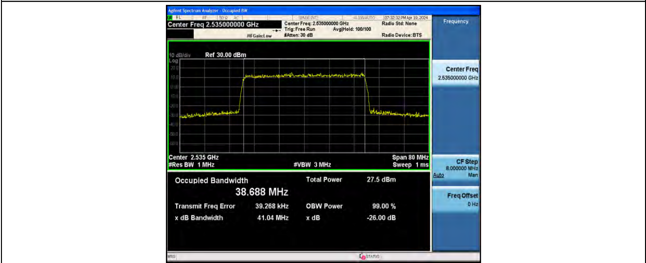
1-N7-PC3-15-40-M-5-DFT-256QAM-Outer_Full-216@0-ANT41-38.688-41.04-≤40-PASS
