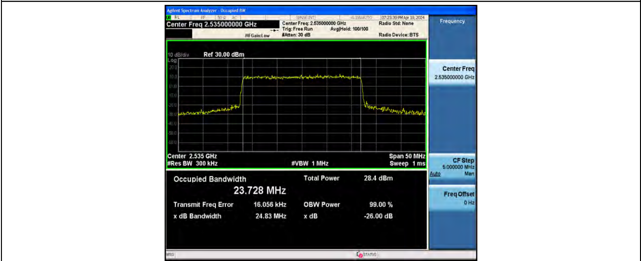
1-N7-PC3-15-25-M-7-CP-16QAM-Outer_Full-133@0-ANT41-23.728-24.83-≤25-PASS
