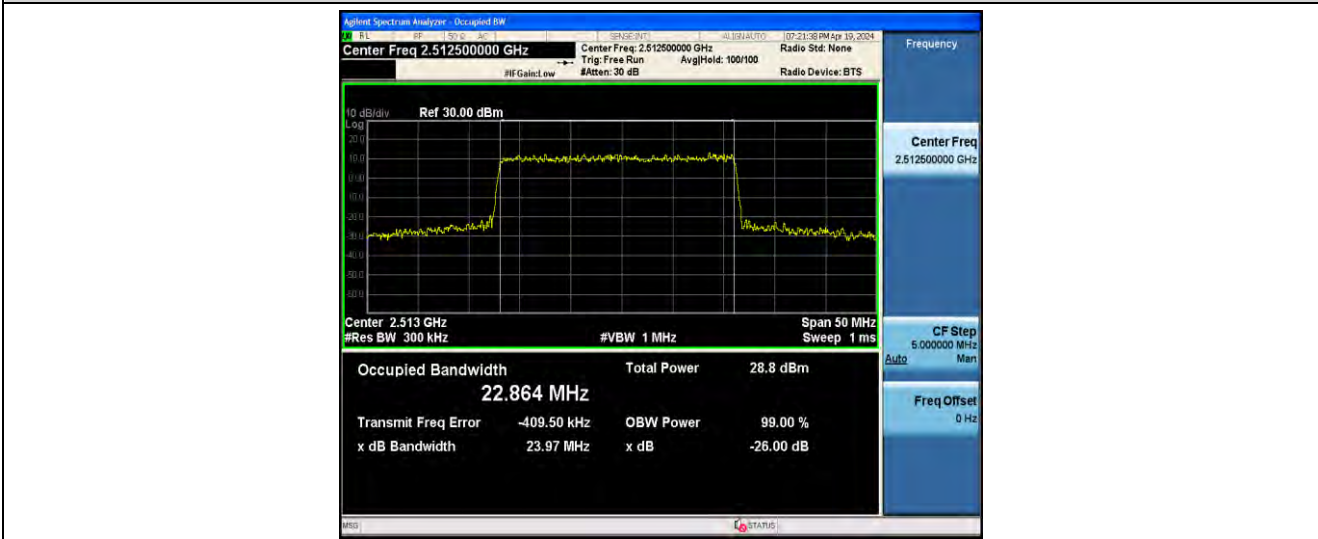
1-N7-PC3-15-25-L-4-DFT-64QAM-Outer_Full-128@0-ANT41-22.864-23.97-≤25-PASS
