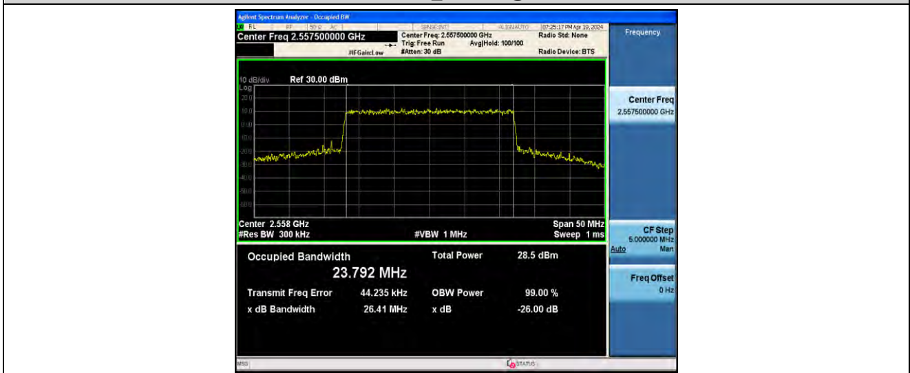
1-N7-PC3-15-25-H-8-CP-64QAM-Outer_Full-133@0-ANT41-23.792-26.41-<25-PASS
