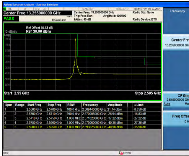
1-N7-PC3-15-20-H-2-DFT-PI2BPSK-Edge_1RB_Right-1@105-ANT41-2593.83-15.98--40.98-PASS
