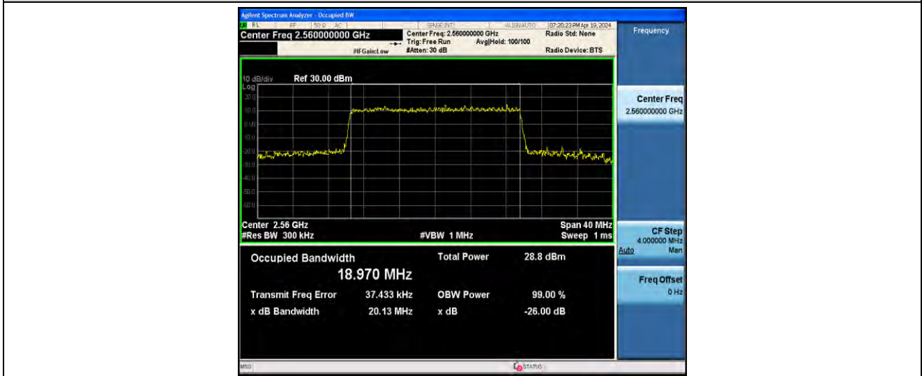
1-N7-PC3-15-20-H-7-CP-16QAM-Outer_Full-106@0-ANT41-18.970-20.13-≤20-PASS
