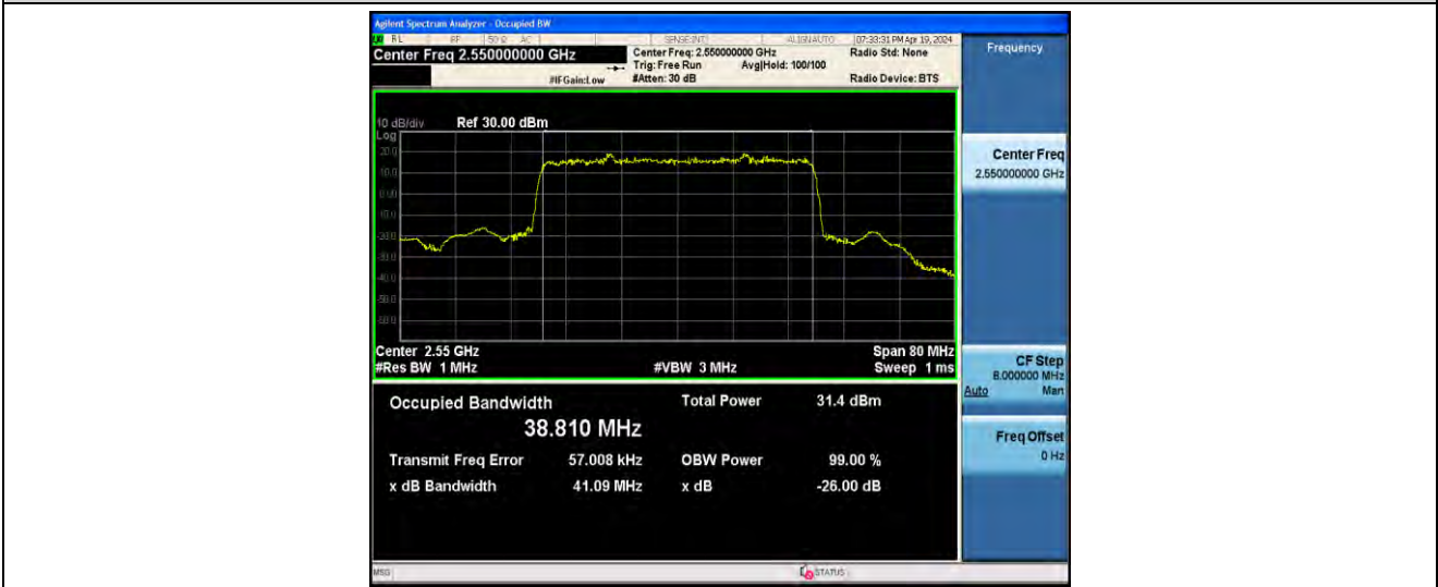
1-N7-PC3-15-40-H-2-DFT-PI2BPSK-Outer_Full-216@0-ANT41-38.810-41.09-<=40-PASS
