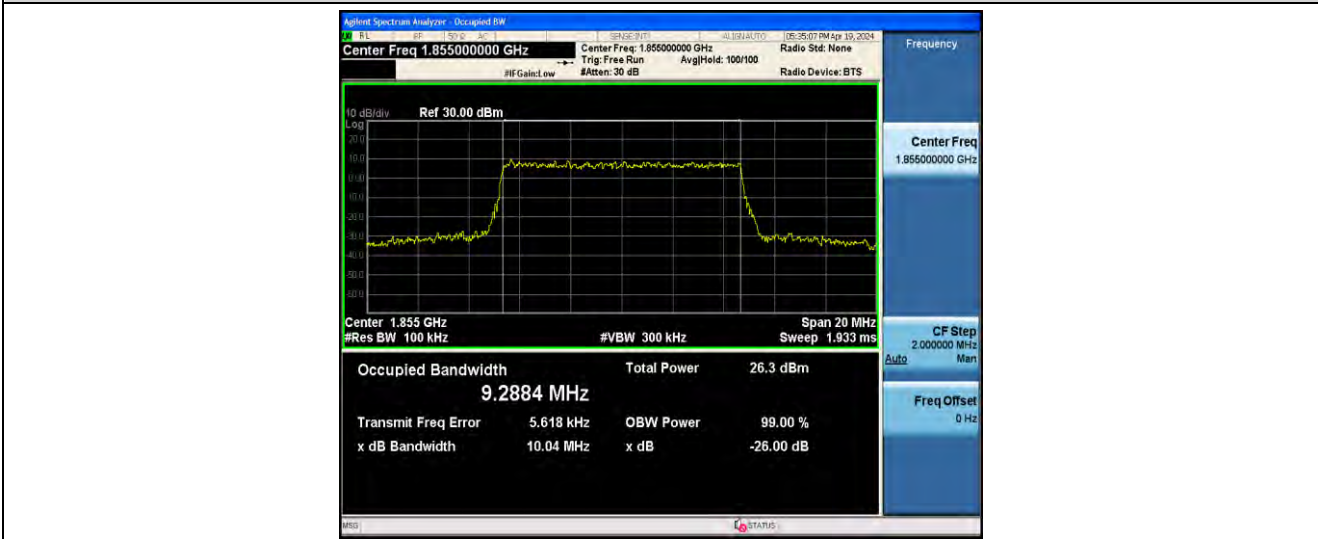
1-N2-PC3-15-10-L-9-CP-256QAM-Outer_Full-52@0-ANT41-9.2884-10.04-≤10-PASS
