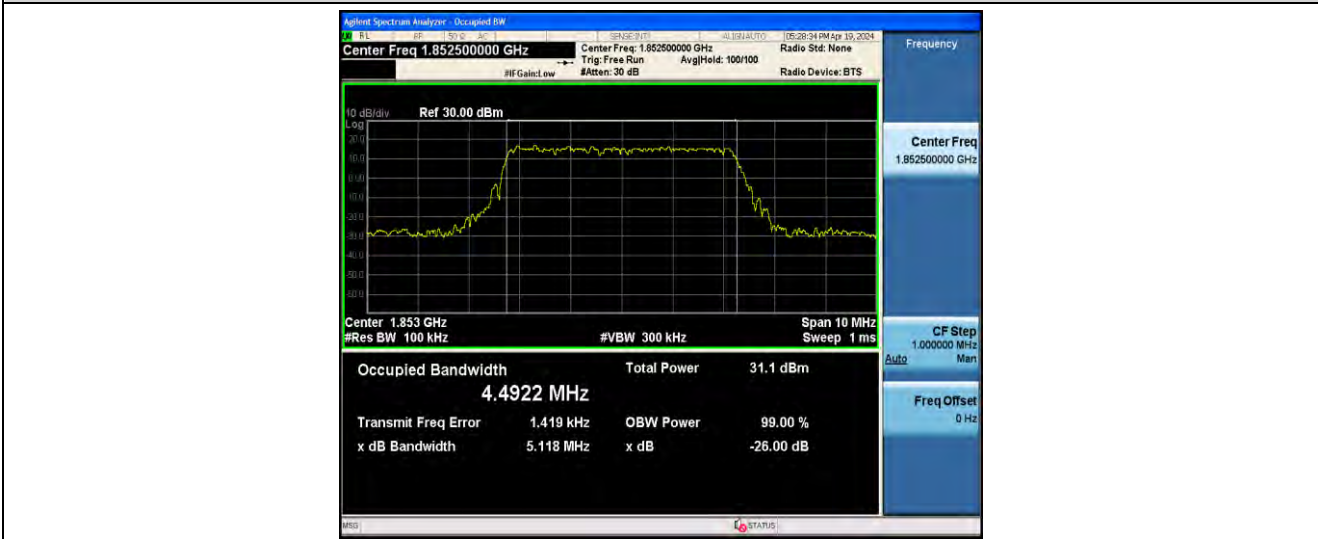
1-N2-PC3-15-5-L-4-DFT-64QAM-Outer_Full-25@0-ANT41-4.4922-5.118-≤5-PASS
