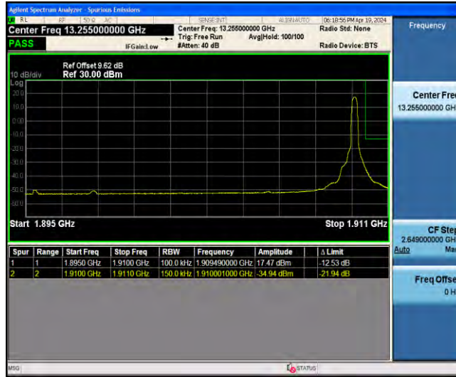
1-N2-PC3-15-15-H-5-CP-QPSK-Edge_1RB_Right-1@78-ANT41-1910.00-21.94--34.94-PASS
