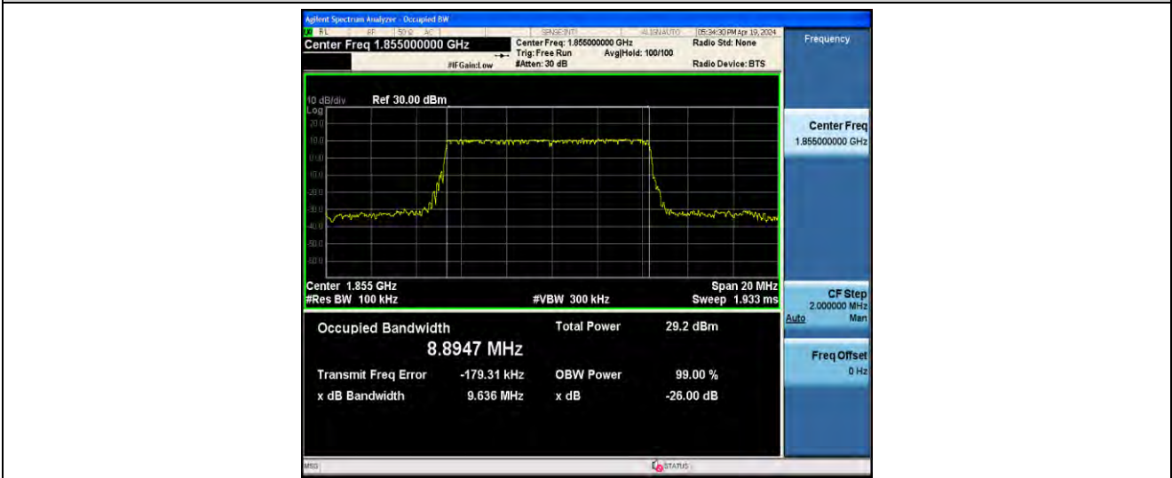
1-N2-PC3-15-10-L-5-DFT-256QAM-Outer_Full-50@0-ANT41-8.8947-9.636-≤10-PASS
