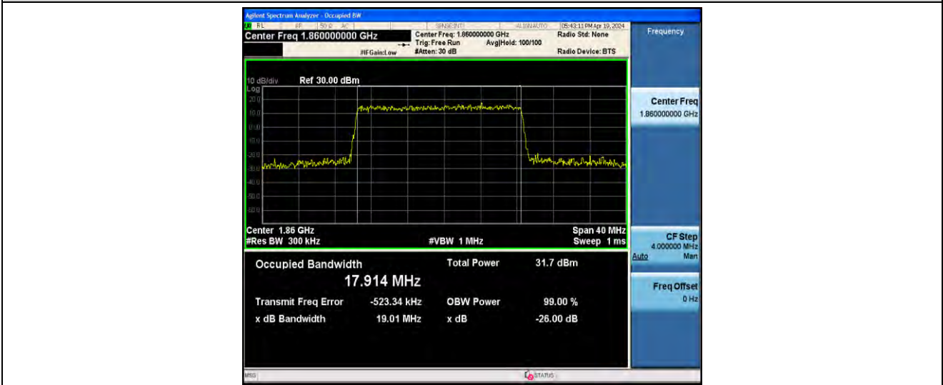
1-N2-PC3-15-20-L-1-DFT-QPSK-Outer_Full-100@0-ANT41-17.914-19.01-≤20-PASS
