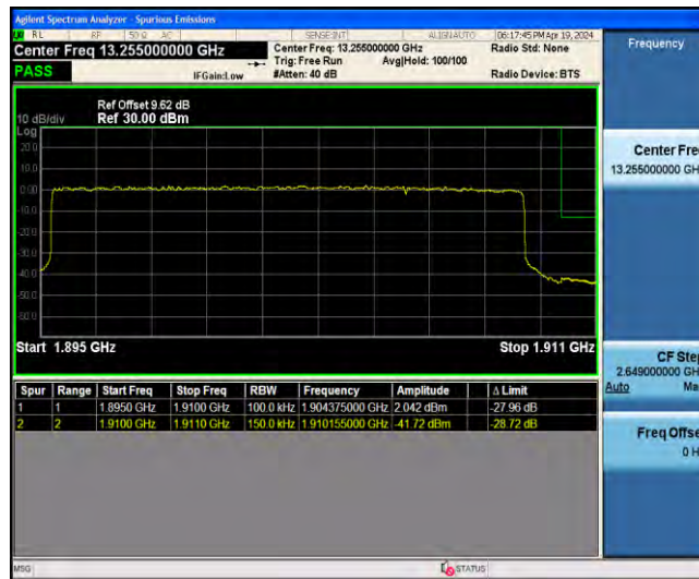
1-N2-PC3-15-15-H-3-DFT-PI2BPSK-Outer_Full-75@0-ANT41-1910.16-28.72--41.72-PASS
