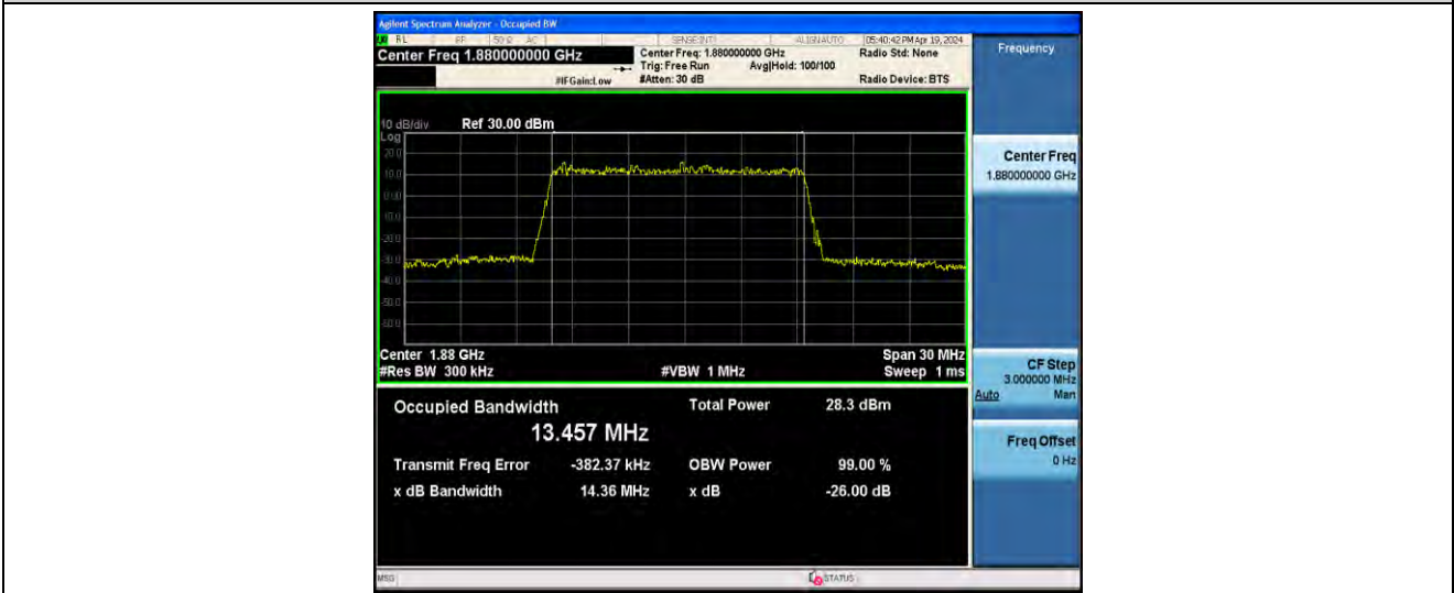
1-N2-PC3-15-15-M-5-DFT-256QAM-Outer_Full-75@0-ANT41-13.457-14.36-≤15-PASS
