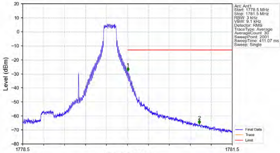
Band66_1.4MHz_64QAM_HCH_1779.3MHz_RB_1_5_NTNV
