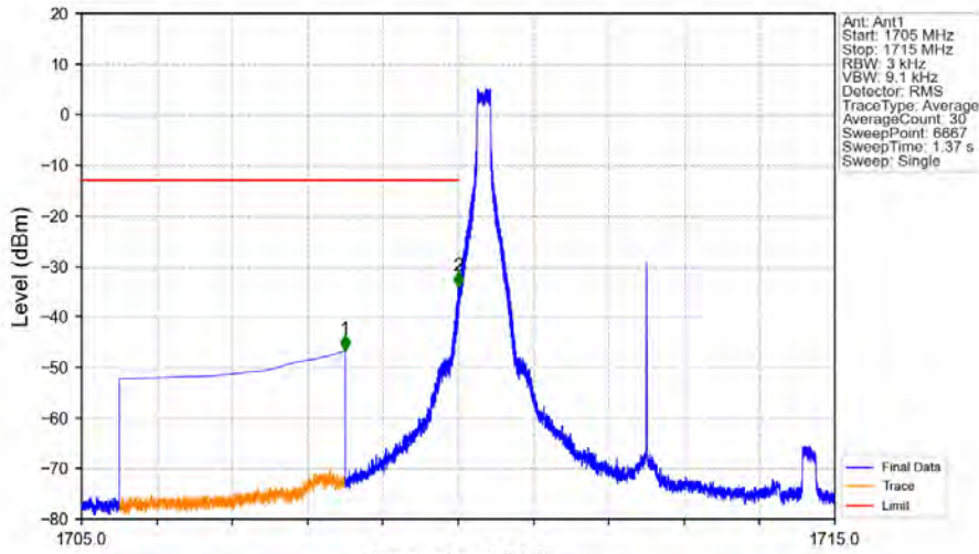
Band66_5MHz_64QAM_LCH_1712.5MHz_RB_1_0_NTV
