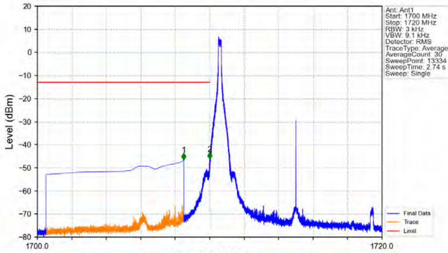
Band66_10MHz_16QAM_LCH_1715MHz_RB_1_0_NTNV
