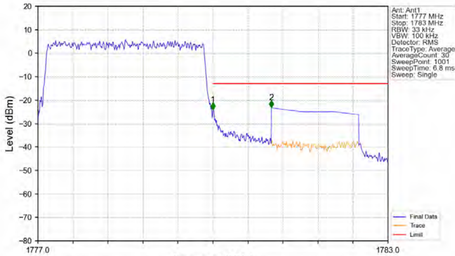
Band66_3MHz_QPSK_HCH_1778.5MHz_RB_15_0_NTNV
