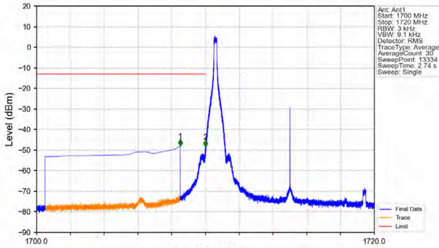
Band66_10MHz_64QAM_LCH_1715MHz_RB_1_0_NTNV
