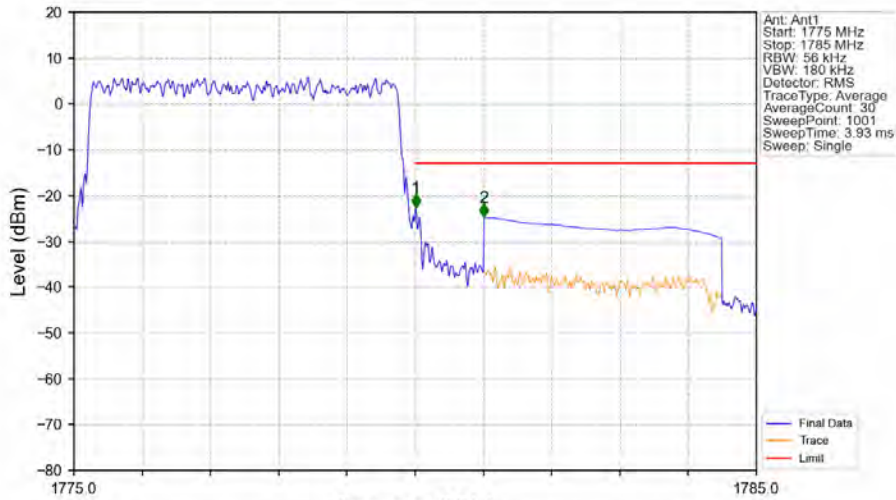
Band66_5MHz_QPSK_HCH_1777.5MHz_RB_25_0_NTNV
