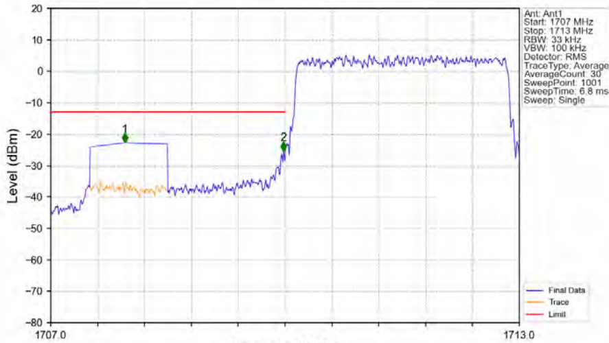
Band66_3MHz_QPSK_LCH_1711.5MHz_RB_15_0_NTNV
