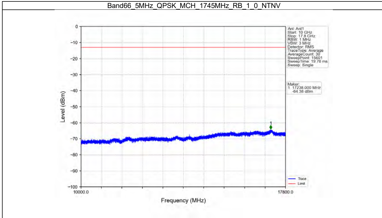
Band66_5MHz_QPSK_MCH_1745MHz_RB_1_0_NTNV
