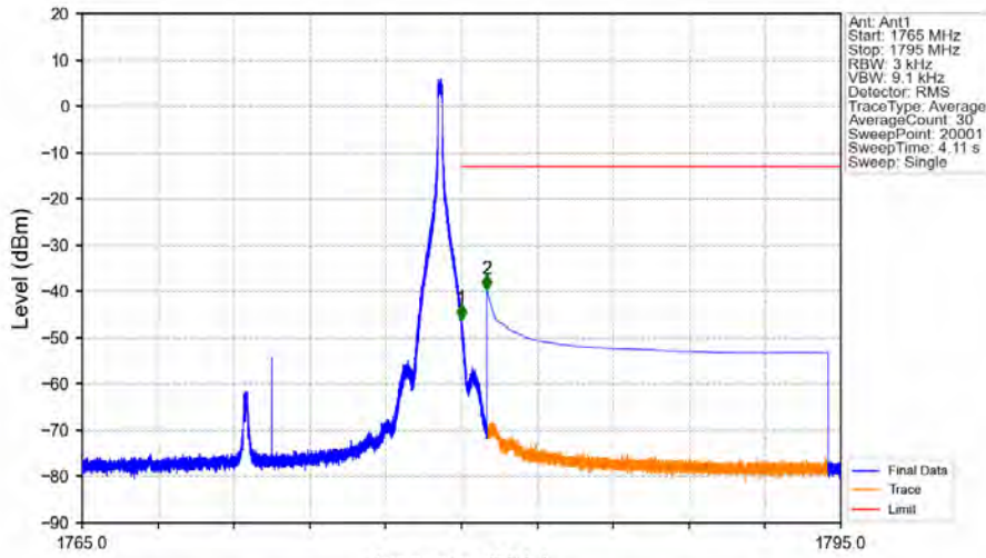
Band66_15MHz_64QAM_HCH_1772.5MHz_RB_1_74_NTNV
