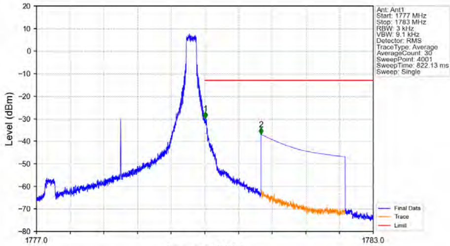
Band66_3MHz_QPSK_HCH_1778.5MHz_RB_1_14_NTNV
