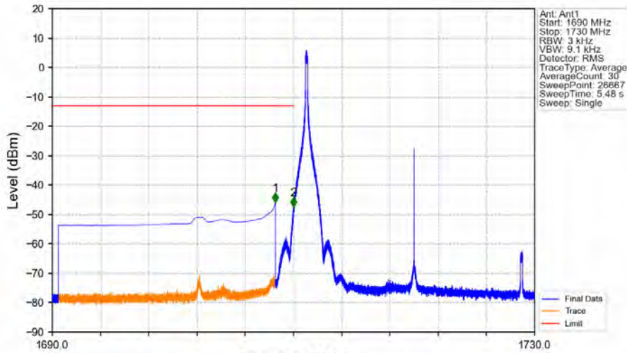
Band66_20MHz_64QAM_LCH_1720MHz_RB_1_0_NTNV
