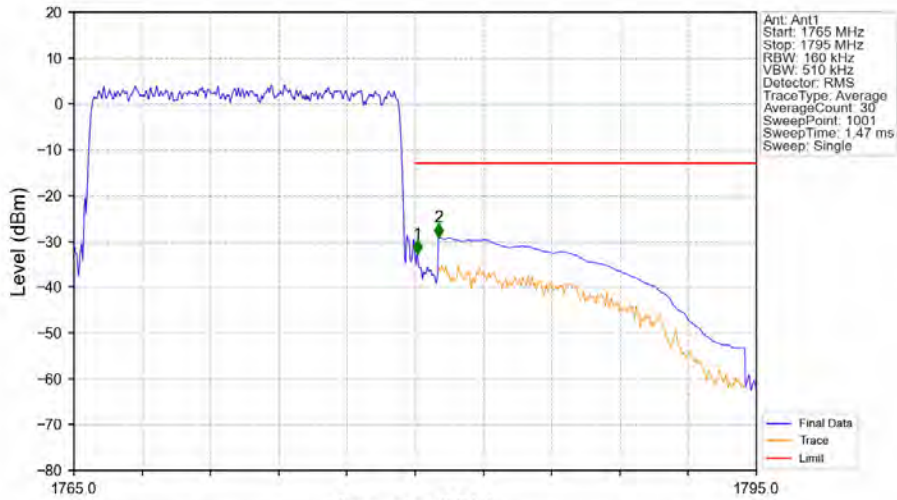
Band66_15MHz_16QAM_HCH_1772.5MHz_RB_75_0_NTNV
