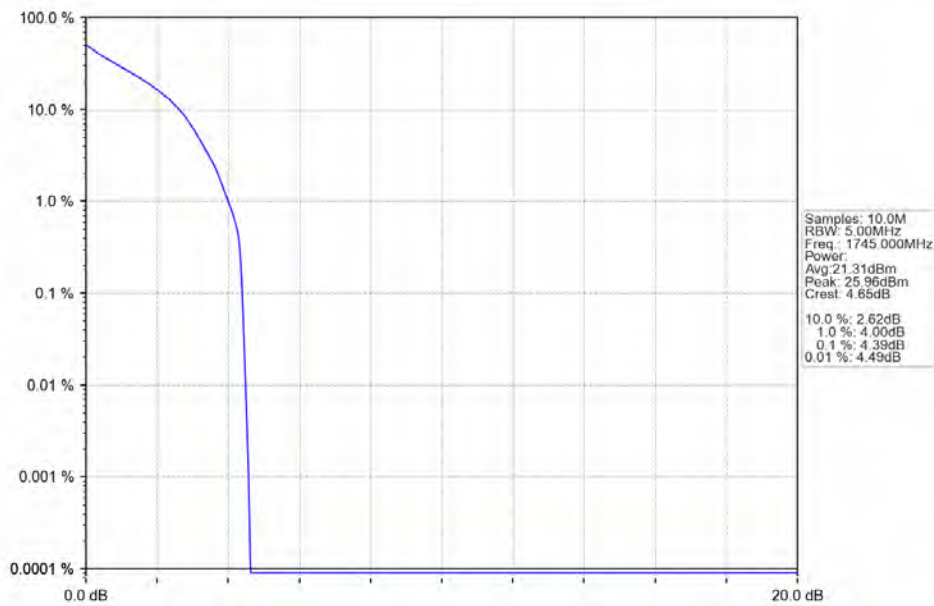
Band66_1.4MHz_QPSK_MCH_1745MHz_RB_6_0_NTNV
