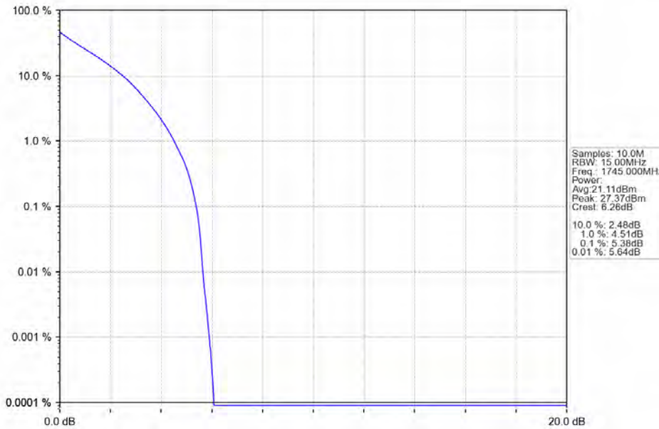
Band66_15MHz_QPSK_MCH_1745MHz_RB_75_0_NTNV
