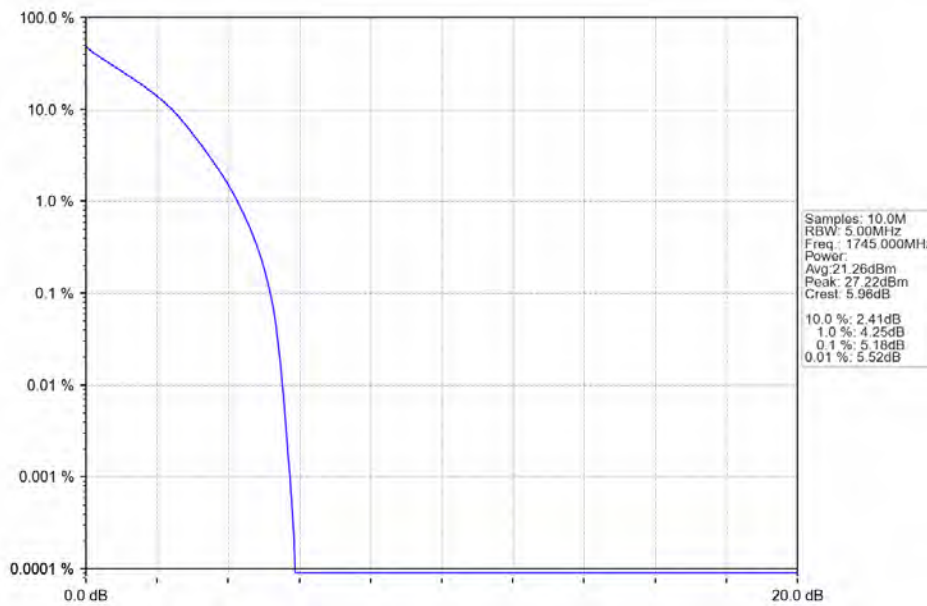
Band66_5MHz_QPSK_MCH_1745MHz_RB_25_0_NTNV
