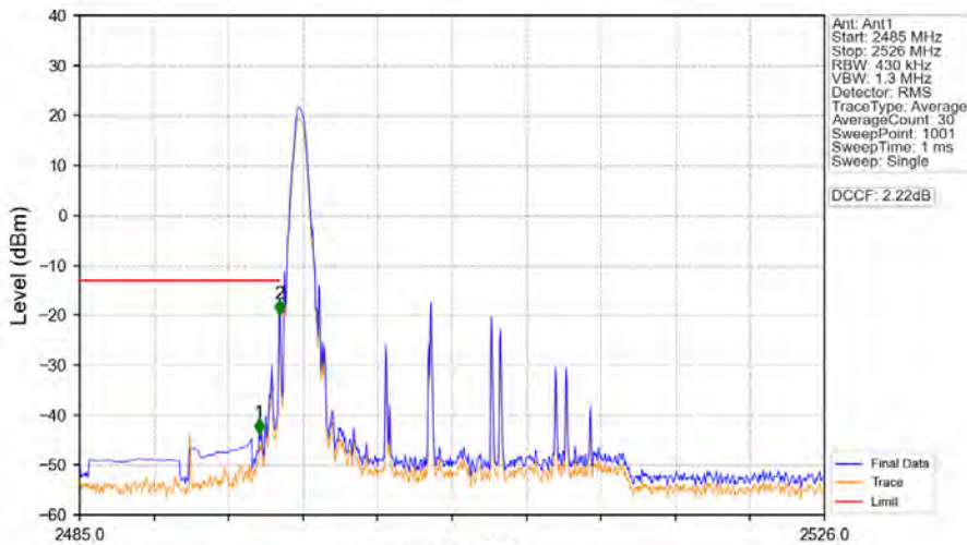
Band41_20MHz_16QAM_LCH_2506MHz_RB_1_0_NTNV
