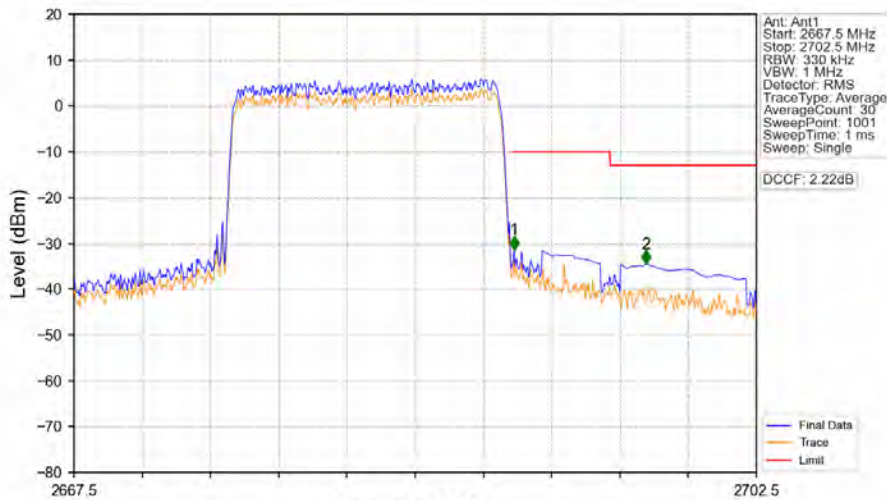
Band41_15MHz_64QAM_HCH_2682.5MHz_RB_75_0_NTNV
