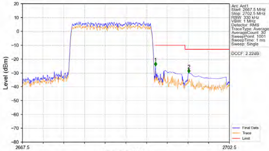
Band41_15MHz_16QAM_HCH_2682.5MHz_RB_75_0_NTNV
