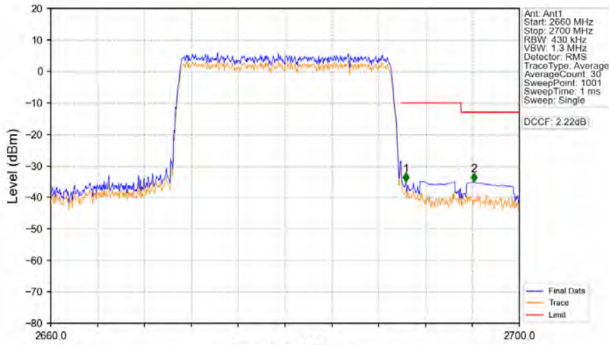
Band41_20MHz_64QAM_HCH_2680MHz_RB_100_0_NTNV
