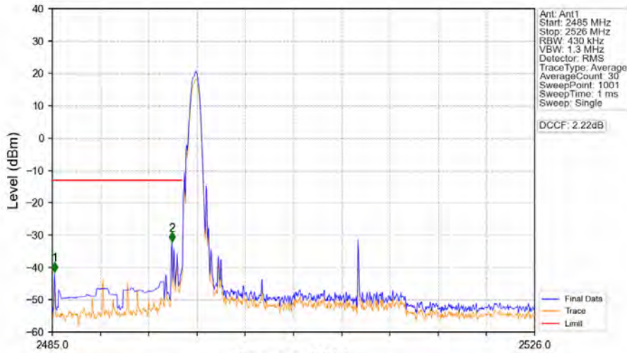
Band41_20MHz_64QAM_LCH_2506MHz_RB_1_0_NTNV
