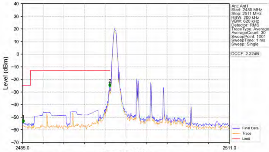
Band41_10MHz_64QAM_LCH_2501MHz_RB_1_0_NTNV
