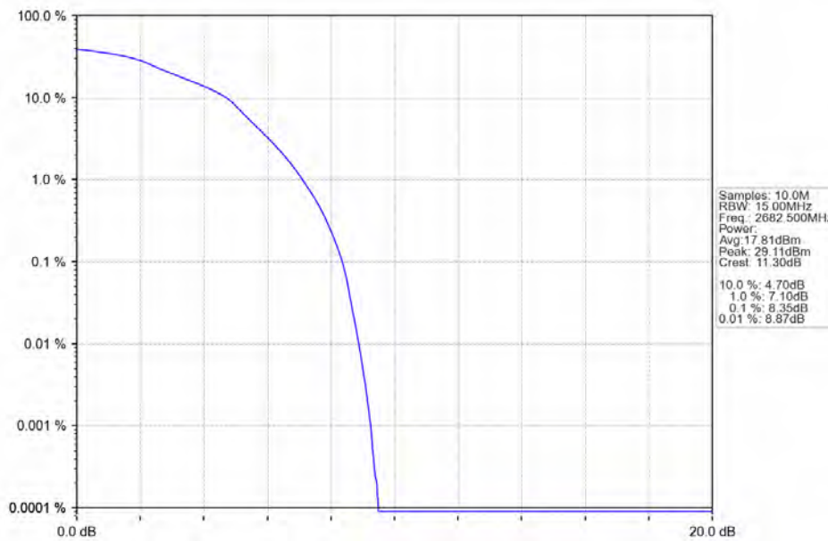
Band41_15MHz_16QAM_HCH_2682.5MHz_RB_75_0_NTNV
