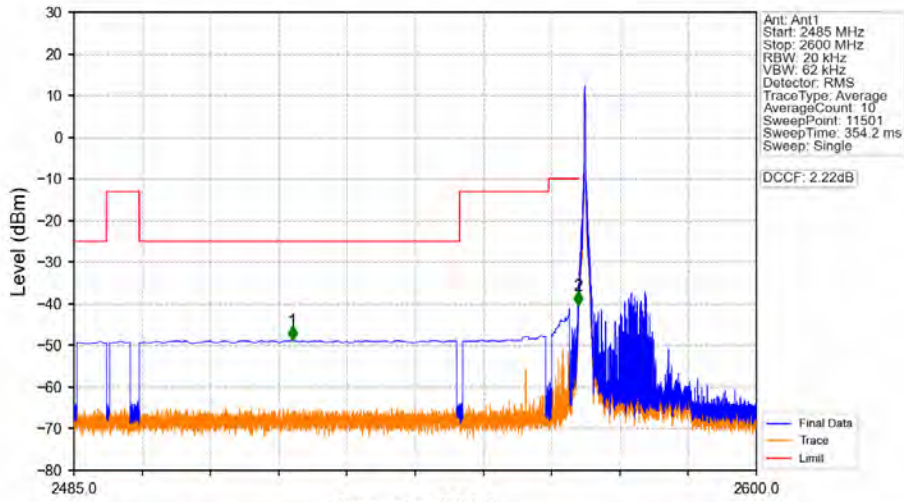
Band38_20MHz_64QAM_LCH_2580MHz_RB_1_0_NTNV
