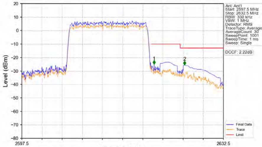
Band38_15MHz_16QAM_HCH_2612.5MHz_RB_75_0_NTNV
