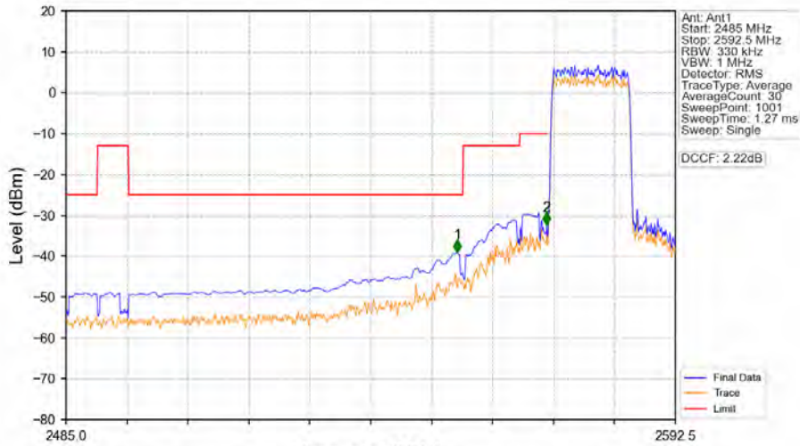
Band38_15MHz_16QAM_LCH_2577.5MHz_RB_75_0_NTNV
