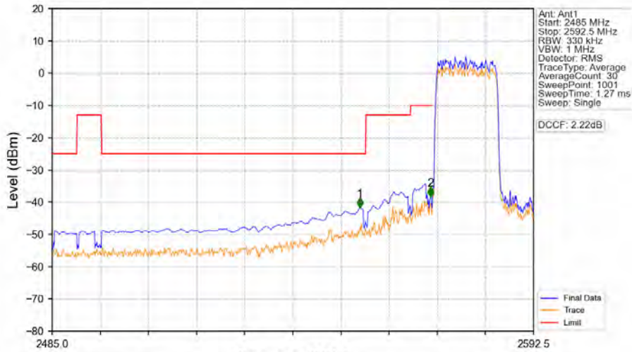
Band38_15MHz_64QAM_LCH_2577.5MHz_RB_75_0_NTNV
