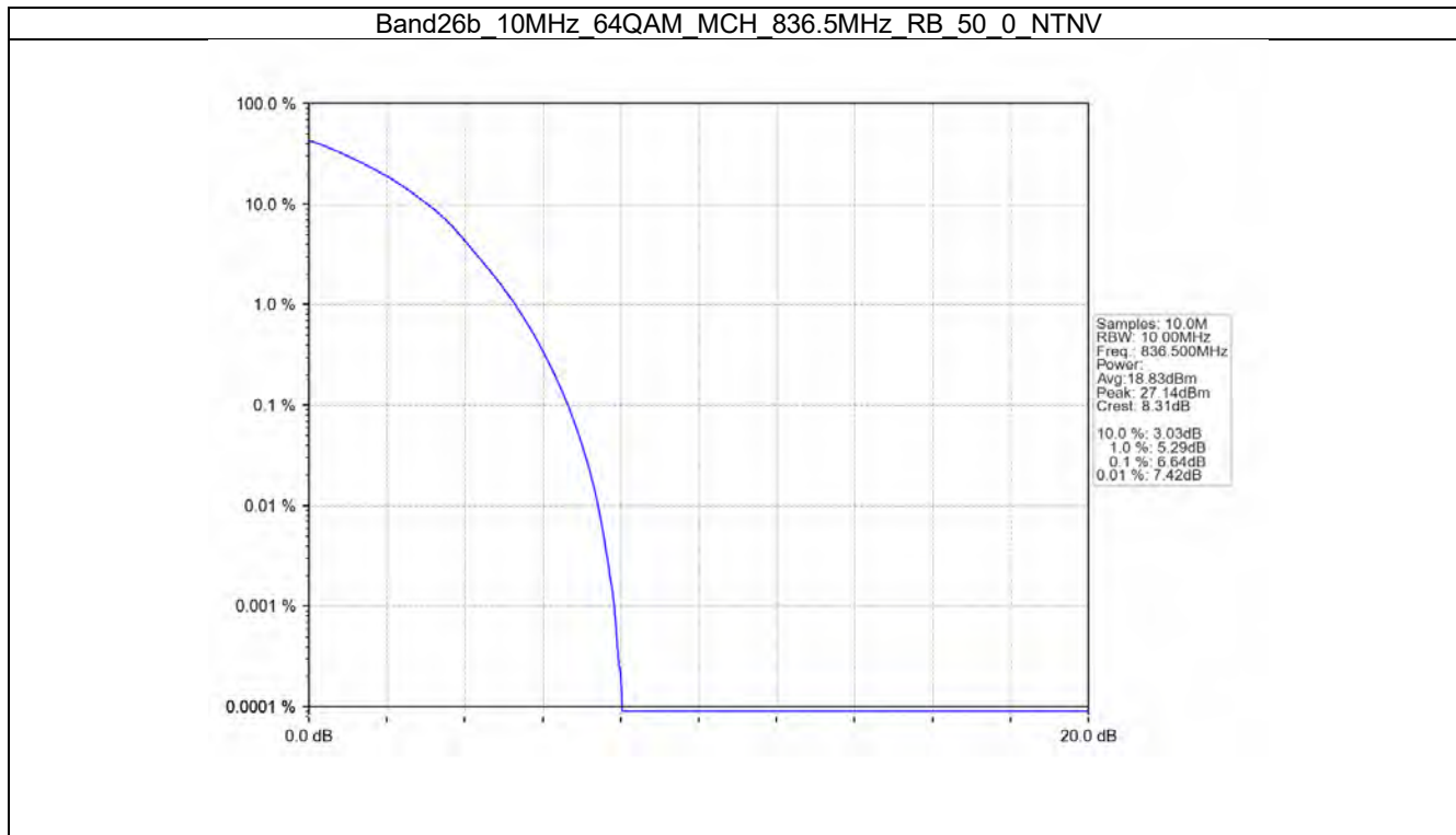
Band26b_10MHz_64QAM_MCH_836.5MHz_RB_50_0_NTNV
