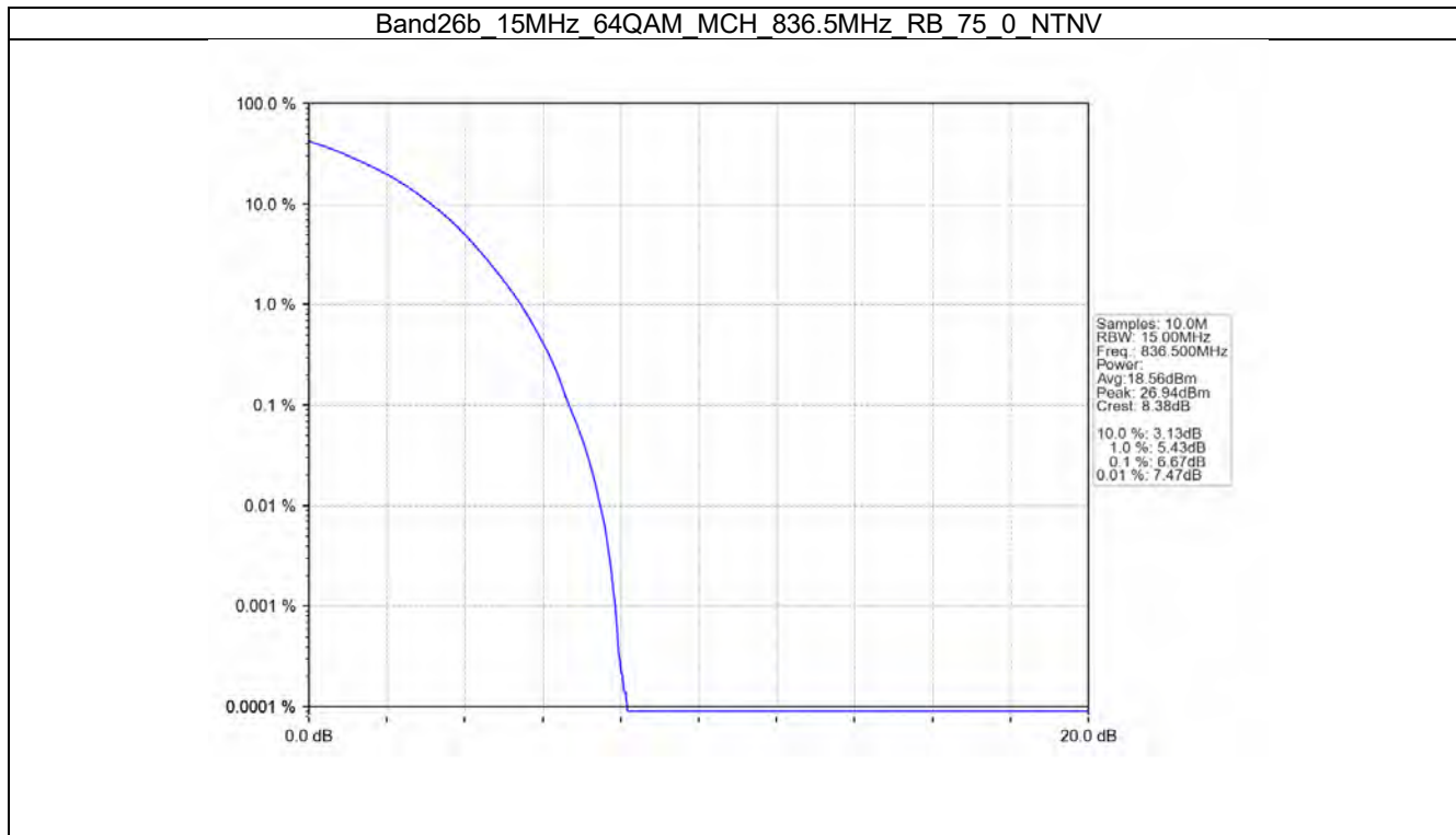
Band26b_15MHz_64QAM_MCH_836.5MHz_RB_75_0_NTNV
