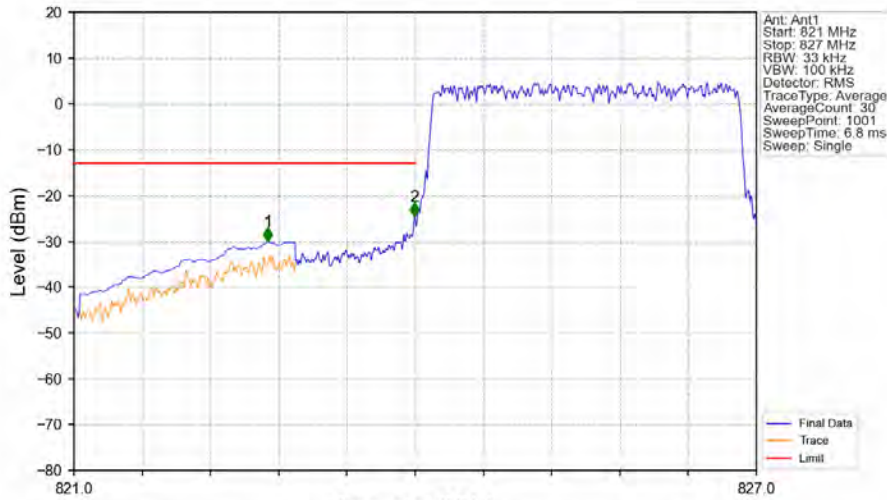
Band26b_3MHz_QPSK_LCH_825.5MHz_RB_15_0_NTNV
