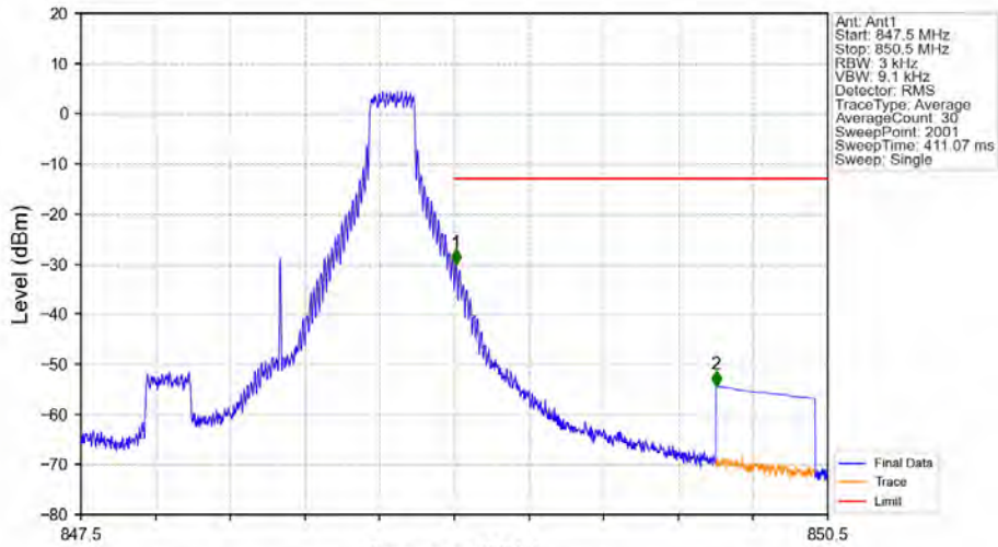
Band26b_1.4MHz_64QAM_HCH_848.3MHz_RB_1_5_NTNV
