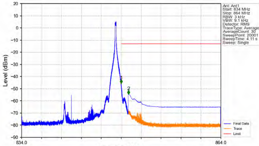
Band26b_15MHz_16QAM_HCH_841.5MHz_RB_1_74_NTNV
