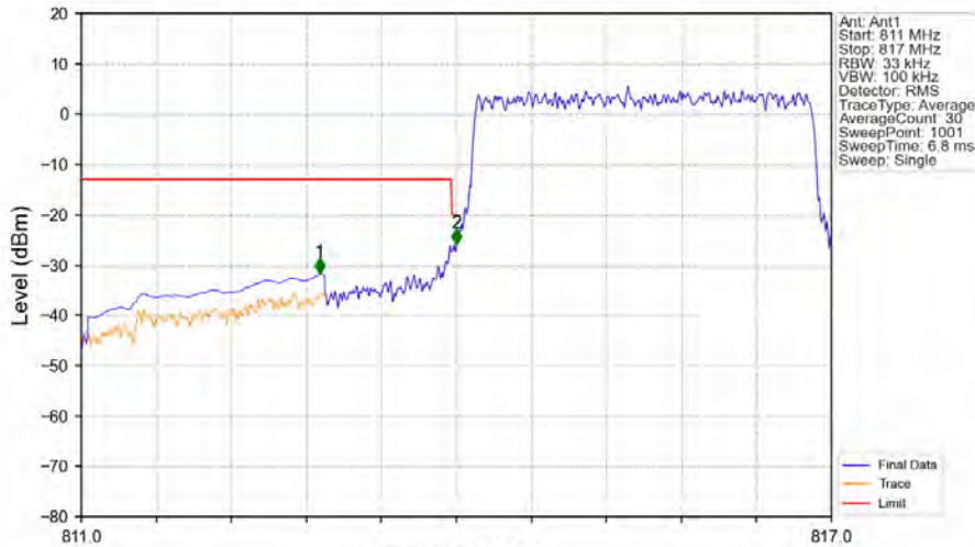
Band26a_3MHz_QPSK_LCH_815.5MHz_RB_15_0_NTNV
