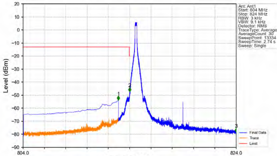
Band26a_10MHz_16QAM_LCH_819MHz_RB_1_0_NTNV
