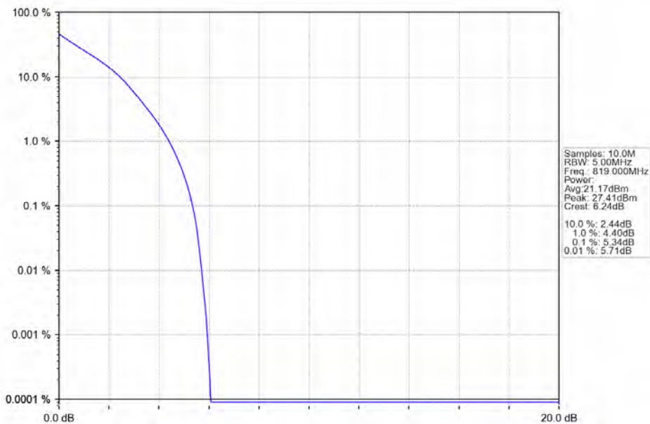
Band26a_5MHz_QPSK_MCH_819MHz_RB_25_0_NTV
