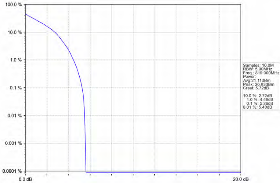
Band26a_1.4MHz_QPSK_MCH_819MHz_RB_6_0_NTNV
