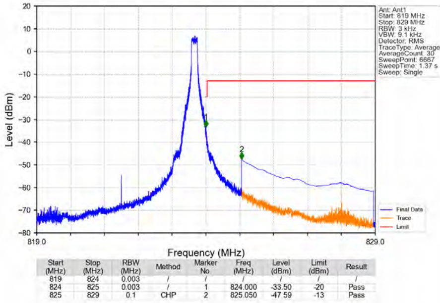
Band26a_5MHz_QPSK_HCH_821.5MHz_RB_1_24_NTNV
