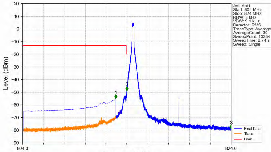
Band26a_10MHz_64QAM_LCH_819MHz_RB_1_0_NTNV
