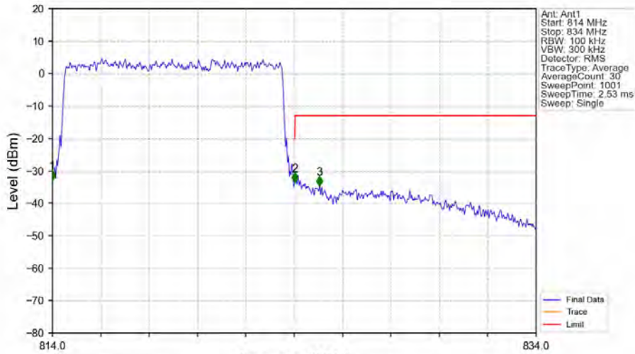
Band26a_10MHz_QPSK_HCH_819MHz_RB_50_0_NTNV
