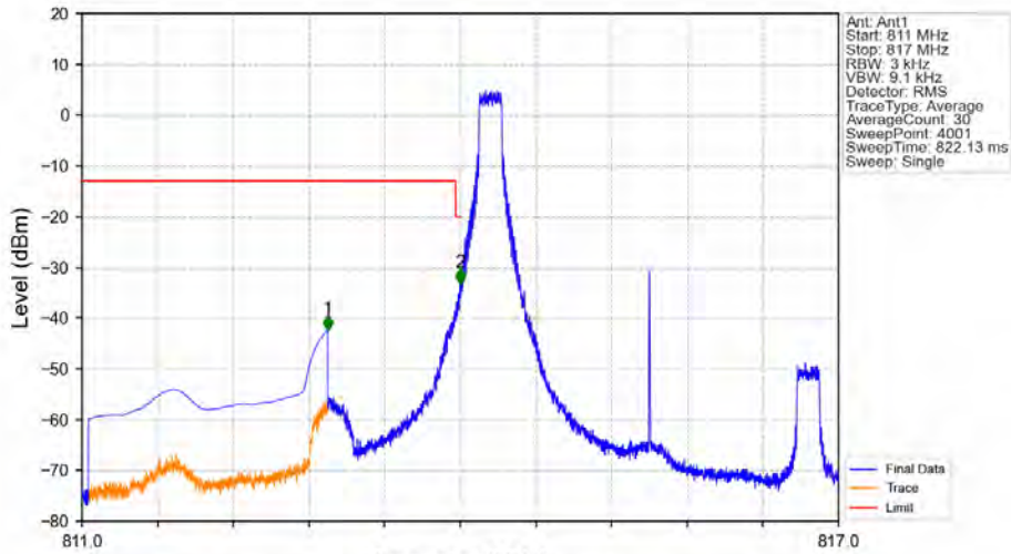
Band26a_3MHz_64QAM_LCH_815.5MHz_RB_1_0_NTNV
