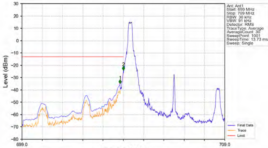
Band17_5MHz_16QAM_LCH_706.5MHz_RB_1_0_NTNV
