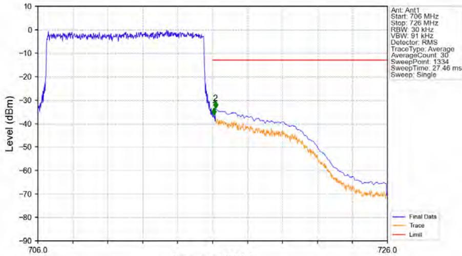
Band17_10MHz_QPSK_HCH_711MHz_RB_50_0_NTV
