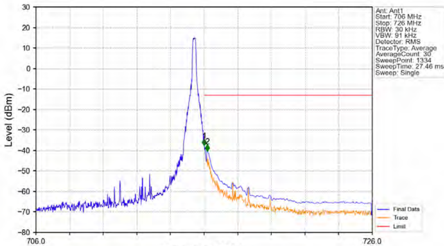
Band17_10MHz_16QAM_HCH_711MHz_RB_1_49_NTNV
