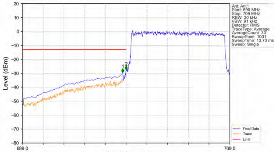
Band17_5MHz_64QAM_LCH_706.5MHz_RB_25_0_NTNV
