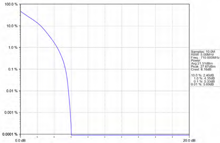
Band17_5MHz_QPSK_MCH_710MHz_RB_25_0_NTNV
