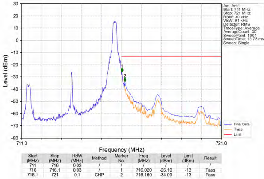
Band17_5MHz_16QAM_HCH_713.5MHz_RB_1_24_NTNV
