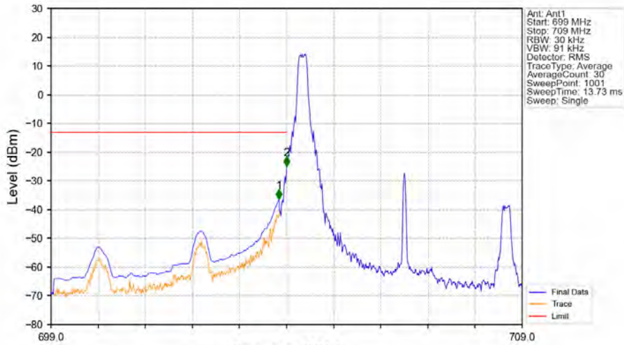
Band17_5MHz_64QAM_LCH_706.5MHz_RB_1_0_NTNV
