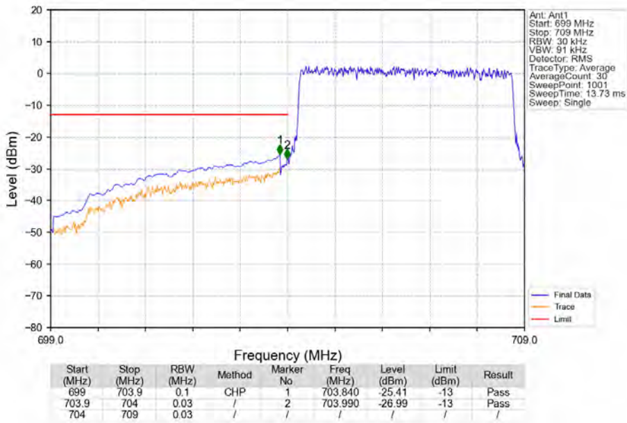
Band17_5MHz_QPSK_LCH_706.5MHz_RB_25_0_NTV
