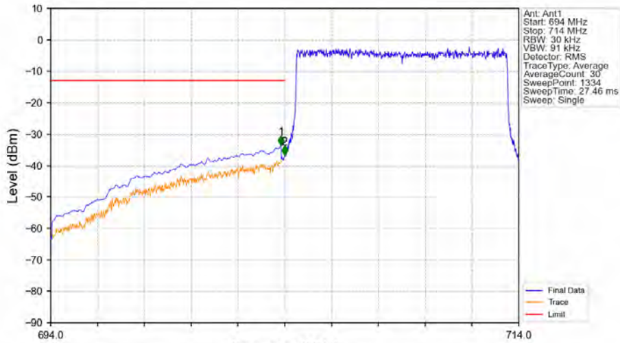
Band17_10MHz_64QAM_LCH_709MHz_RB_50_0_NTNV
