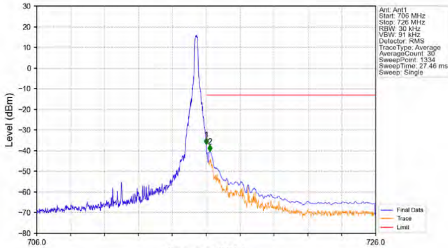
Band17_10MHz_QPSK_HCH_711MHz_RB_1_49_NTV
