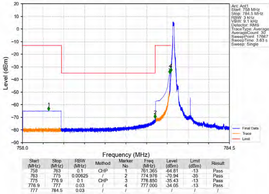
Band13_5MHz_64QAM_LCH_779.5MHz_RB_1_0_NTNV
