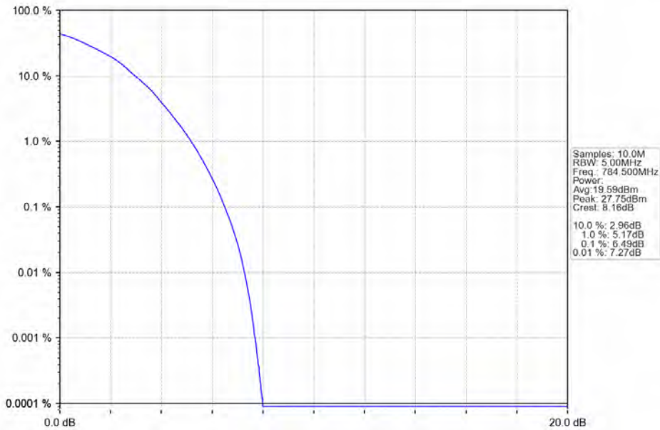
Band13_5MHz_64QAM_HCH_784.5MHz_RB_25_0_NTNV
