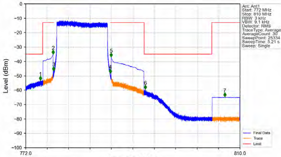
Band13_10MHz_64QAM_HCH_782MHz_RB_50_0_NTNV
