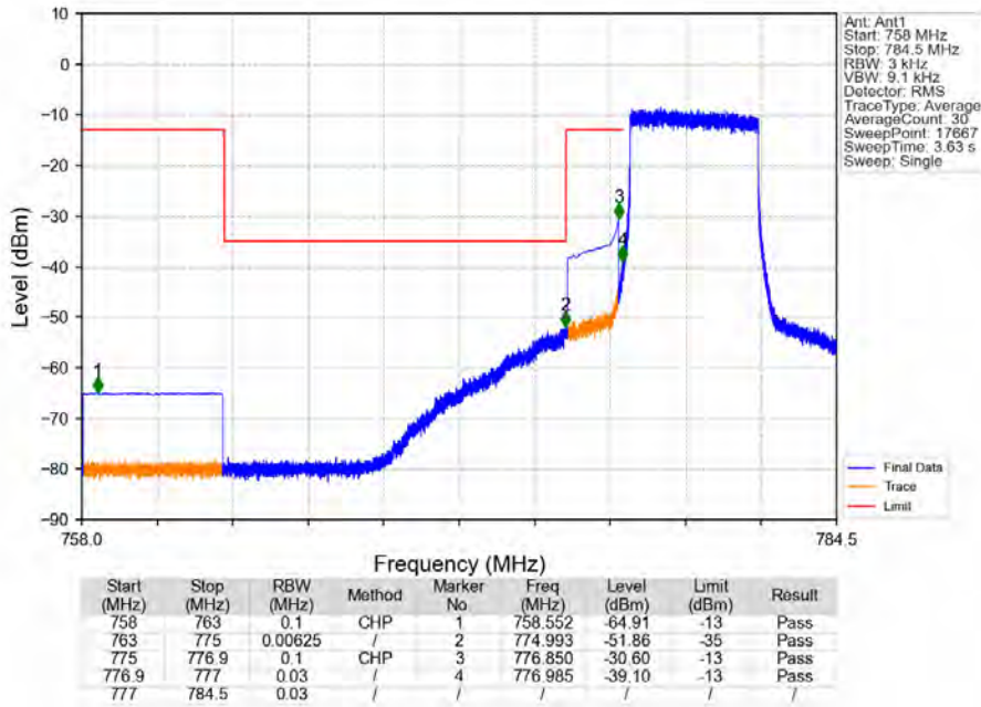
Band13_5MHz_64QAM_LCH_779.5MHz_RB_25_0_NTNV
