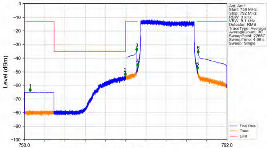
Band13_10MHz_64QAM_LCH_782MHz_RB_50_0_NTNV
