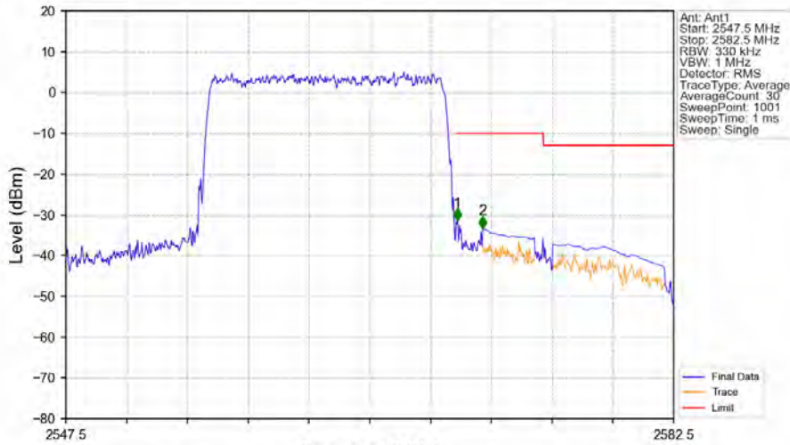
Band7_15MHz_64QAM_HCH_2562.5MHz_RB_75_0_NTNV
