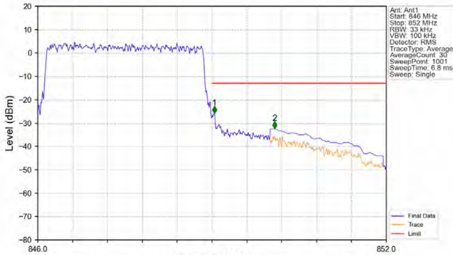
Band5_3MHz_16QAM_HCH_847.5MHz_RB_15_0_NTNV
