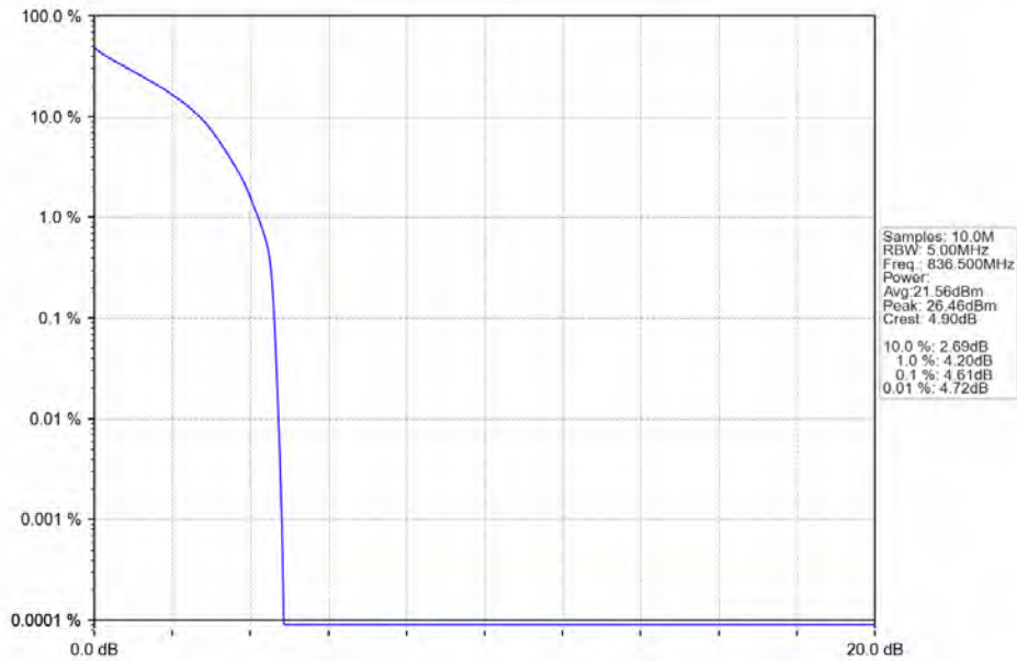
Band5_1.4MHz_QPSK_MCH_836.5MHz_RB_6_0_NTV
