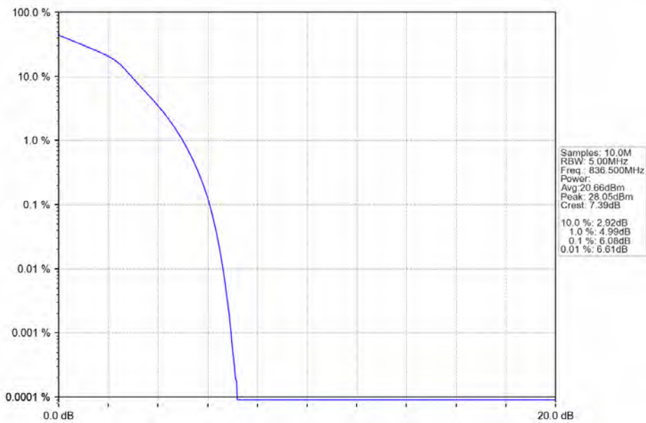
Band5_5MHz_16QAM_MCH_836.5MHz_RB_25_0_NTNV
