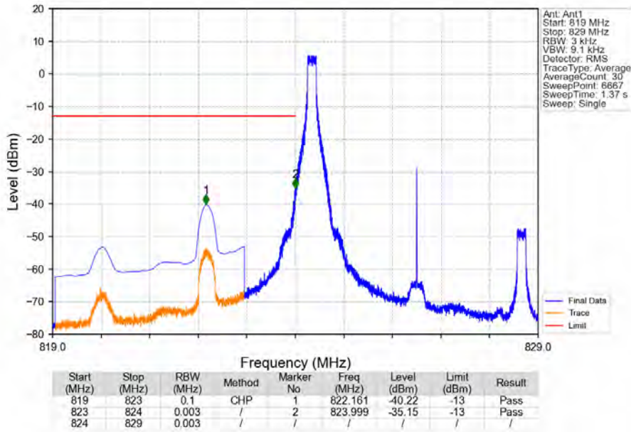
Band5_5MHz_64QAM_LCH_826.5MHz_RB_1_0_NTNV
