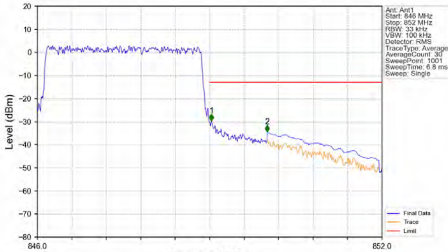
Band5_3MHz_64QAM_HCH_847.5MHz_RB_15_0_NTNV
