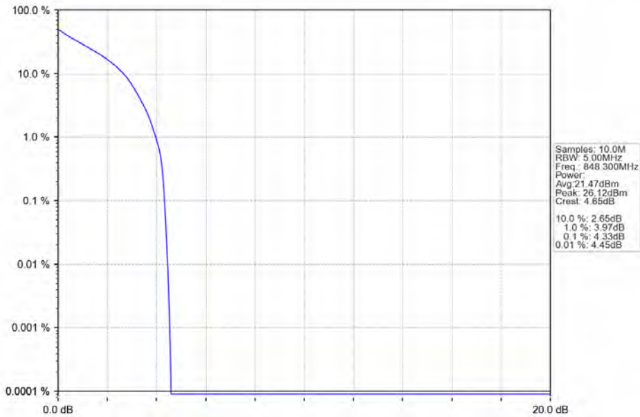
Band5_1.4MHz_QPSK_HCH_848.3MHz_RB_6_0_NTNV
