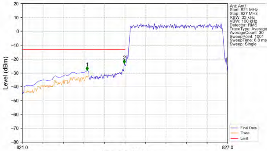
Band5_3MHz_QPSK_LCH_825.5MHz_RB_15_0_NTNV
