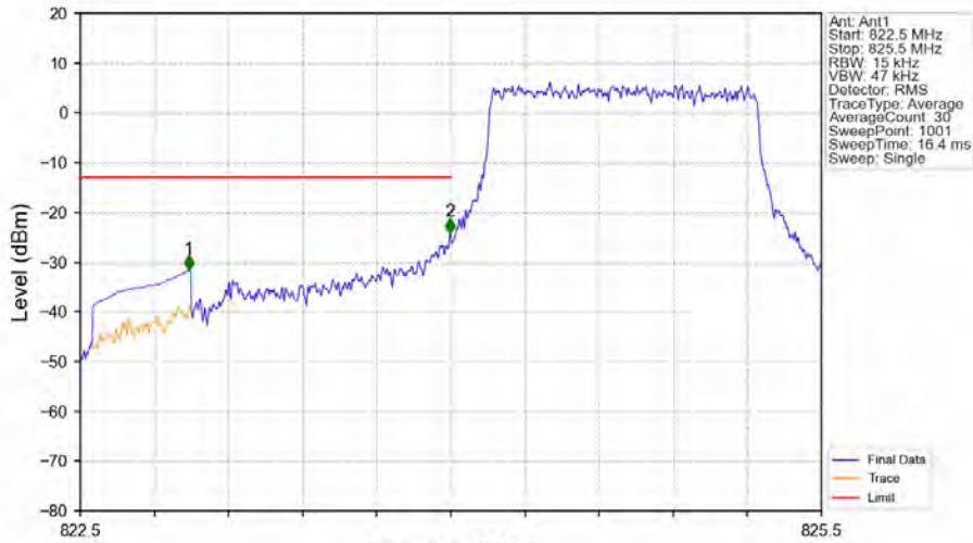
Band5_1.4MHz_QPSK_LCH_824.7MHz_RB_6_0_NTNV
