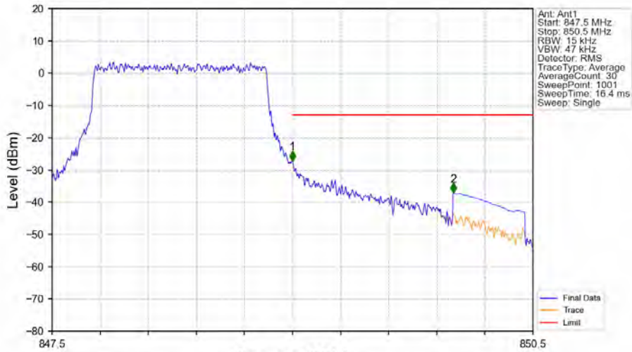
Band5_1.4MHz_64QAM_HCH_848.3MHz_RB_6_0_NTNV
