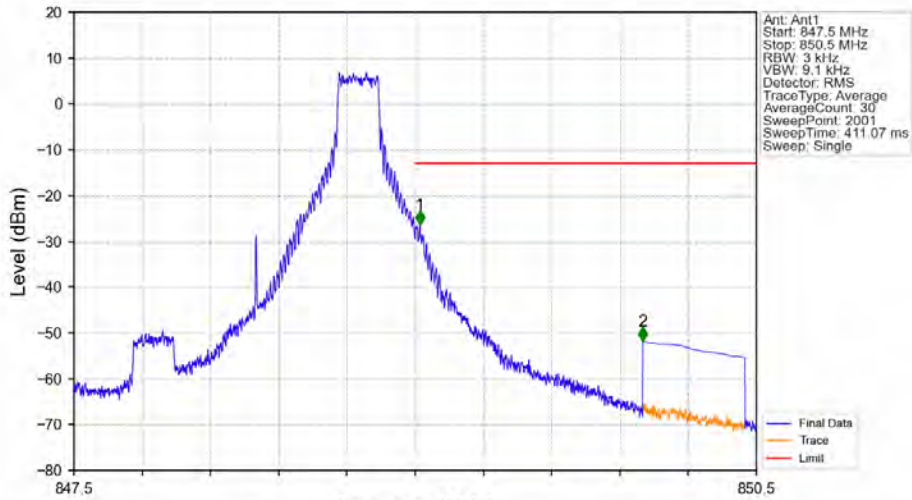
Band5_1.4MHz_QPSK_HCH_848.3MHz_RB_1_5_NTV
