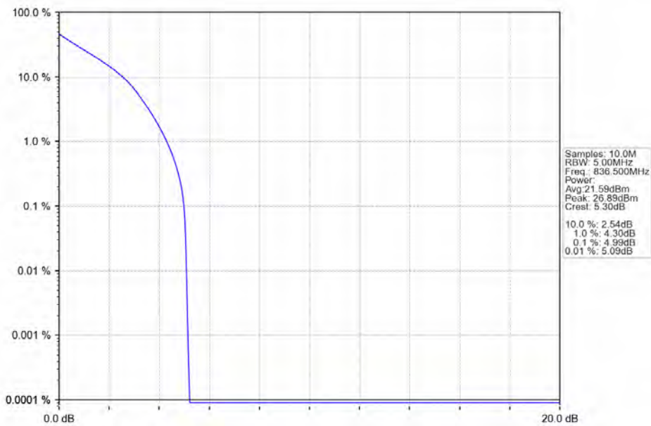
Band5_3MHz_QPSK_MCH_836.5MHz_RB_15_0_NTNV
