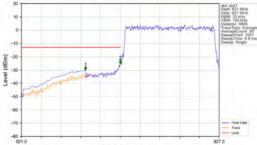
Band5_3MHz_64QAM_LCH_825.5MHz_RB_15_0_NTNV
