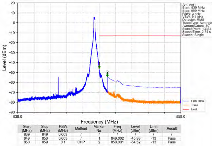
Band5_10MHz_16QAM_HCH_844MHz_RB_1_49_NTNV
