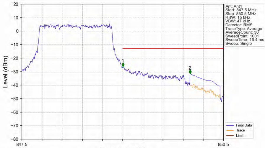
Band5_1.4MHz_QPSK_HCH_848.3MHz_RB_6_0_NTNV
