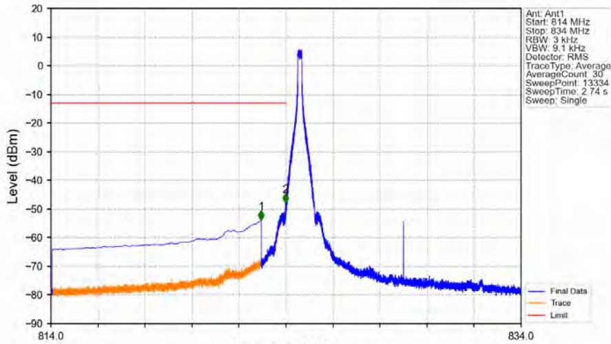
Band5_10MHz_64QAM_LCH_829MHz_RB_1_0_NTNV
