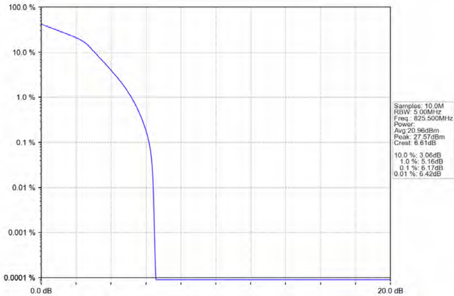
Band5_3MHz_16QAM_LCH_825.5MHz_RB_15_0_NTNV
