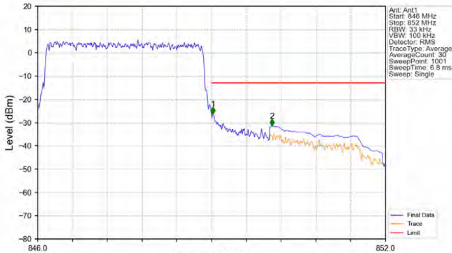
Band5_3MHz_QPSK_HCH_847.5MHz_RB_15_0_NTNV
