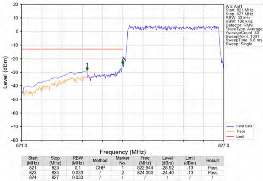
Band5_3MHz_16QAM_LCH_825.5MHz_RB_15_0_NTNV
