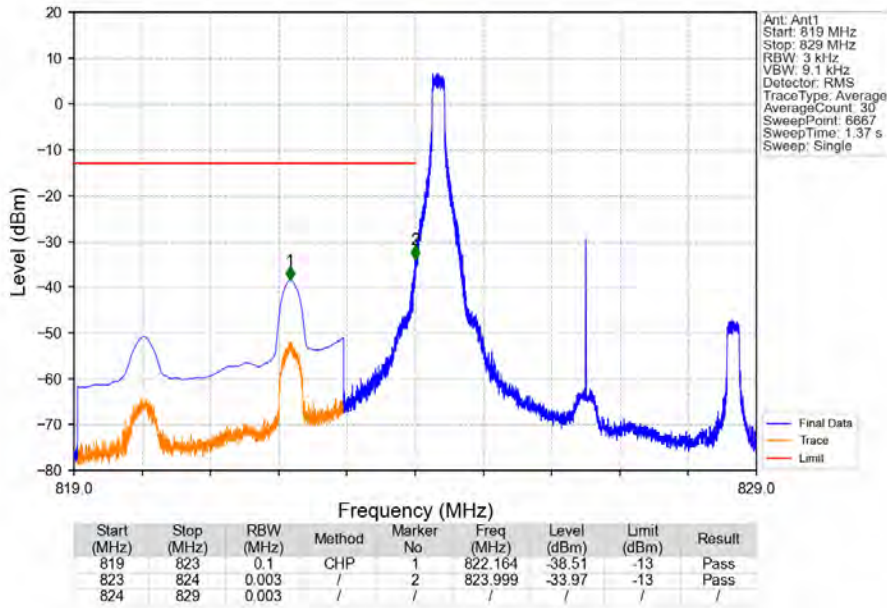
Band5_5MHz_16QAM_LCH_826.5MHz_RB_1_0_NTNV
