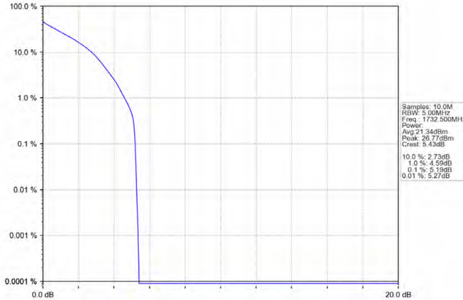
Band4 1.4MHz QPSK MCH 1732.5MHz RB 6 0 NTV
