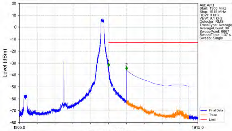
Band2_5MHz_QPSK_HCH_1907.5MHz_RB_1_24_NTNV
