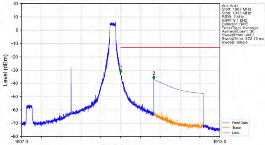
Band2_3MHz_16QAM_HCH_1908.5MHz_RB_1_14_NTNV
