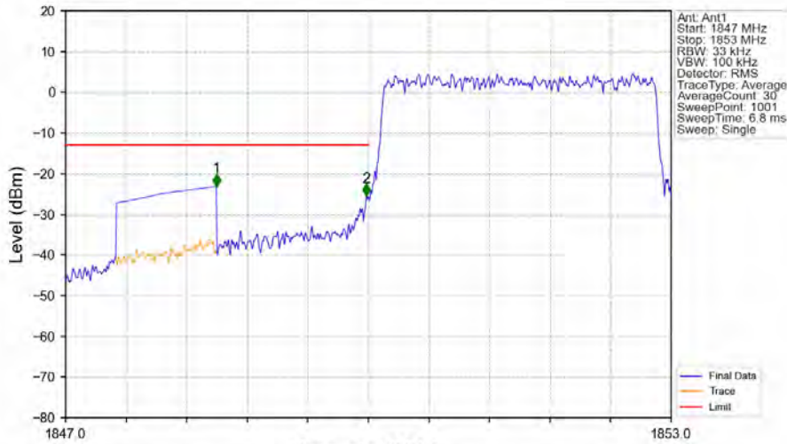
Band2_3MHz_16QAM_LCH_1851.5MHz_RB_15_0_NTNV
