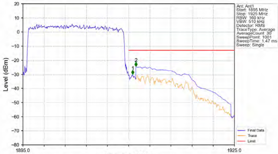
Band2_15MHz_QPSK_HCH_1902.5MHz_RB_75_0_NTNV
