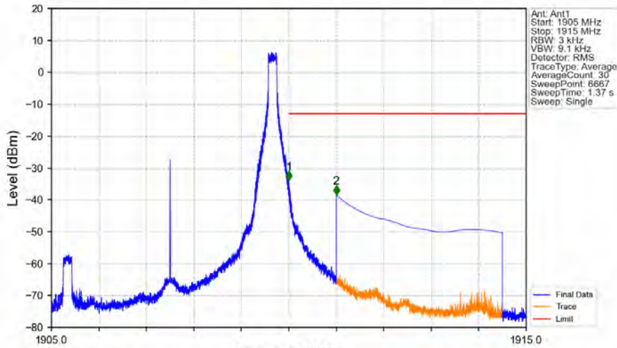
Band2_5MHz_16QAM_HCH_1907.5MHz_RB_1_24_NTNV
