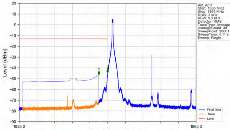
Band2_15MHz_64QAM_LCH_1857.5MHz_RB_1_0_NTNV
