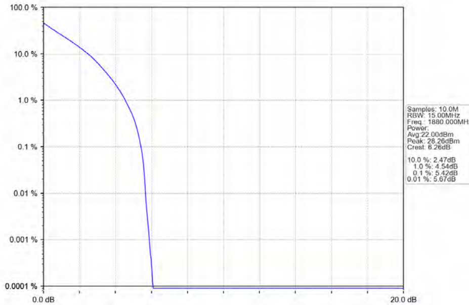
Band2_15MHz_QPSK_MCH_1880MHz_RB_75_0_NTNV
