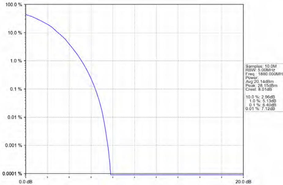
Band2_5MHz_64QAM_MCH_1880MHz_RB_25_0_NTNV
