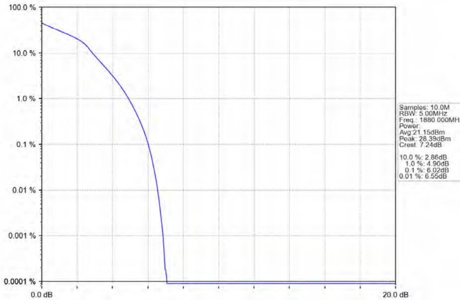
Band2_5MHz_16QAM_MCH_1880MHz_RB_25_0_NTNV
