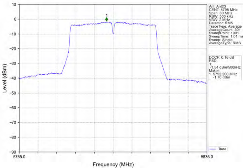
802.11ac(VHT40)_HCH_5795MHz_Ant23_NTNV
