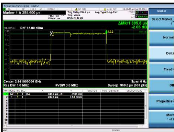
8-DPSK 3DH1
