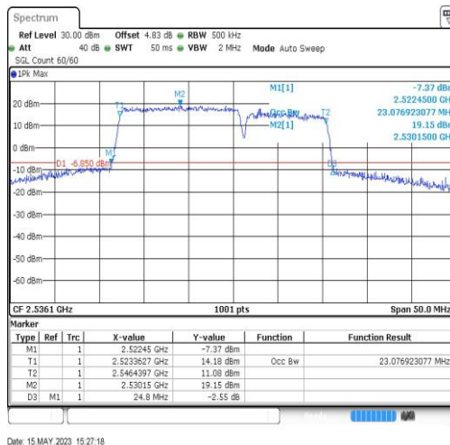
7-7-15MHz-10MHz-64QAM-64QAM-21051-21171-75RB#0-50RB#0-23.077
