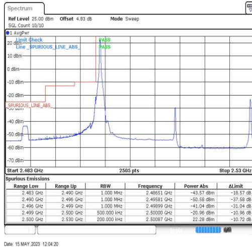
7-7-15MHz-15MHz-QPSK-QPSK-20825-20975-1RB#0-0RB#0
