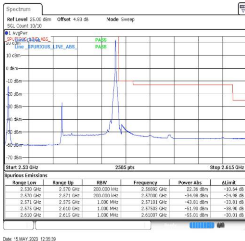
7-7-20MHz-20MHz-QPSK-QPSK-21152-21350-0RB#0-1RB#99
