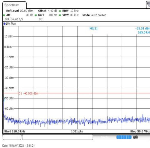
7-7-20MHz-20MHz-QPSK-QPSK-21152-21350-1RB#0-0RB#0-0.15~30MHz
