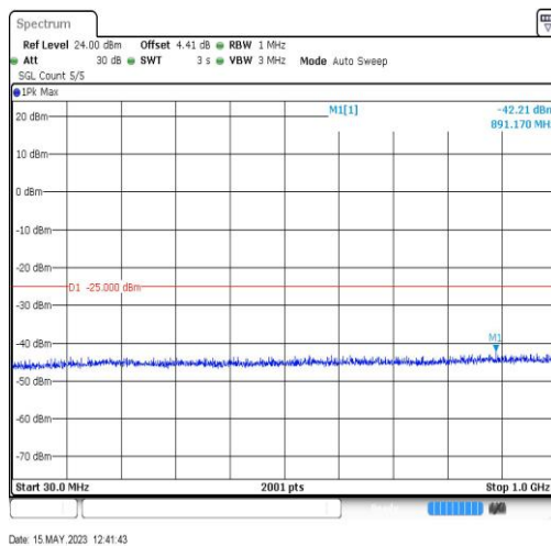
7-7-20MHz-20MHz-QPSK-QPSK-21152-21350-1RB#0-0RB#0-30~1000MHz
