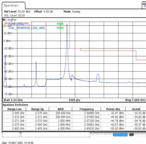
7-7-20MHz-10MHz-QPSK-QPSK-21251-21395-0RB#0-1RB#49
