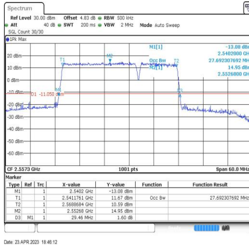
7-7-20MHz-10MHz-16QAM-16QAM-21251-21395-100RB#0-50RB#0-27.692
