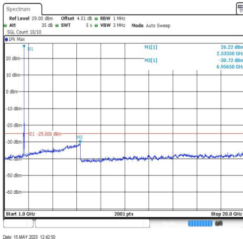
7-7-20MHz-20MHz-QPSK-QPSK-21152-21350-1RB#0-0RB#0-1000~20000MHz
