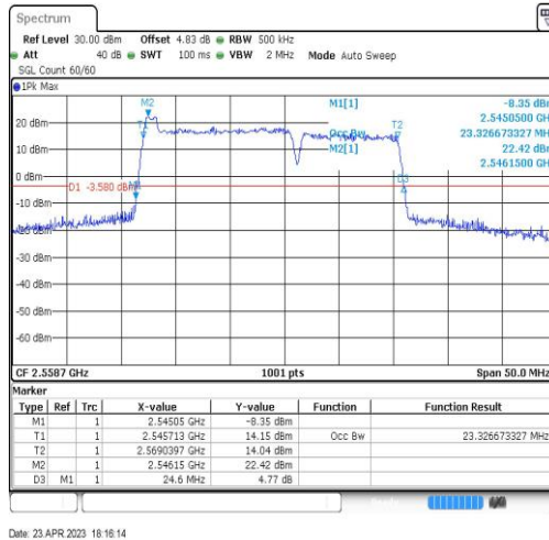
7-7-15MHz-10MHz-16QAM-16QAM-21277-21397-75RB#0-50RB#0-23.327
