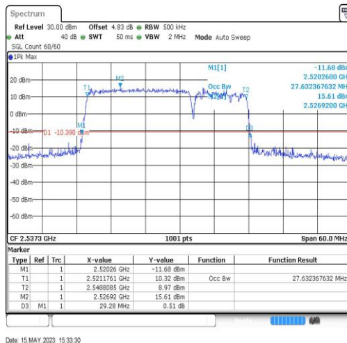
7-7-20MHz-10MHz-64QAM-64QAM-21051-21195-100RB#0-50RB#0-27.632
