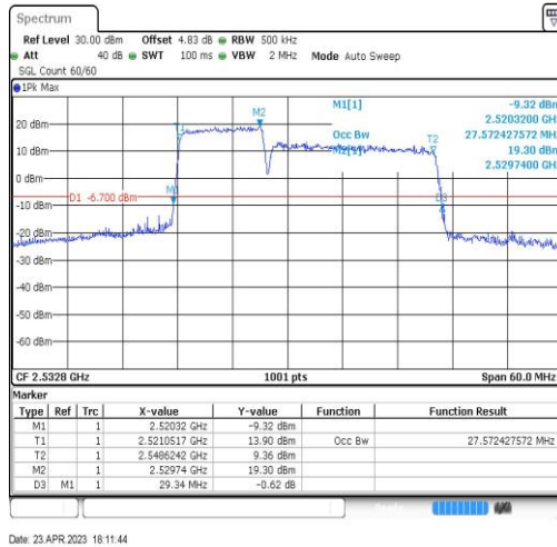
7-7-10MHz-20MHz-QPSK-QPSK-21006-21150-50RB#0-100RB#0-27.572
