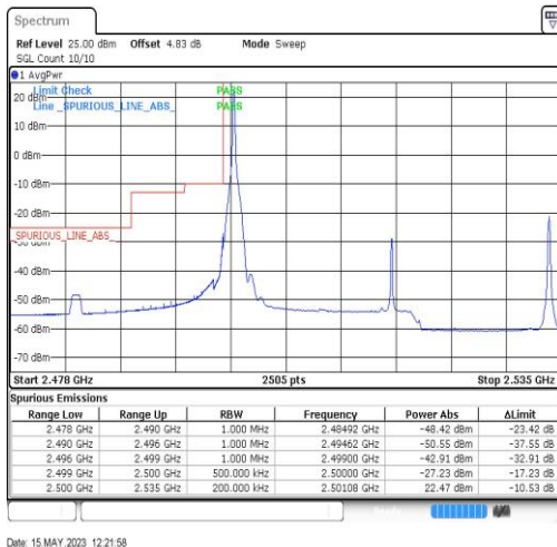
7-7-20MHz-15MHz-QPSK-QPSK-20850-21021-1RB#0-0RB#0
