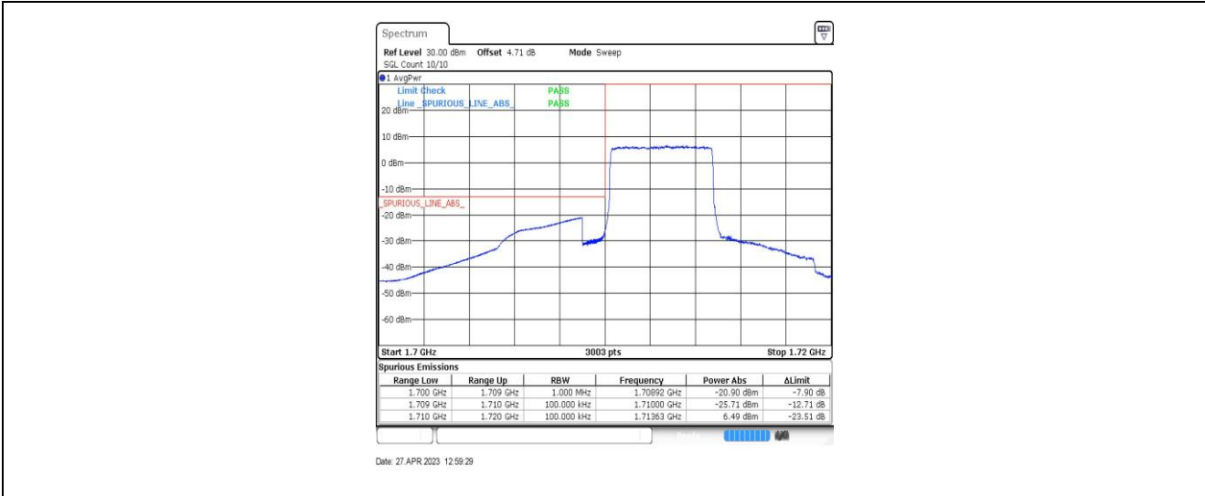
Band66-5MHz-QPSK-131997-25RB#0
