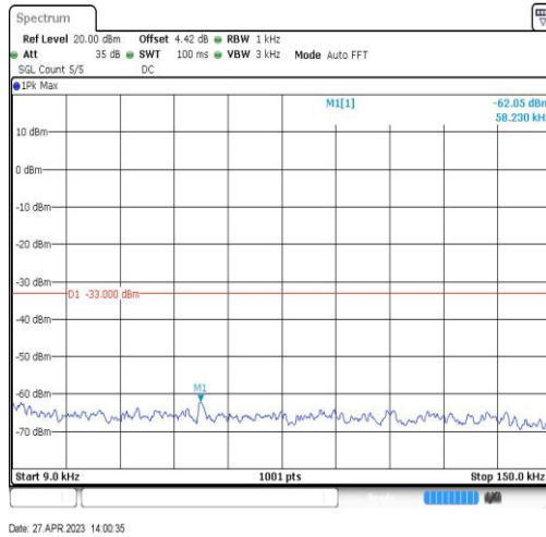
Band66-20MHz-QPSK-132572-1RB#0-Range1:0.009~0.15MHz
