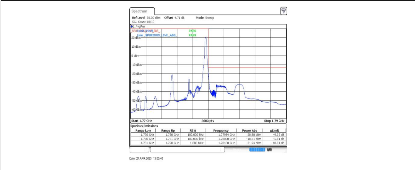
Band66-5MHz-QPSK-132647-1RB#24
