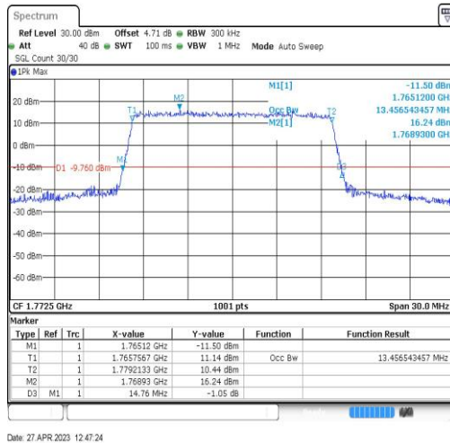
Band66-15MHz-16QAM-132597-75RB#0-13.457
