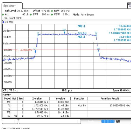
Band66-20MHz-QPSK-132572-100RB#0-17.902
