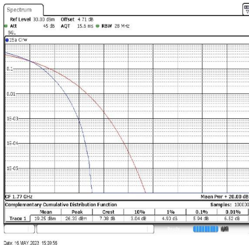
Band66-20MHz-16QAM-132572-100RB#0
