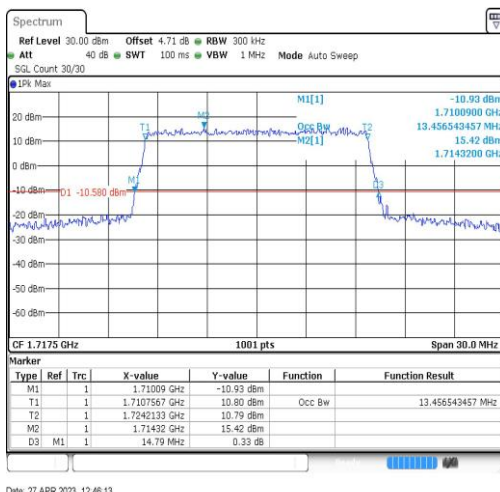
Band66-15MHz-16QAM-132047-75RB#0-13.457
