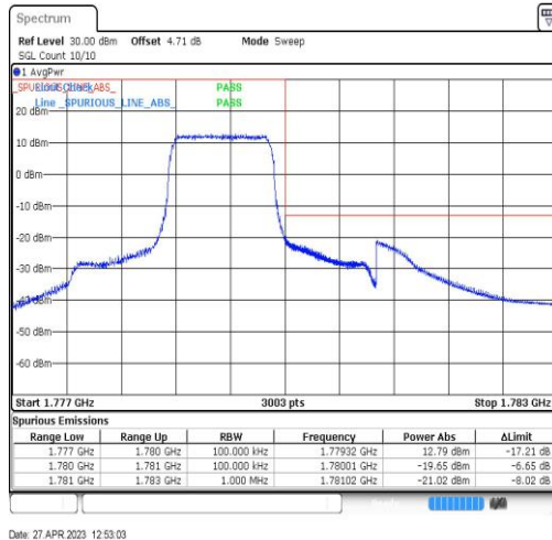
Band66-1.4MHz-QPSK-132665-6RB#0
