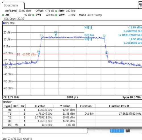
Band66-20MHz-16QAM-132572-100RB#0-17.862
