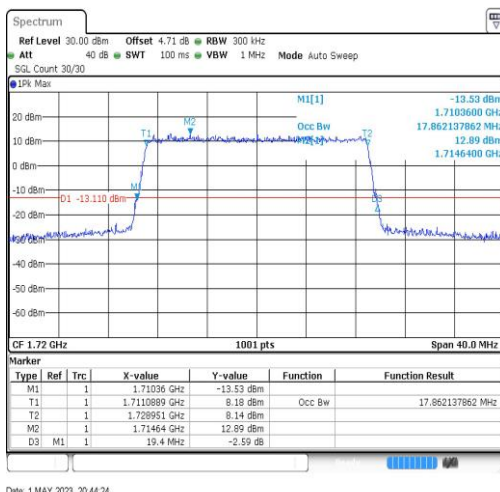
Band66-20MHz-64QAM-132072-100RB#0-17.862
