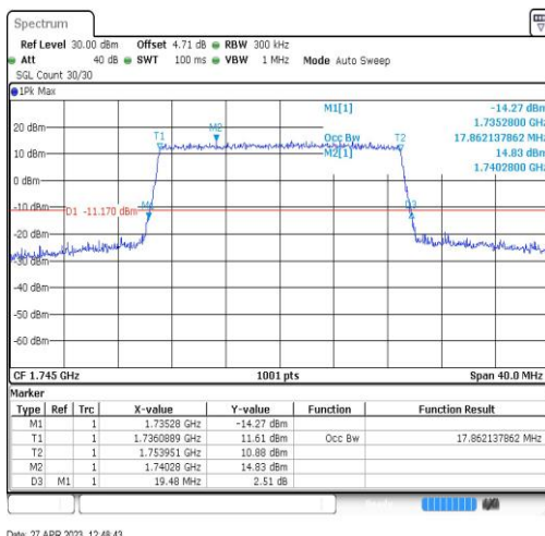
Band66-20MHz-16QAM-132322-100RB#0-17.862
