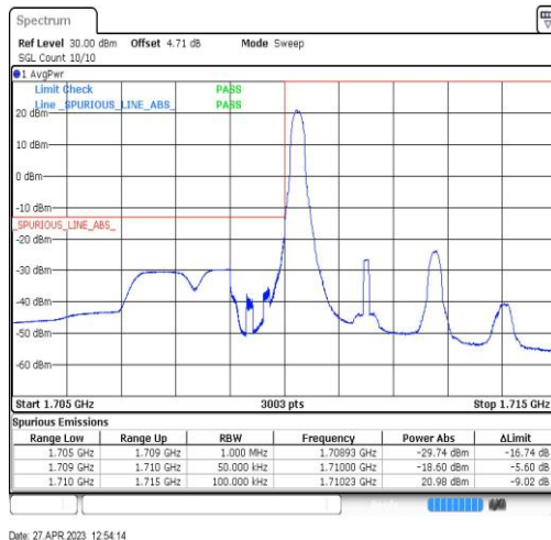
Band66-3MHz-QPSK-131987-1RB#0
