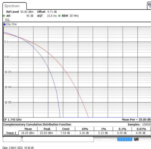
Band66-20MHz-64QAM-132322-100RB#0
