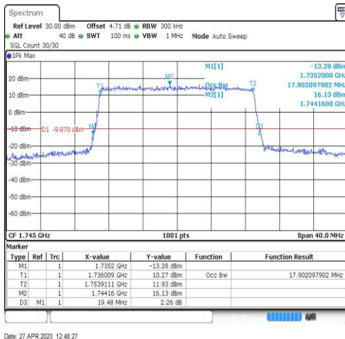
Band66-20MHz-QPSK-132322-100RB#0-17.902
