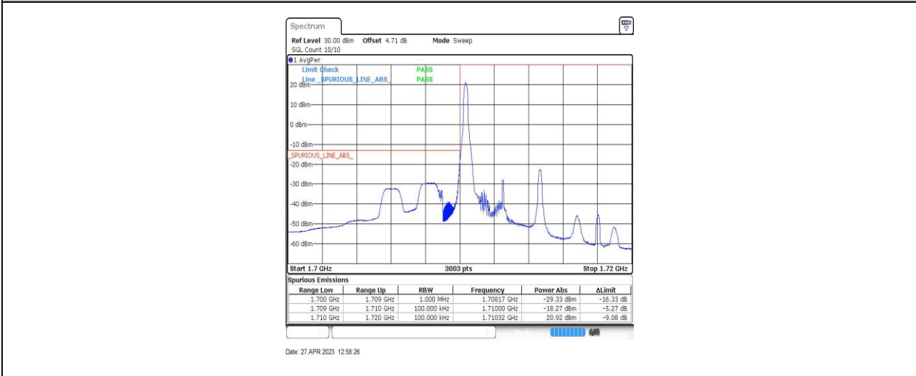
Band66-5MHz-QPSK-131997-1RB#0
