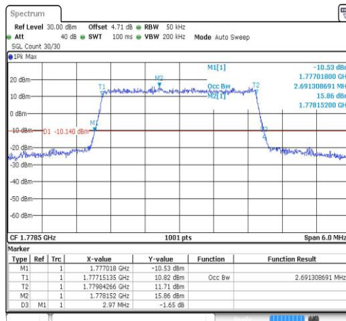
Band66-3MHz-QPSK-132322-15RB#0-2.697
