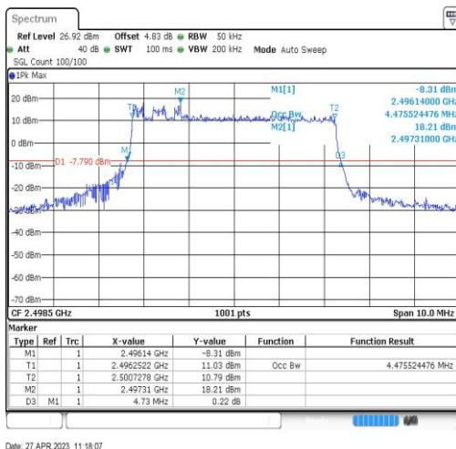
Band41-5MHz-QPSK-39675-25RB#0-4.476
