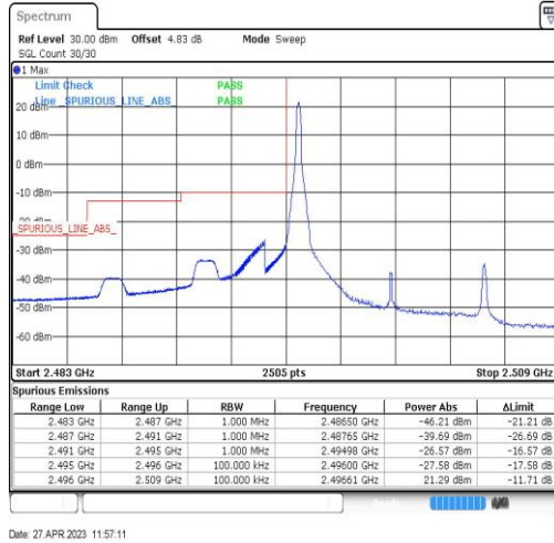
Band41-10MHz-QPSK-39700-1RB#0
