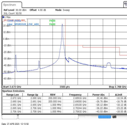
Band41-15MHz-QPSK-41515-1RB#74
