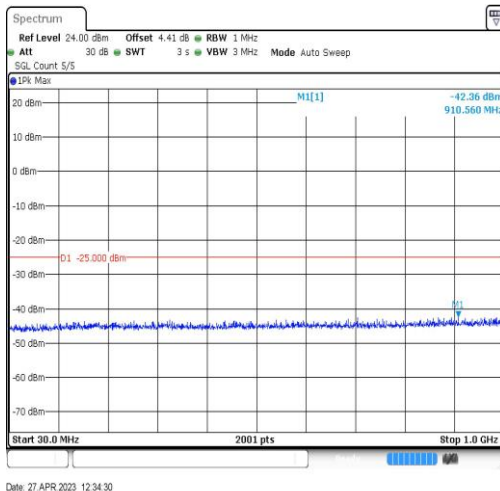
Band41-20MHz-QPSK-41490-1RB#0-Range3:30~1000MHz
