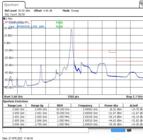
Band41-5MHz-QPSK-41565-1RB#24
