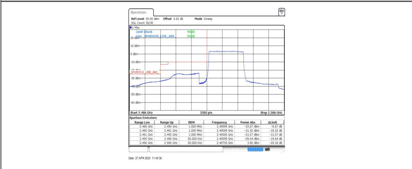
Band41-5MHz-QPSK-39675-25RB#0
