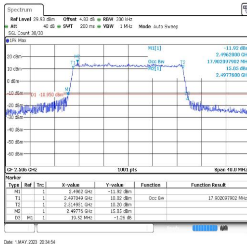
Band41-20MHz-64QAM-39750-100RB#0-17.902
