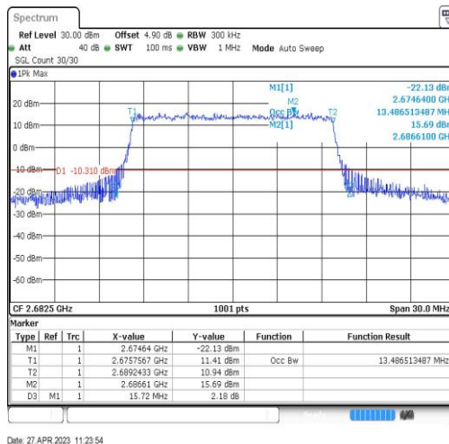
Band41-15MHz-16QAM-41515-75RB#0-13.487
