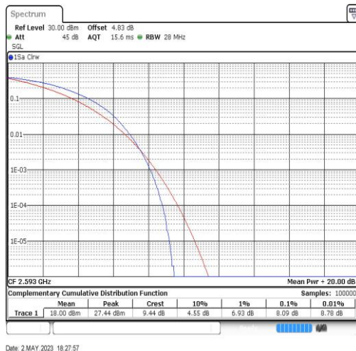
Band41-20MHz-64QAM-40620-100RB#0
