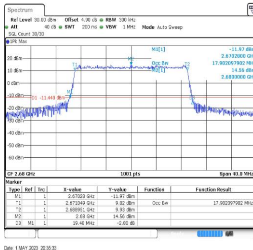
Band41-20MHz-64QAM-41490-100RB#0-17.902
