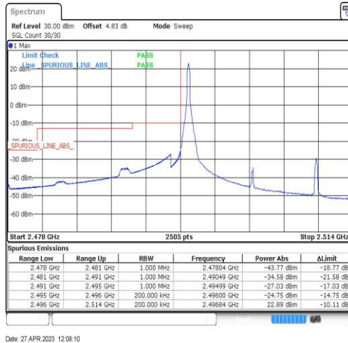
Band41-15MHz-QPSK-39725-1RB#0
