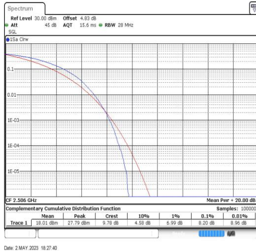
Band41-20MHz-64QAM-39750-100RB#0
