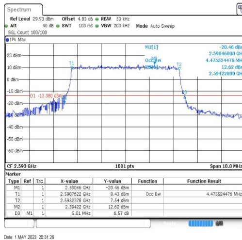
Band41-5MHz-64QAM-40620-25RB#0-4.476
