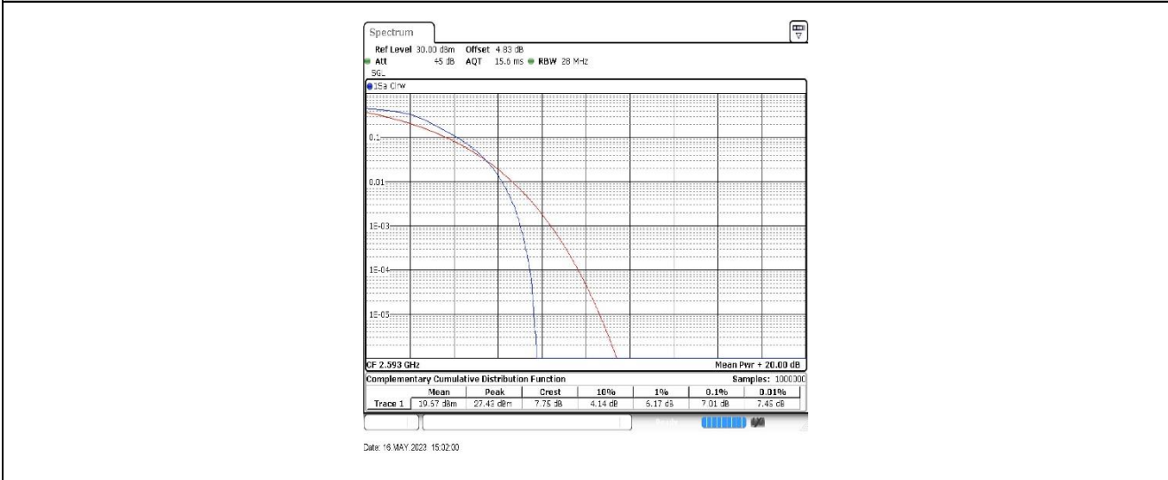
Band41-20MHz-QPSK-40620-100RB#0
