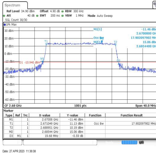
Band41-20MHz-16QAM-41490-100RB#0-17.902
