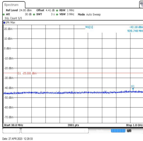
Band41-20MHz-QPSK-39750-1RB#0-Range3:30~1000MHz
