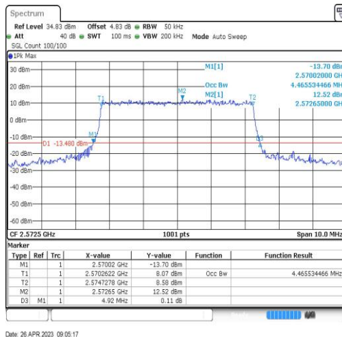
Band38-5MHz-16QAM-37775-25RB#0-4.466
