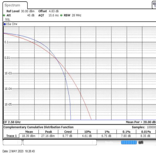
Band38-20MHz-64QAM-37850-100RB#0
