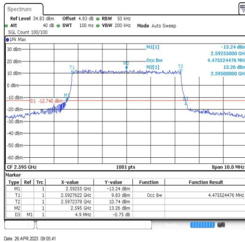
Band38-5MHz-QPSK-38000-25RB#0-4.476
