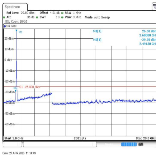
Band38-20MHz-QPSK-38150-1RB#0-Range4:1000~20000MHz
