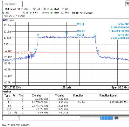
Band38-5MHz-QPSK-37775-25RB#0-4.476
