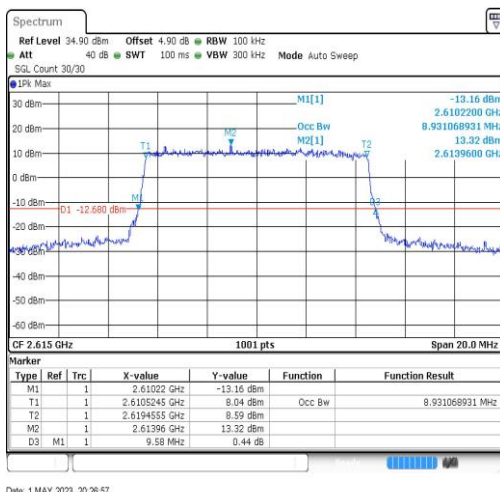
Band38-10MHz-64QAM-38200-50RB#0-8.931
