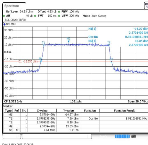
Band38-10MHz-64QAM-37800-50RB#0-8.931
