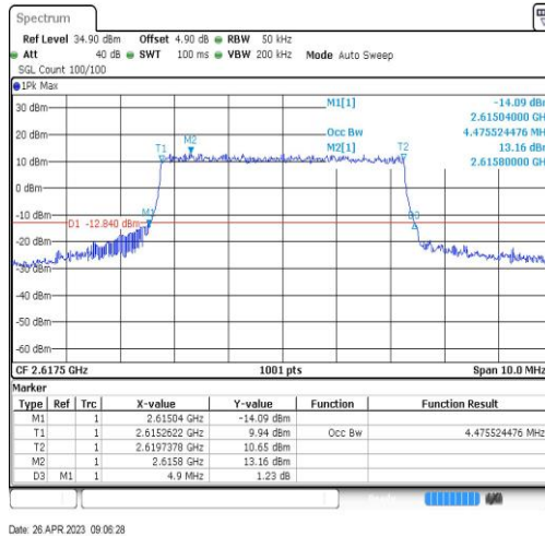
Band38-5MHz-QPSK-38225-25RB#0-4.476
