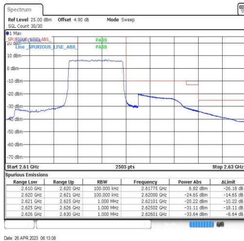
Band38-5MHz-QPSK-38225-25RB#0
