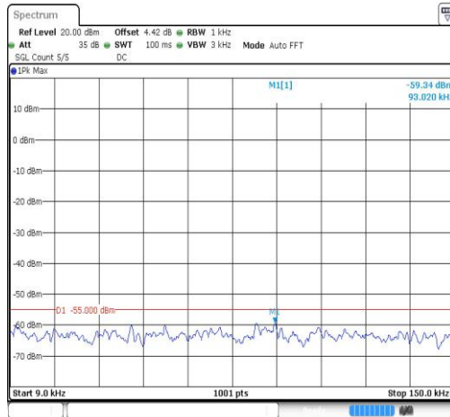
Band38-20MHz-QPSK-38150-1RB#0-Range1:0.009~0.15MHz
