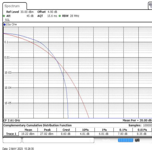
Band38-20MHz-16QAM-38150-100RB#0
