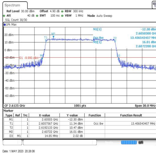
Band38-15MHz-64QAM-38175-75RB#0-13.457
