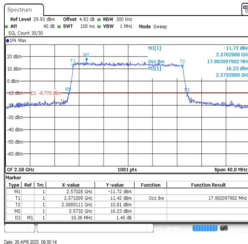
Band38-20MHz-QPSK-37850-100RB#0-17.902
