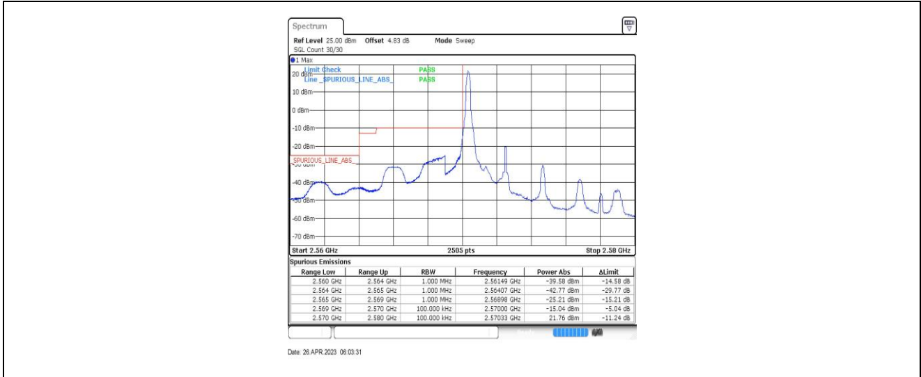
Band38-5MHz-QPSK-37775-1RB#0
