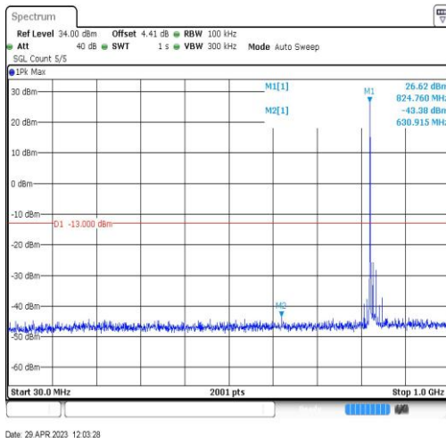
Band26-15MHz-QPSK-26865-1RB#0-Range3:30~1000MHz
