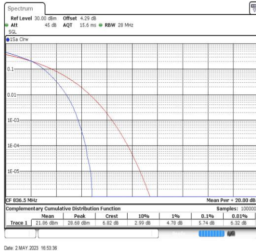
Band26-15MHz-16QAM-26915-75RB#0
