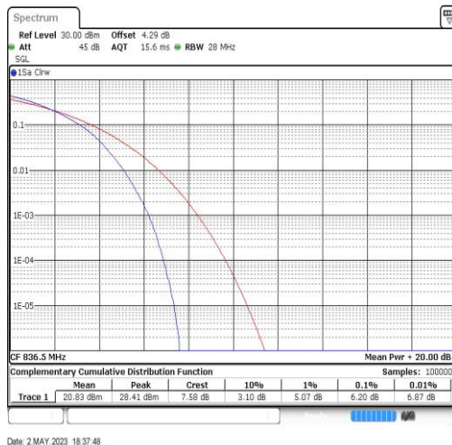
Band26-15MHz-64QAM-26915-75RB#0
