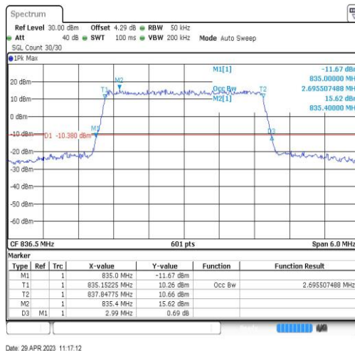
Band26-3MHz-16QAM-26915-15RB#0-2.696
