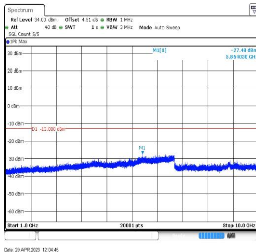
Band26-15MHz-QPSK-26965-1RB#0-Range4:1000~10000MHz
