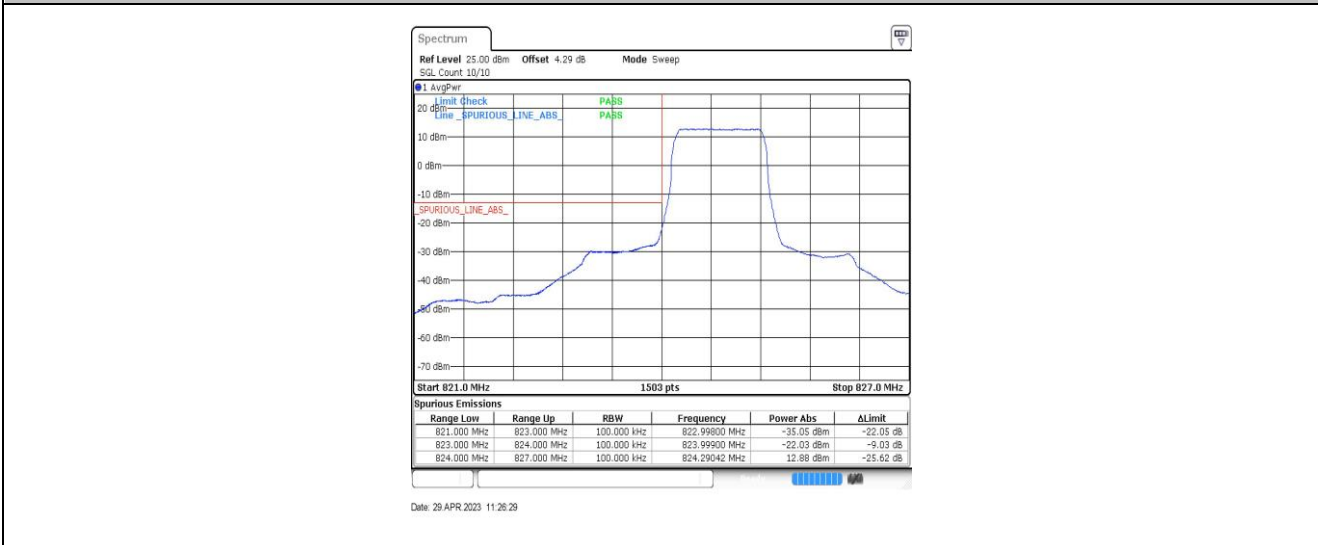
Band26-1.4MHz-QPSK-26797-6RB#0
