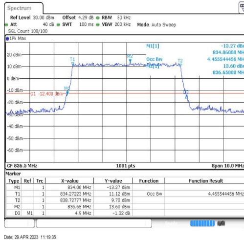
Band26-5MHz-16QAM-26915-25RB#0-4.456
