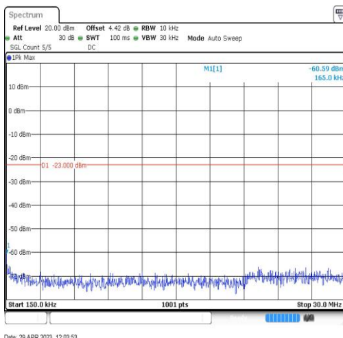
Band26-15MHz-QPSK-26915-1RB#0-Range2:0.15~30MHz
