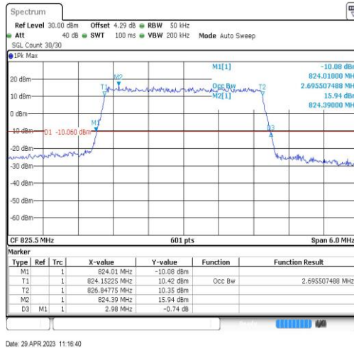
Band26-3MHz-16QAM-26805-15RB#0-2.696
