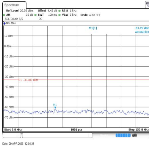
Band26-15MHz-QPSK-26965-1RB#0-Range1:0.009~0.15MHz
