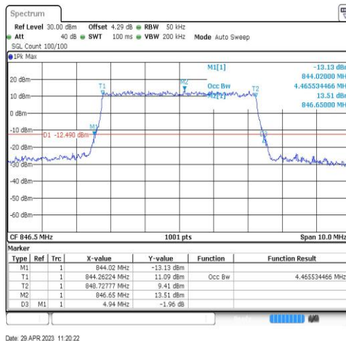
Band26-5MHz-16QAM-27015-25RB#0-4.466
