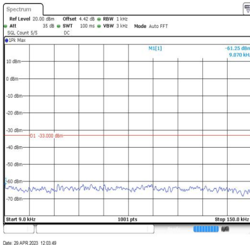
Band26-15MHz-QPSK-26915-1RB#0-Range1:0.009~0.15MHz
