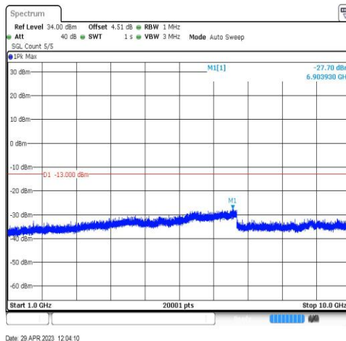
Band26-15MHz-QPSK-26915-1RB#0-Range4:1000~10000MHz
