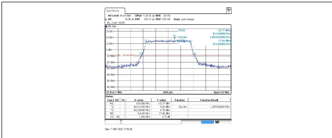
Band26-1.4MHz-QPSK-26697-6RB#0-2.97
