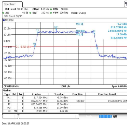
Band26-3MHz-QPSK-26740-15RB#0-2.691
