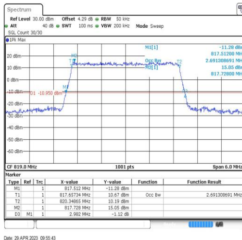
Band26-3MHz-16QAM-26740-15RB#0-2.691
