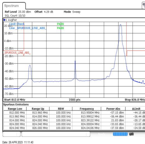
Band26-10MHz-QPSK-26740-1RB#49
