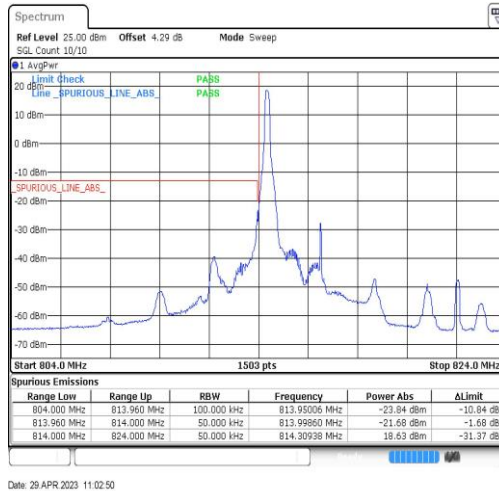
Band26-5MHz-QPSK-26715-1RB#0
