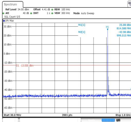
Band26-10MHz-QPSK-26740-1RB#0-Range3:30~1000MHz
