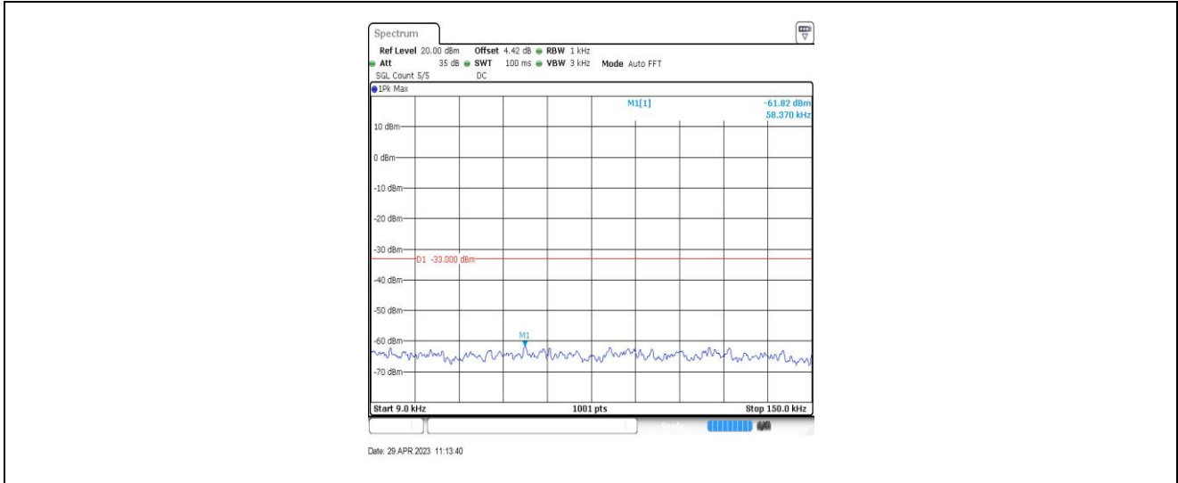
Band26-10MHz-QPSK-26740-1RB#0-Range1:0.009~0.15MHz
