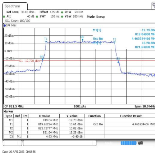
Band26-5MHz-16QAM-26765-25RB#0-4.466
