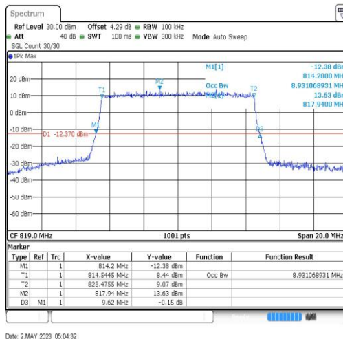
Band26-10MHz-64QAM-26740-50RB#0-8.931
