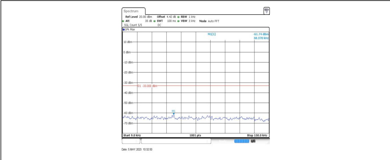
Band19-15MHz-QPSK-24075-1RB#0-Range1:0.009~0.15MHz
