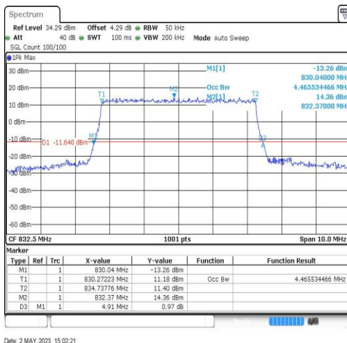
Band19-5MHz-QPSK-24025-25RB#0-4.466
