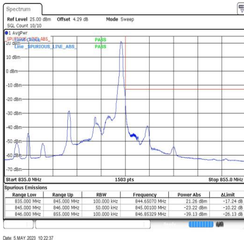
Band19-5MHz-QPSK-24125-1RB#24
