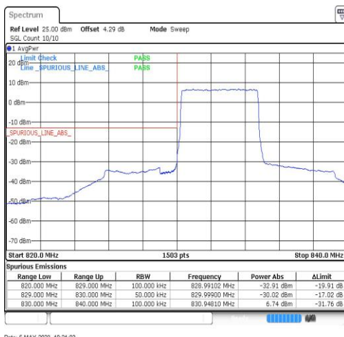
Band19-5MHz-QPSK-24025-25RB#0
