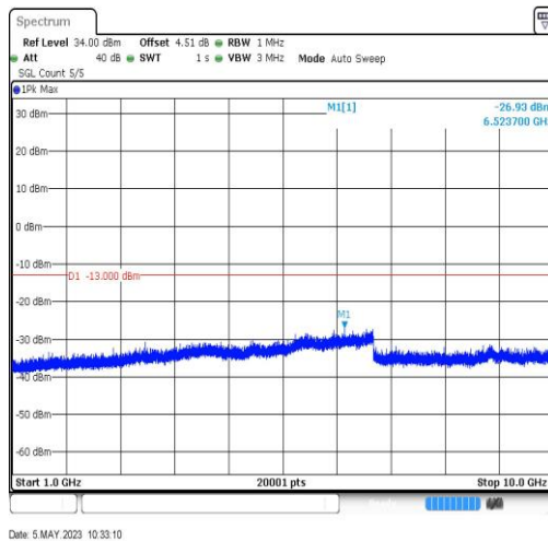
Band19-15MHz-QPSK-24075-1RB#0-Range4:1000~10000MHz
