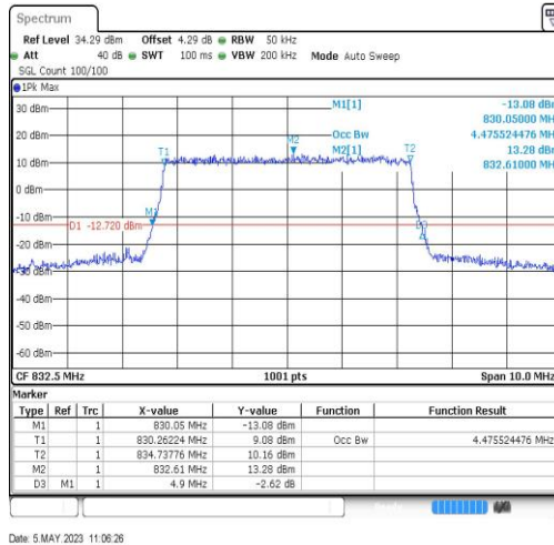
Band19-5MHz-64QAM-24025-25RB#0-4.476
