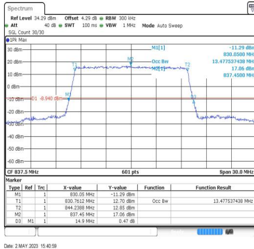
Band19-15MHz-QPSK-24075-75RB#0-13.478
