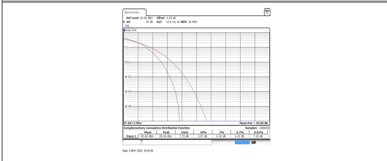
Band19-15MHz-16QAM-24075-75RB#0
