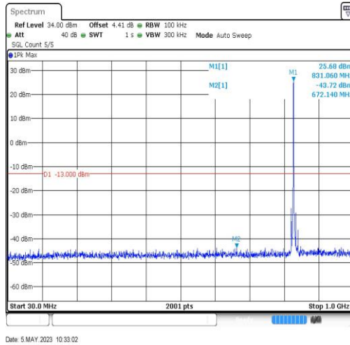
Band19-15MHz-QPSK-24075-1RB#0-Range3:30~1000MHz
