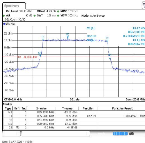
Band19-10MHz-64QAM-24100-50RB#0-8.918
