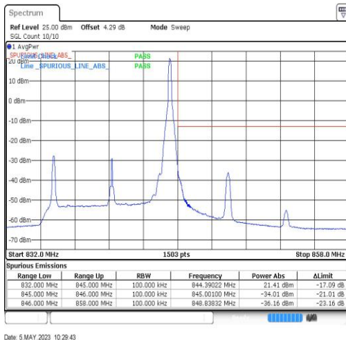
Band19-10MHz-QPSK-24100-1RB#49
