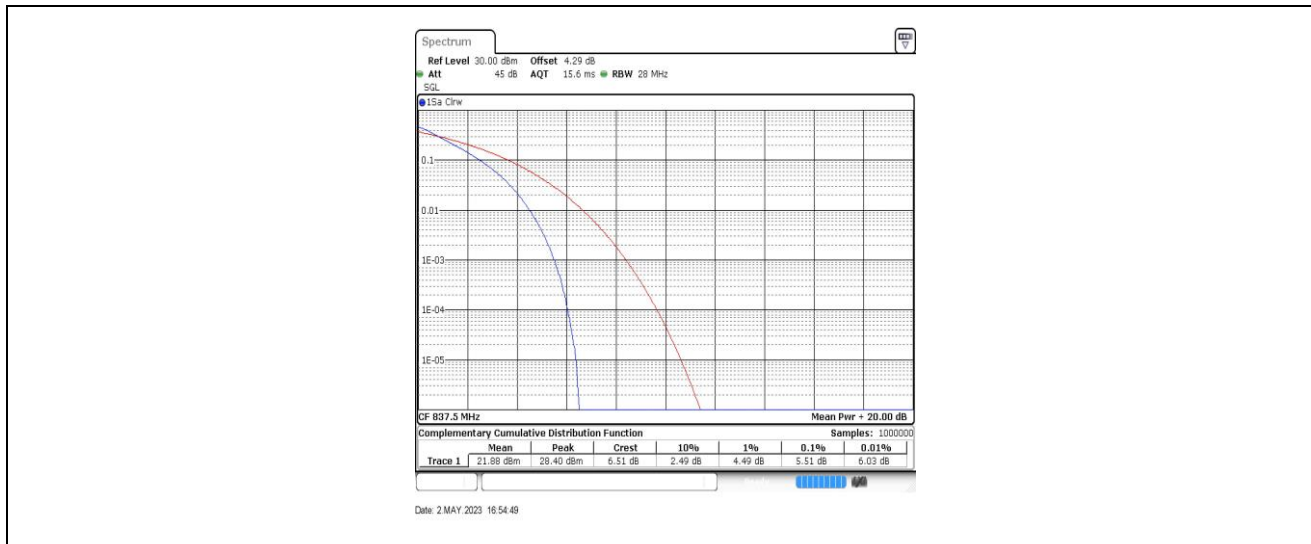
Band19-15MHz-QPSK-24075-75RB#0
