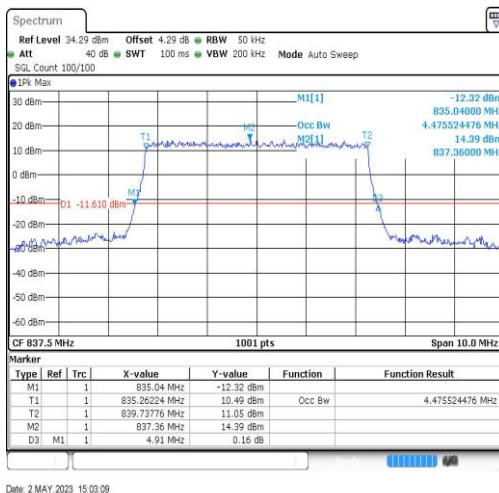
Band19-5MHz-QPSK-24075-25RB#0-4.476
