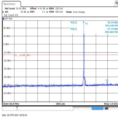
Band17-10MHz-QPSK-23780-1RB#0-Range3:30~1000MHz
