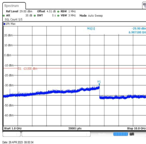
Band17-10MHz-QPSK-23780-1RB#0-Range4:1000~10000MHz
