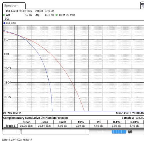
Band17-10MHz-16QAM-23780-50RB#0
