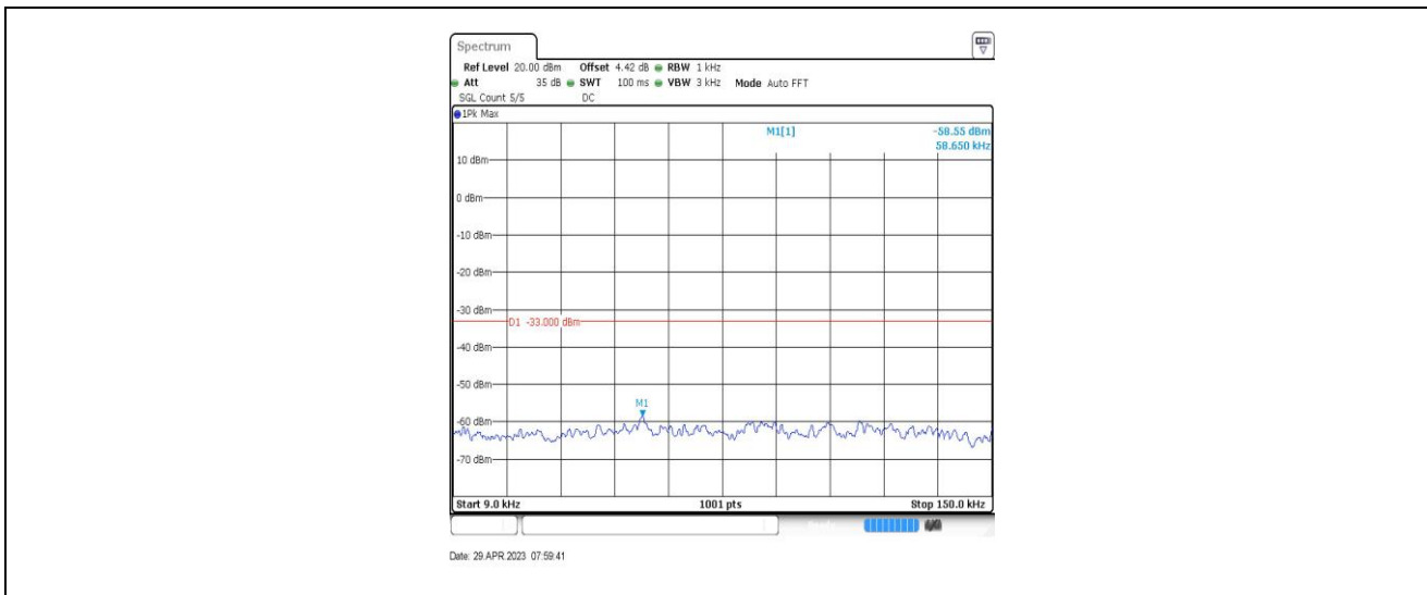
Band17-10MHz-QPSK-23780-1RB#0-Range1:0.009~0.15MHz
