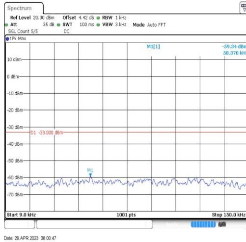
Band17-10MHz-QPSK-23790-1RB#0-Range1:0.009~0.15MHz
