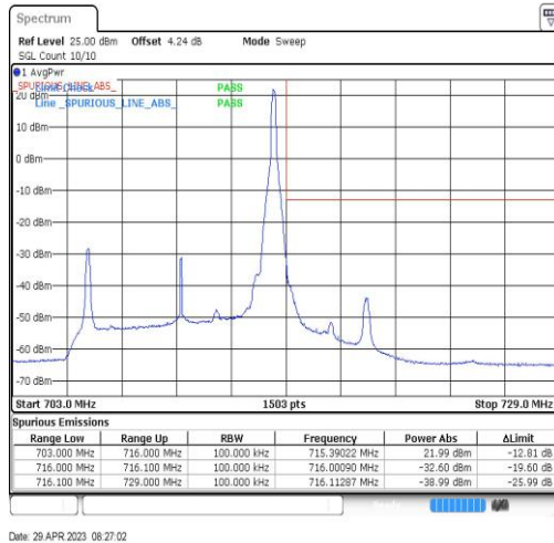
Band17-10MHz-QPSK-23800-1RB#49
