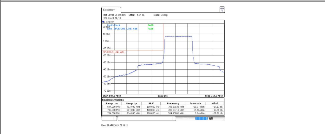
Band17-5MHz-QPSK-23755-25RB#0
