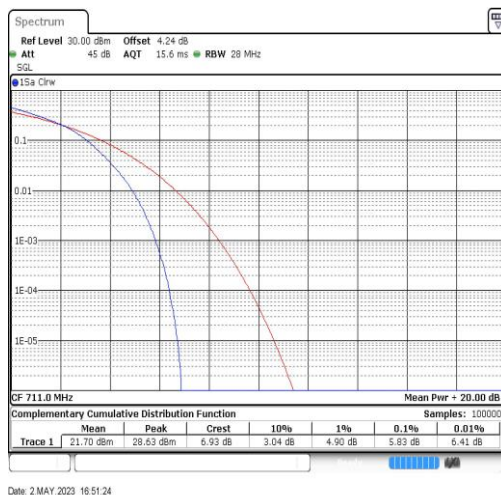
Band17-10MHz-16QAM-23800-50RB#0
