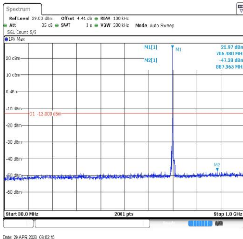
Band17-10MHz-QPSK-23800-1RB#0-Range3:30~1000MHz
