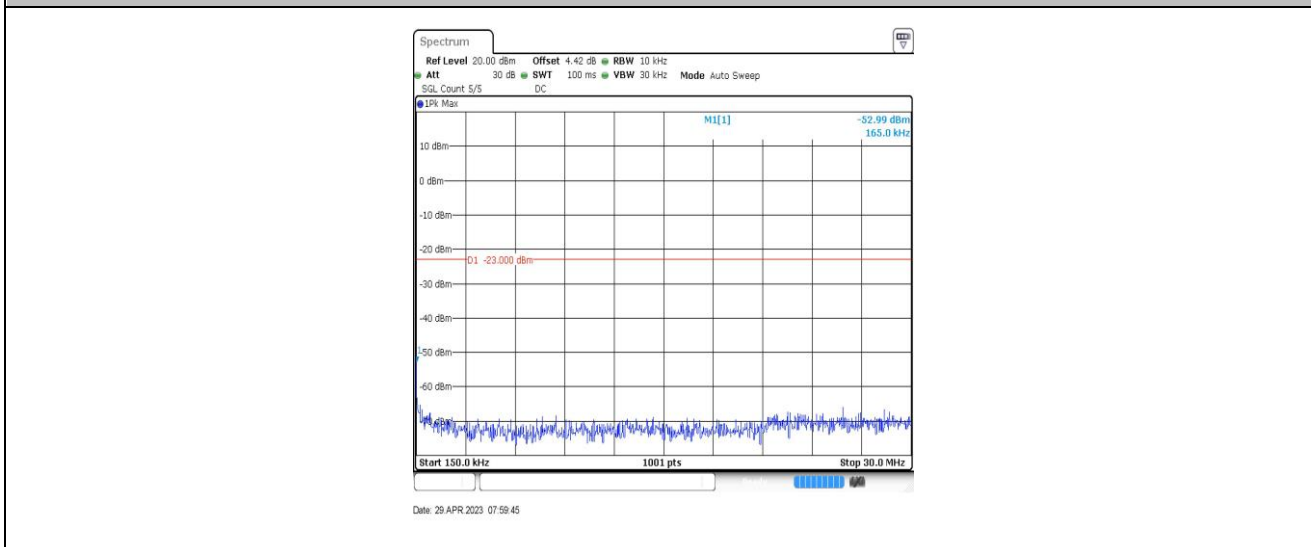
Band17-10MHz-QPSK-23780-1RB#0-Range2:0.15~30MHz
