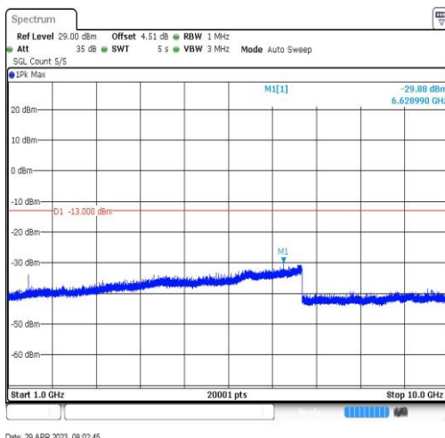
Band17-10MHz-QPSK-23800-1RB#0-Range4:1000~10000MHz
