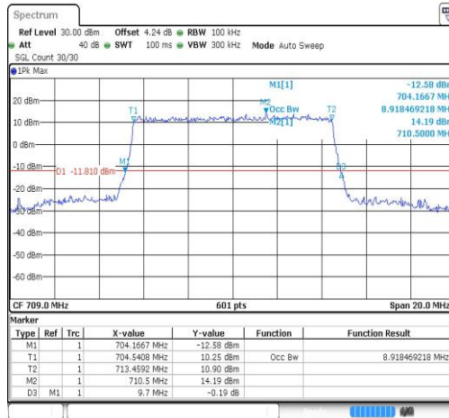
Band17-10MHz-16QAM-23780-50RB#0-8.918
