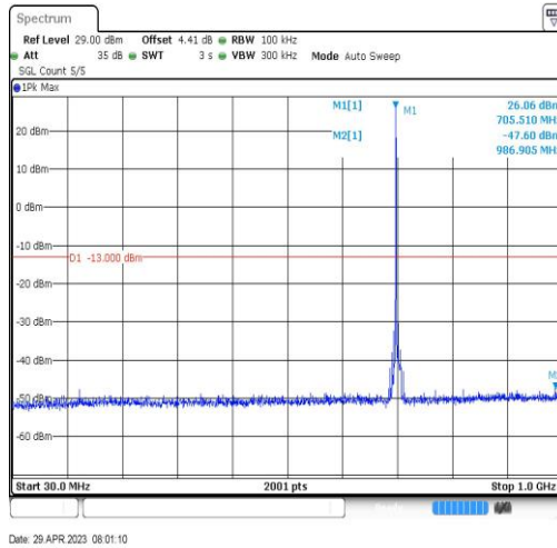
Band17-10MHz-QPSK-23790-1RB#0-Range3:30~1000MHz
