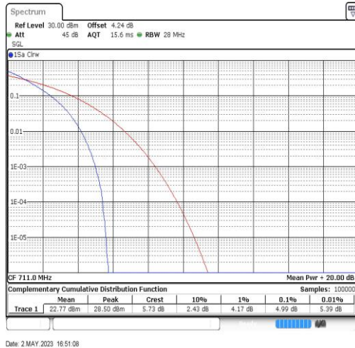
Band17-10MHz-QPSK-23800-50RB#0
