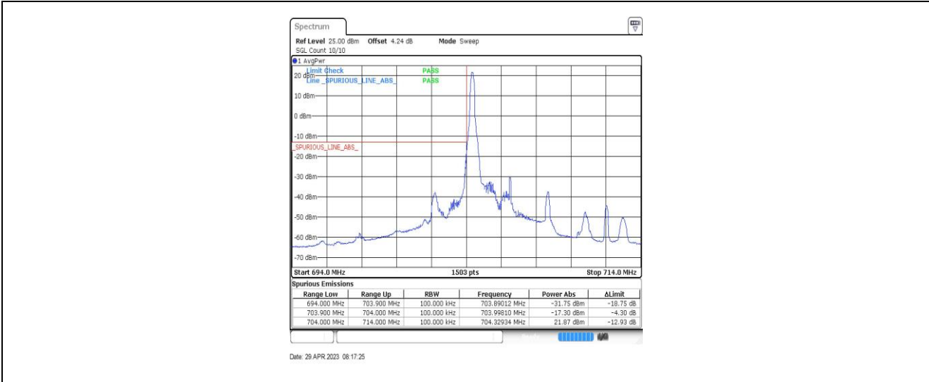
Band17-5MHz-QPSK-23755-1RB#0
