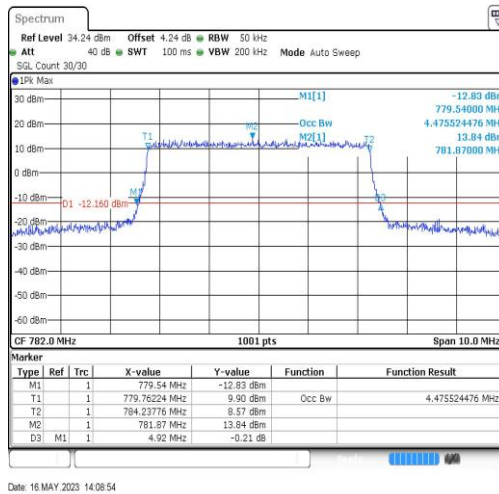
Band13-5MHz-QPSK-23230-25RB#0-4.476
