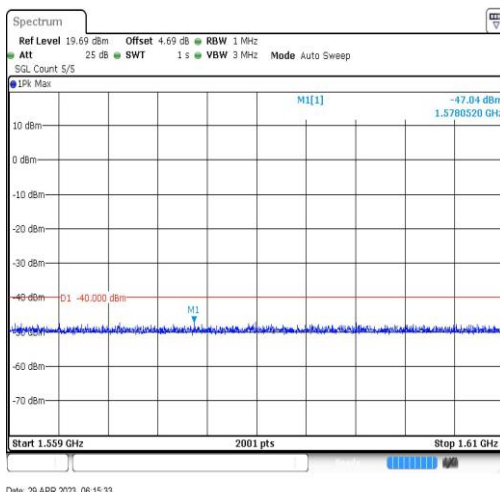
Band13-10MHz-QPSK-23230-1RB#0-Range4:1559~1610MHz
