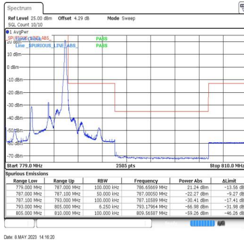
Band13-5MHz-QPSK-23255-1RB#24
