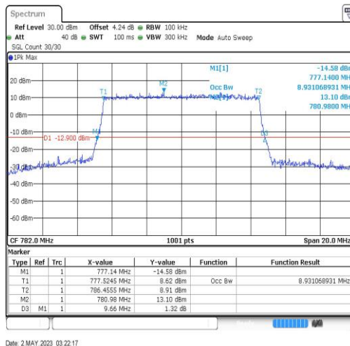
Band13-10MHz-64QAM-23230-50RB#0-8.931
