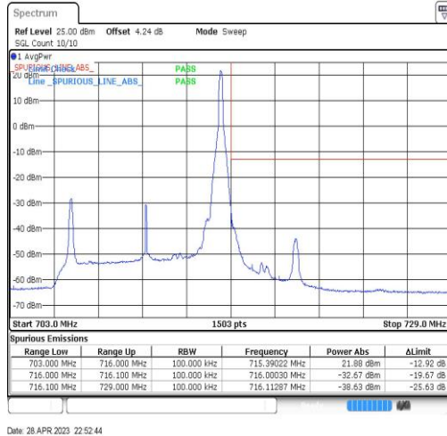
Band12-10MHz-QPSK-23130-1RB#49
