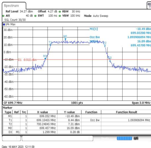
Band12-1.4MHz-64QAM-23017-6RB#0-1.094
