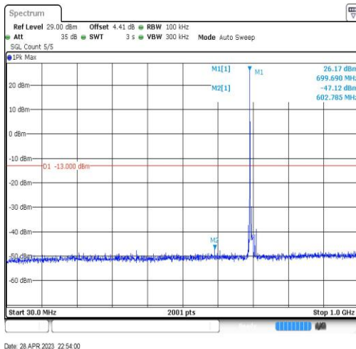
Band12-10MHz-QPSK-23060-1RB#0-Range3:30~1000MHz
