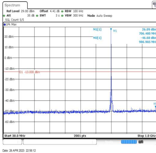
Band12-10MHz-QPSK-23130-1RB#0-Range3:30~1000MHz
