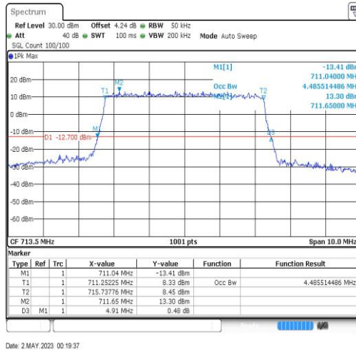
Band12-5MHz-64QAM-23155-25RB#0-4.486
