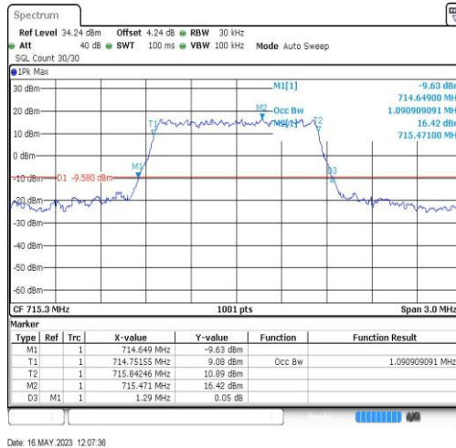
Band12-1.4MHz-QPSK-23173-6RB#0-1.091
