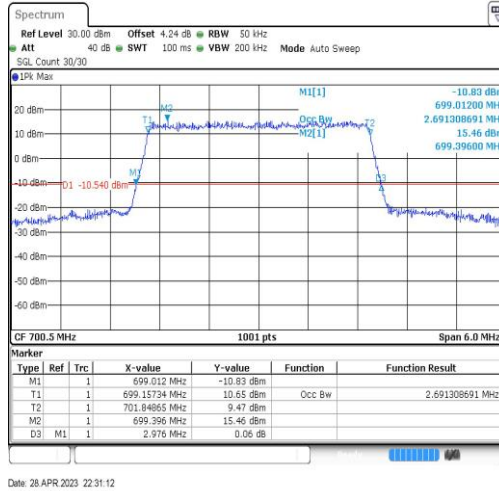
Band12-3MHz-16QAM-23025-15RB#0-2.691
