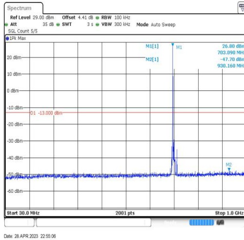
Band12-10MHz-QPSK-23095-1RB#0-Range3:30~1000MHz
