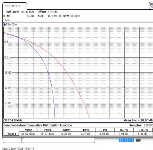
Band12-10MHz-16QAM-23060-50RB#0
