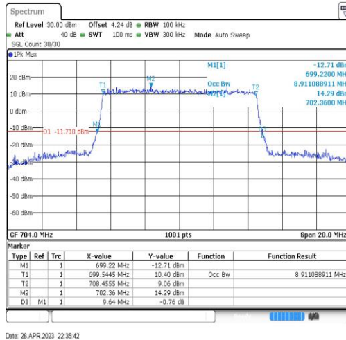
Band12-10MHz-16QAM-23060-50RB#0-8.911
