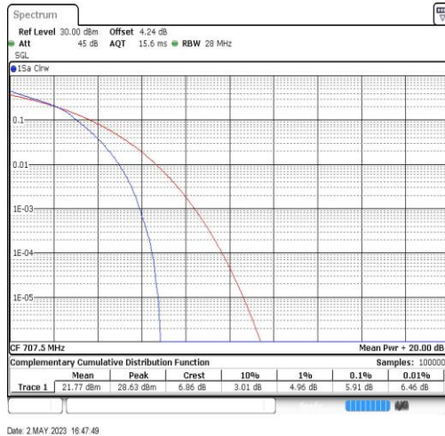
Band12-10MHz-16QAM-23095-50RB#0
