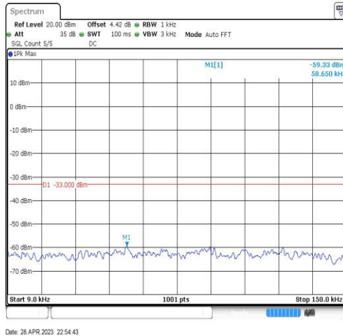
Band12-10MHz-QPSK-23095-1RB#0-Range1:0.009~0.15MHz
