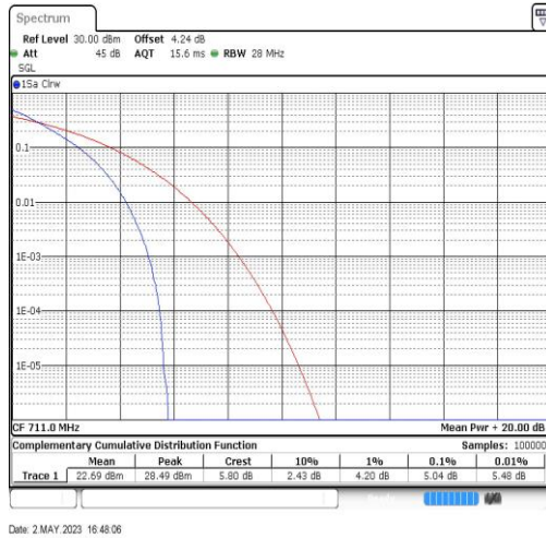
Band12-10MHz-QPSK-23130-50RB#0
