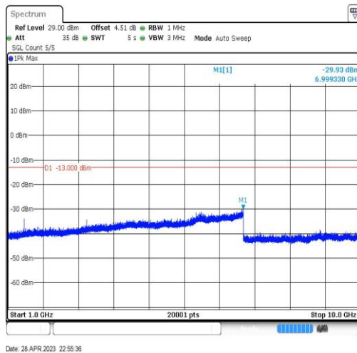
Band12-10MHz-QPSK-23095-1RB#0-Range4:1000~10000MHz
