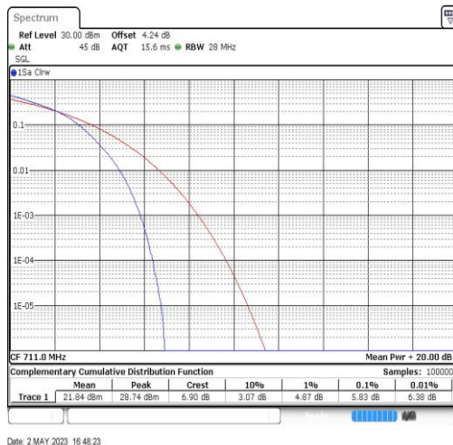
Band12-10MHz-16QAM-23130-50RB#0
