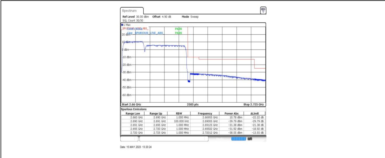
41-41-10MHz-20MHz-QPSK-QPSK-41346-41490-50RB#0-100RB#0
