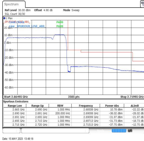
41-41-20MHz-5MHz-QPSK-QPSK-41440-41557-100RB#0-25RB#0
