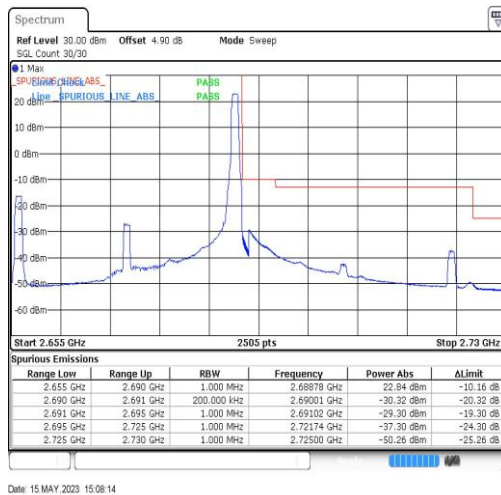
41-41-15MHz-20MHz-QPSK-QPSK-41319-41490-0RB#0-1RB#99
