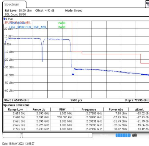
41-41-20MHz-15MHz-QPSK-QPSK-41341-41512-100RB#0-75RB#0
