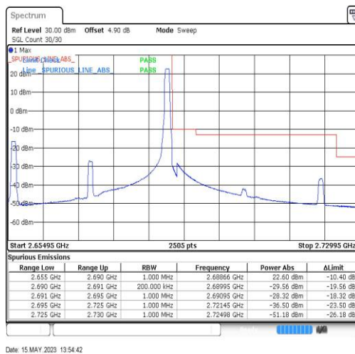
41-41-20MHz-15MHz-QPSK-QPSK-41341-41512-0RB#0-1RB#74
