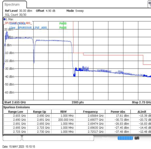
41-41-15MHz-20MHz-QPSK-QPSK-41319-41490-75RB#0-100RB#0
