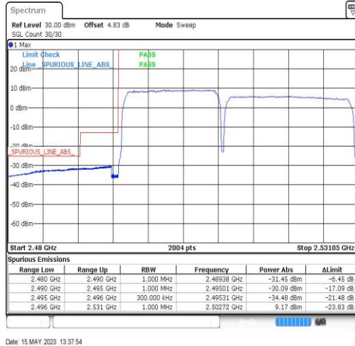
41-41-15MHz-20MHz-QPSK-QPSK-39728-39899-75RB#0-100RB#0
