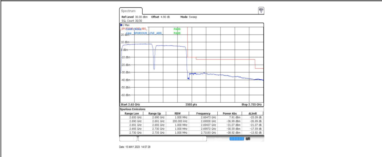
41-41-20MHz-20MHz-QPSK-QPSK-41292-41490-100RB#0-100RB#0
