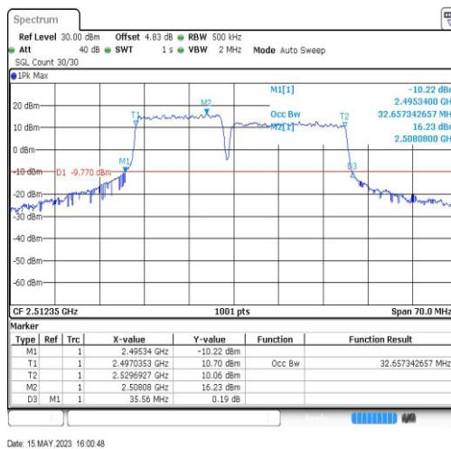
41-41-15MHz-20MHz-QPSK-QPSK-39728-39899-75RB#0-100RB#0-32.657
