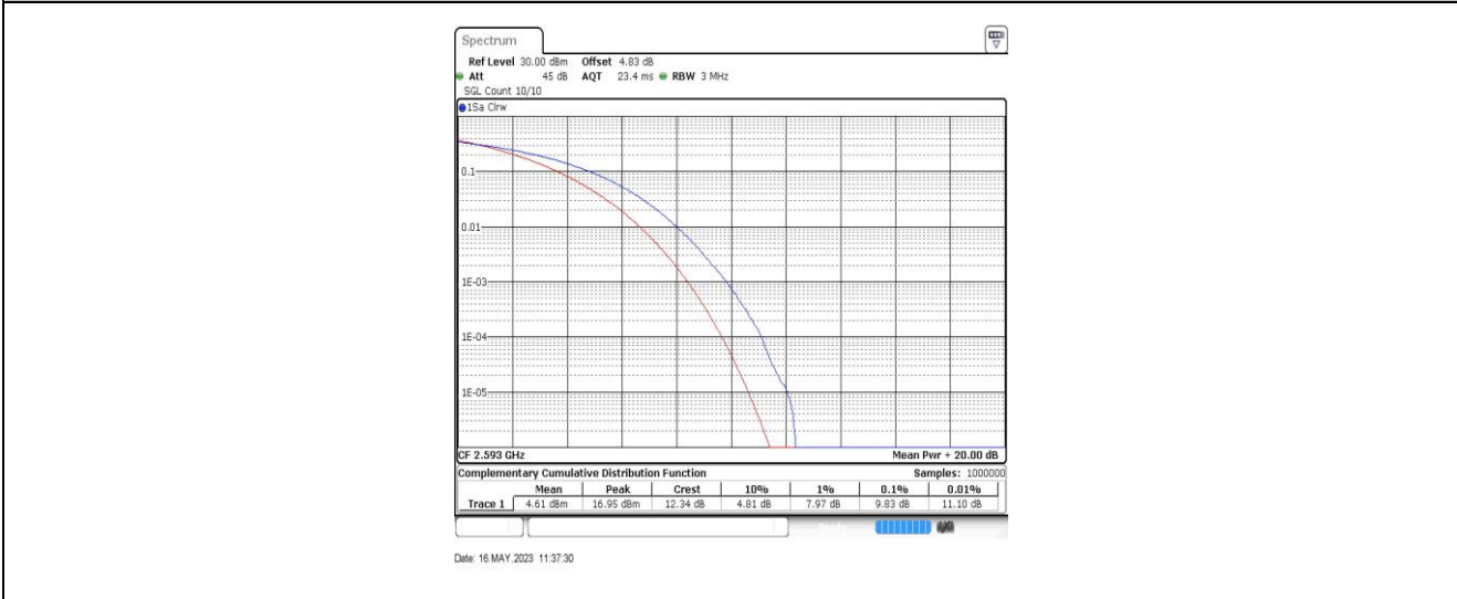
41-41-20MHz-20MHz-QPSK-QPSK-40521-40719-100RB#0-100RB#0
