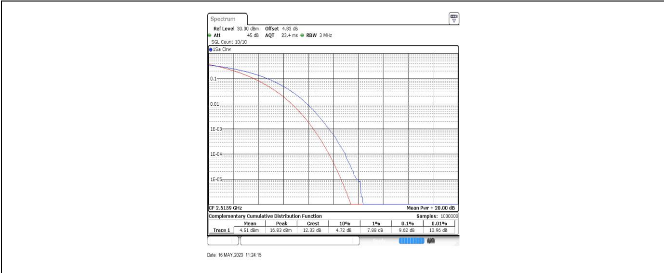
41-41-20MHz-20MHz-QPSK-QPSK-39750-39948-100RB#0-100RB#0
