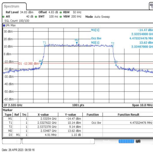
Band7-5MHz-QPSK-21100-25RB#0-4.476
