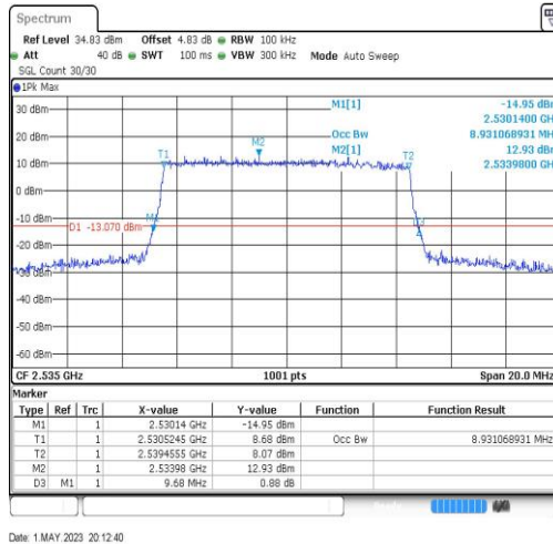
Band7-10MHz-64QAM-21100-50RB#0-8.931
