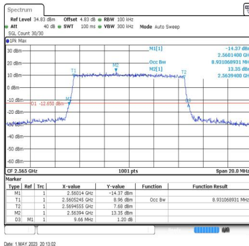
Band7-10MHz-64QAM-21400-50RB#0-8.931
