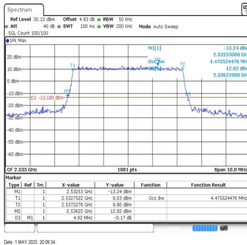
Band7-5MHz-64QAM-21100-25RB#0-4.476
