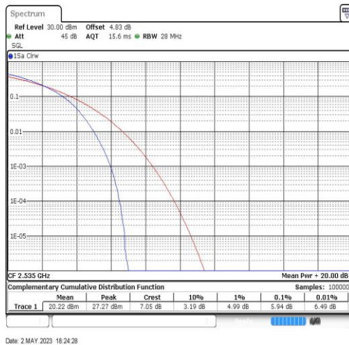
Band7-20MHz-64QAM-21100-100RB#0
