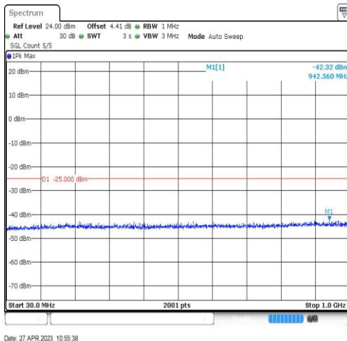
Band7-20MHz-QPSK-20850-1RB#0-Range3:30~1000MHz
