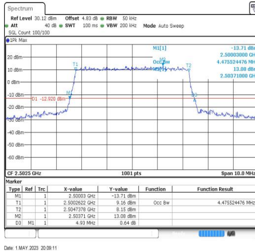
Band7-5MHz-64QAM-20775-25RB#0-4.476
