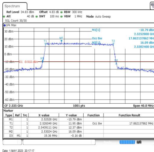
Band7-20MHz-64QAM-21100-100RB#0-17.862
