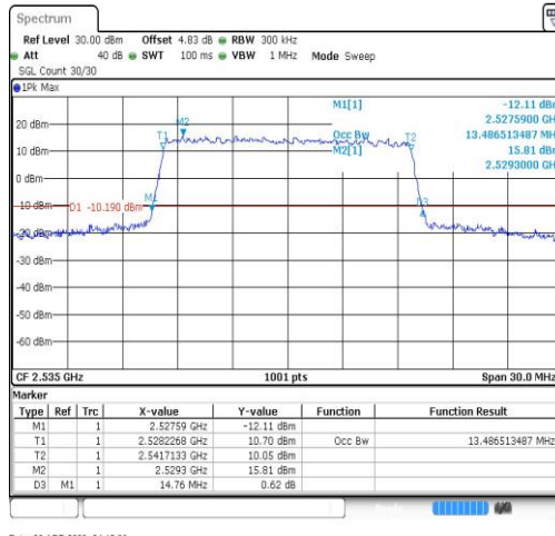
Band7-15MHz-16QAM-21100-75RB#0-13.487
