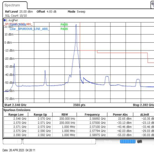
Band7-20MHz-QPSK-21350-1RB#99
