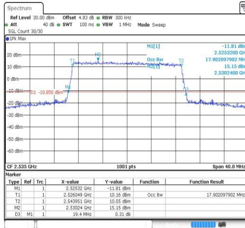
Band7-20MHz-16QAM-21100-100RB#0-17.902
