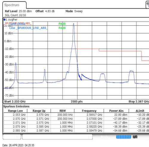
Band7-15MHz-QPSK-21375-1RB#74
