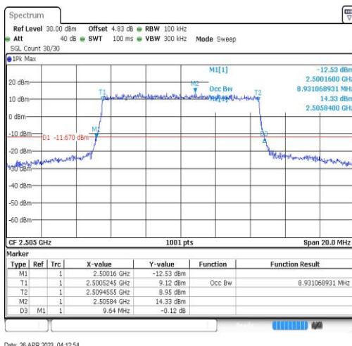
Band7-10MHz-QPSK-20800-50RB#0-8.931
