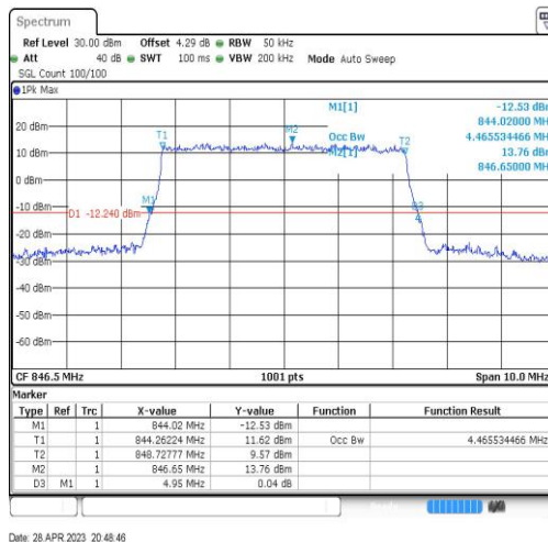
Band5-5MHz-16QAM-20625-25RB#0-4.466
