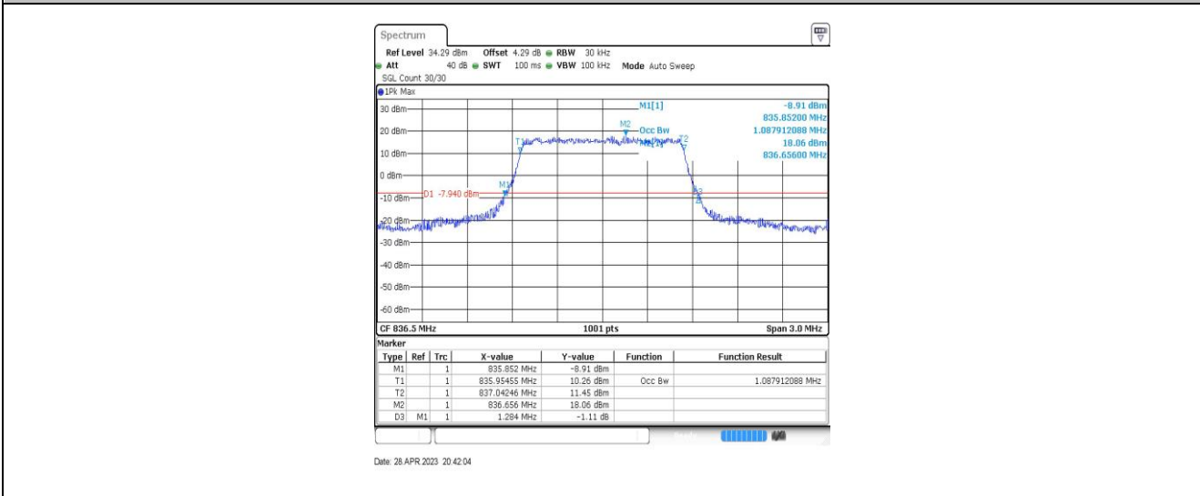
Band5-1.4MHz-QPSK-20525-6RB#0-1.088
