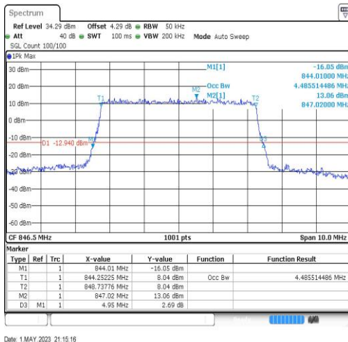
Band5-5MHz-64QAM-20625-25RB#0-4.486
