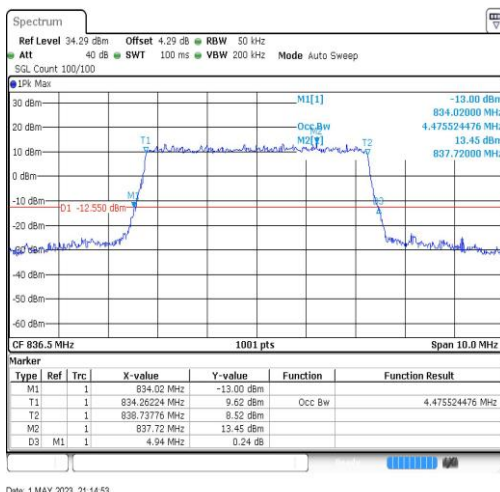
Band5-5MHz-64QAM-20525-25RB#0-4.476
