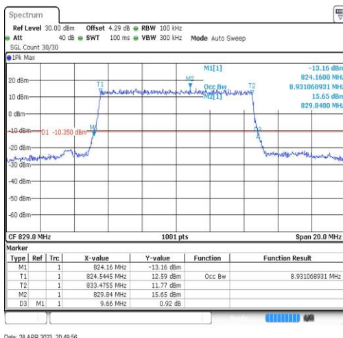
Band5-10MHz-QPSK-20450-50RB#0-8.931
