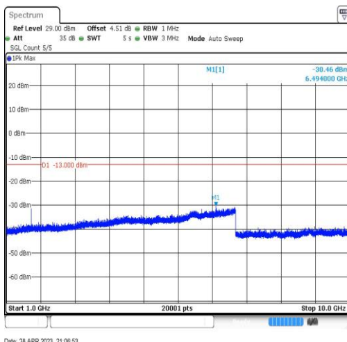
Band5-10MHz-QPSK-20450-1RB#0-Range4:1000~10000MHz
