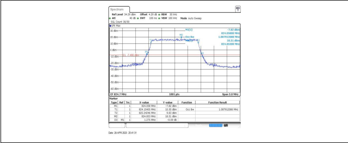
Band5-1.4MHz-QPSK-20407-6RB#0-1.088
