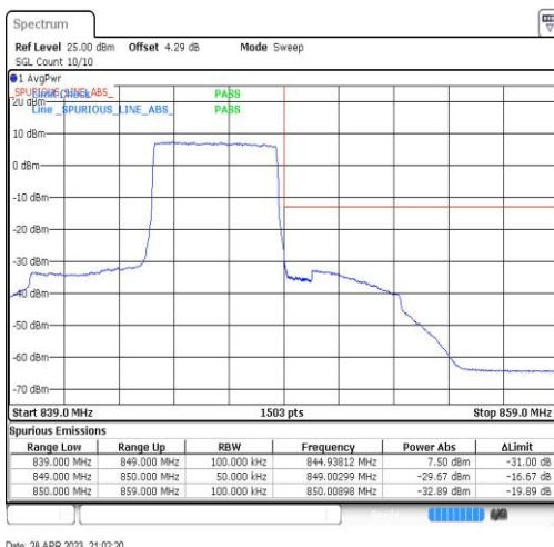
Band5-5MHz-QPSK-20625-25RB#0
