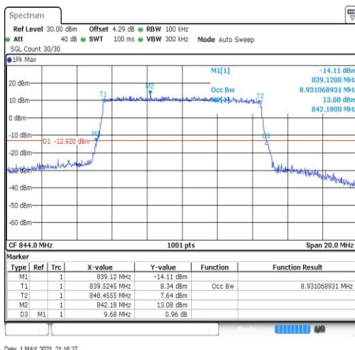
Band5-10MHz-64QAM-20600-50RB#0-8.931
