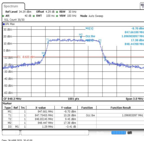
Band5-1.4MHz-16QAM-20643-6RB#0-1.097
