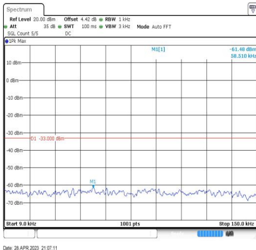
Band5-10MHz-QPSK-20525-1RB#0-Range1:0.009~0.15MHz
