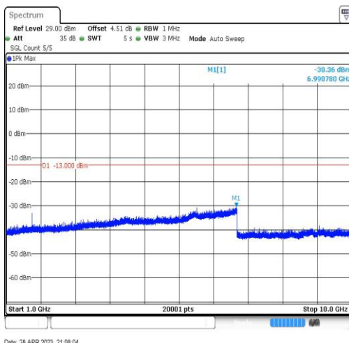
Band5-10MHz-QPSK-20525-1RB#0-Range4:1000~10000MHz
