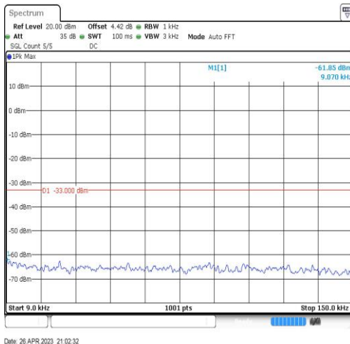
Band4-20MHz-QPSK-20300-1RB#0-Range1:0.009~0.15MHz
