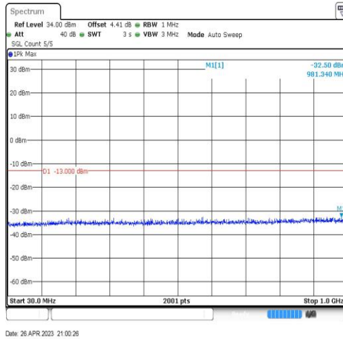
Band4-20MHz-QPSK-20050-1RB#0-Range3:30~1000MHz
