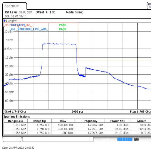
Band4-5MHz-QPSK-20375-25RB#0
