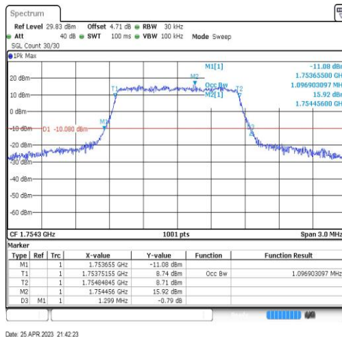
Band4-1.4MHz-16QAM-20393-6RB#0-1.097
