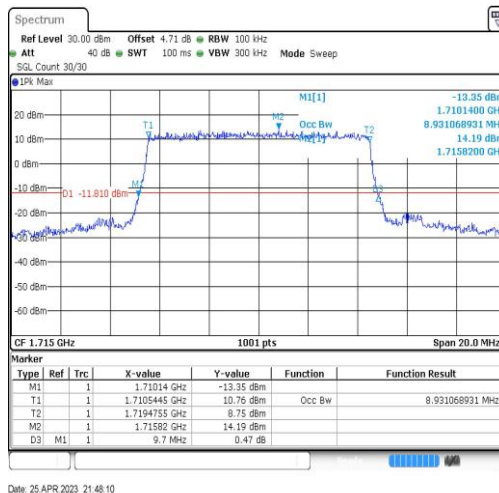
Band4-10MHz-QPSK-20000-50RB#0-8.931
