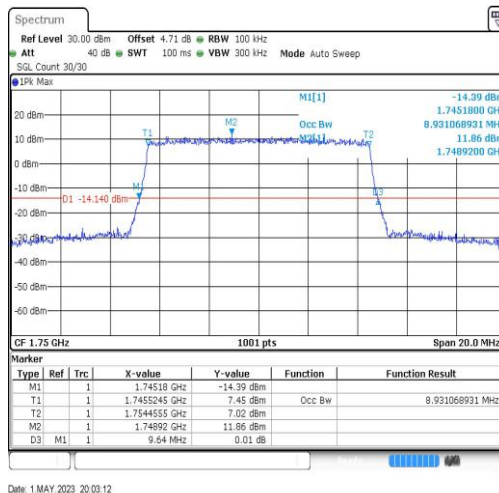
Band4-10MHz-64QAM-20350-50RB#0-8.931
