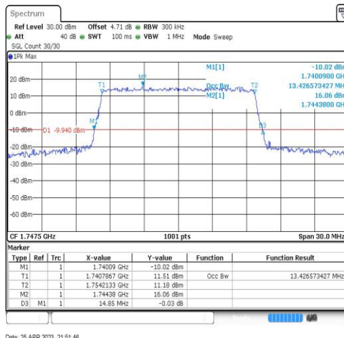
Band4-15MHz-16QAM-20325-75RB#0-13.427
