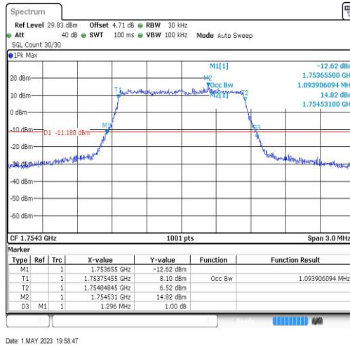
Band4-1.4MHz-64QAM-20393-6RB#0-1.094
