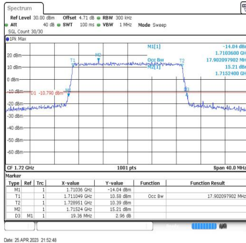
Band4-20MHz-16QAM-20050-100RB#0-17.902
