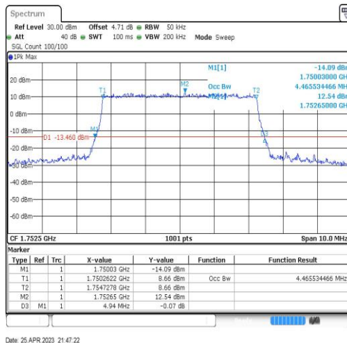
Band4-5MHz-16QAM-20375-25RB#0-4.466
