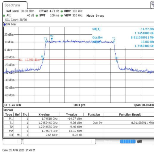
Band4-10MHz-16QAM-20350-50RB#0-8.911
