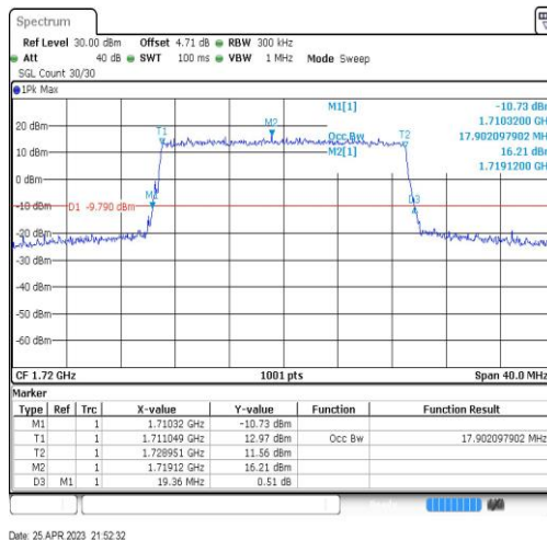
Band4-20MHz-QPSK-20050-100RB#0-17.902
