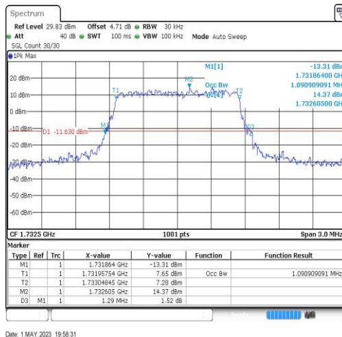
Band4-1.4MHz-64QAM-20175-6RB#0-1.091
