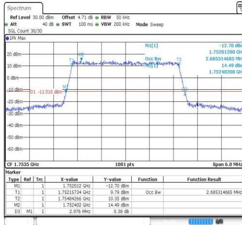
Band4-3MHz-16QAM-20385-15RB#0-2.685
