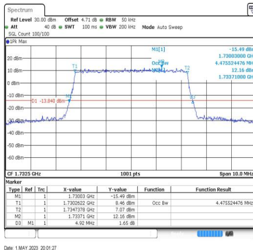
Band4-5MHz-64QAM-20175-25RB#0-4.476
