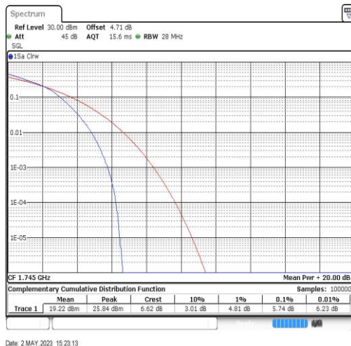
Band4-20MHz-16QAM-20300-100RB#0
