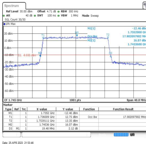
Band4-20MHz-QPSK-20300-100RB#0-17.902
