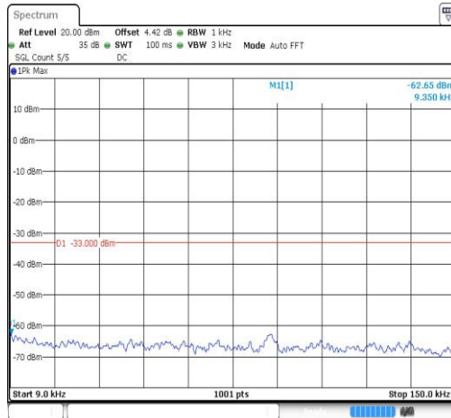
Band2-20MHz-QPSK-19100-1RB#0-Range1:0.009~0.15MHz
