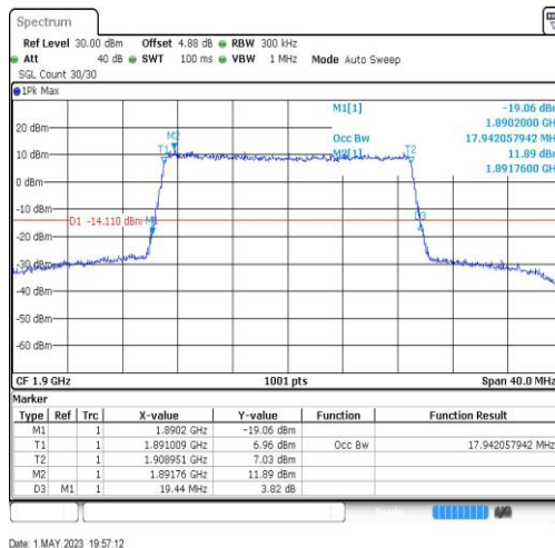
Band2-20MHz-64QAM-19100-100RB#0-17.942
