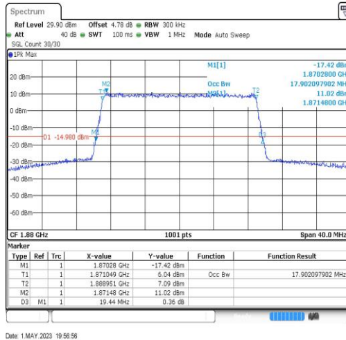
Band2-20MHz-64QAM-18900-100RB#0-17.902
