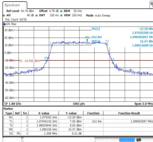
Band2-1.4MHz-16QAM-18900-6RB#0-1.097
