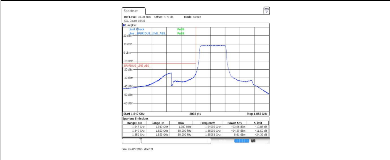
Band2-1.4MHz-QPSK-18607-6RB#0
