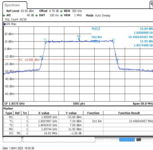
Band2-15MHz-64QAM-18675-75RB#0-13.457
