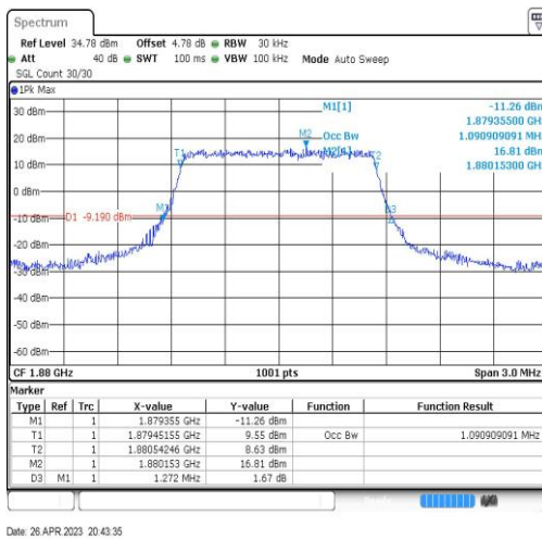
Band2-1.4MHz-QPSK-18900-6RB#0-1.091
