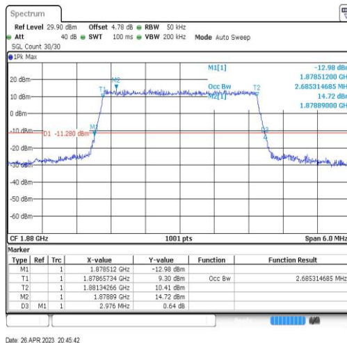
Band2-3MHz-16QAM-18900-15RB#0-2.685
