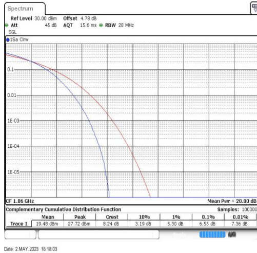
Band2-20MHz-64QAM-18700-100RB#0
