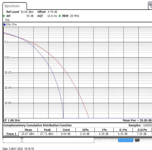
Band2-20MHz-64QAM-18900-100RB#0
