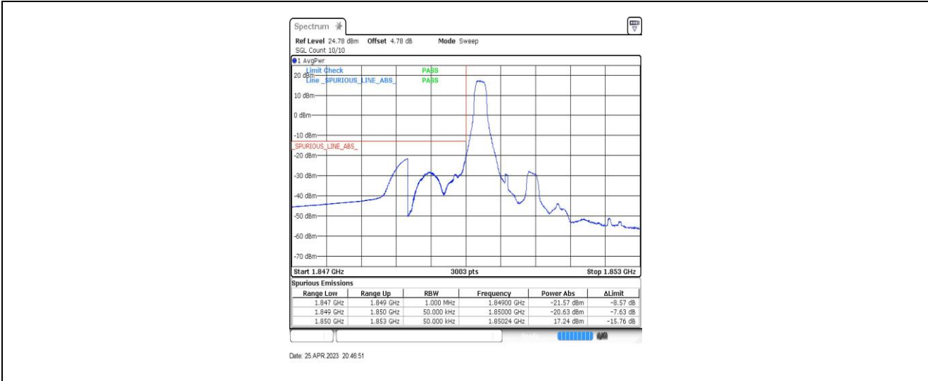
Band2-1.4MHz-QPSK-18607-1RB#0
