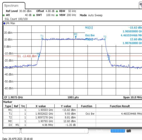
Band2-5MHz-16QAM-19175-25RB#0-4.466
