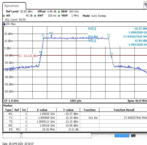
Band2-20MHz-QPSK-19100-100RB#0-17.942
