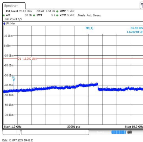
BandV-4182-1000~10000MHz-1670.24
