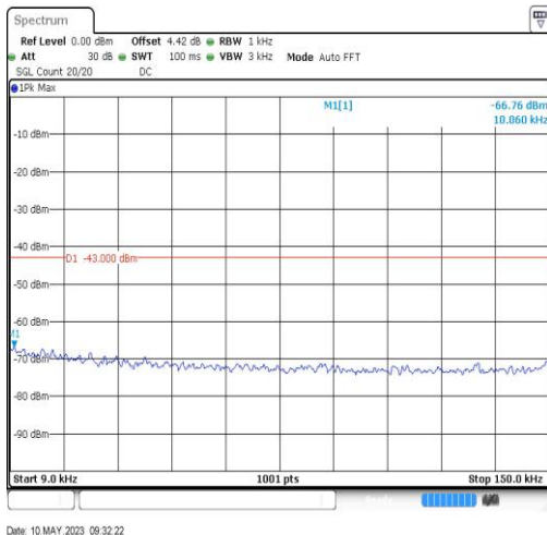
BandII-9400-0.009~0.15MHz-0.01
