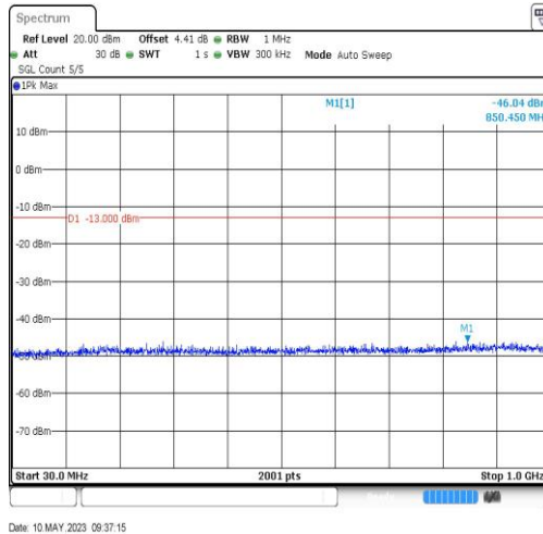
BandIV-1413-30~1000MHz-850.45
