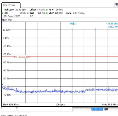
BandIV-1513-0.15~30MHz-0.17
