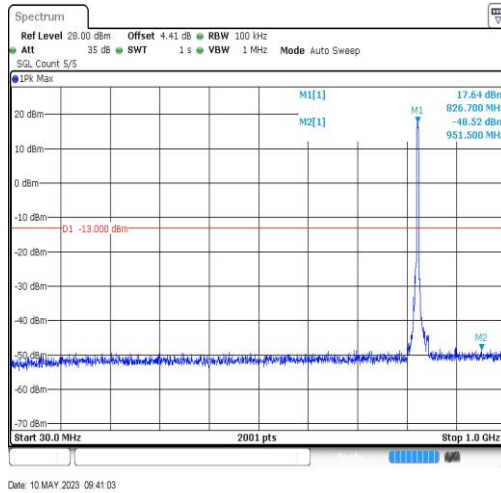
BandV-4132-30~1000MHz-951.5
