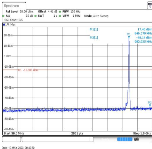
BandV-4233-30~1000MHz-983.03
