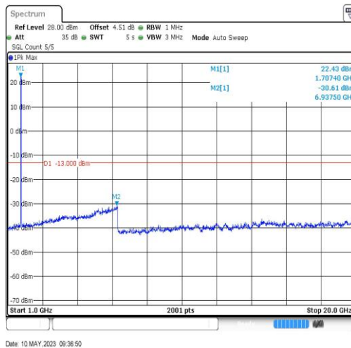
BandIV-1312-1000~20000MHz-6937.5
