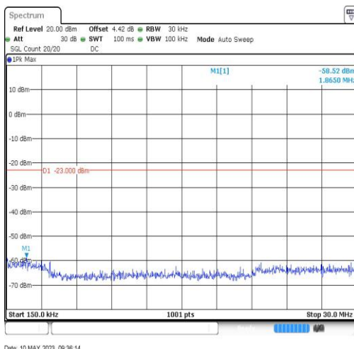
BandIV-1312-0.15~30MHz-1.87
