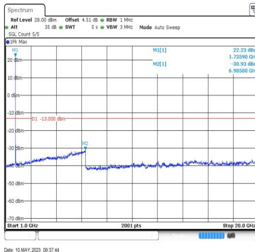
BandIV-1413-1000~20000MHz-6985
