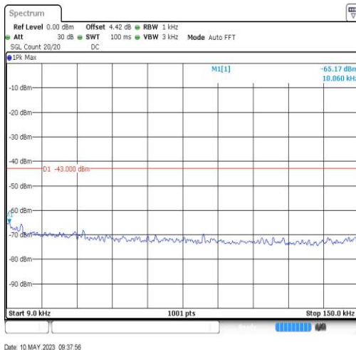
BandIV-1513-0.009~0.15MHz-0.01
