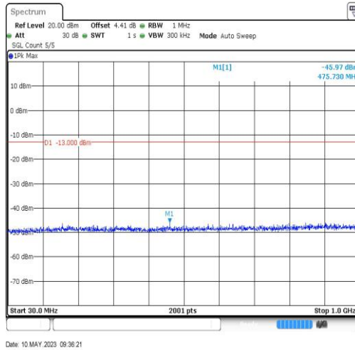
BandIV-1312-30~1000MHz-475.73
