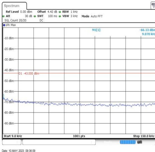
BandIV-1312-0.009~0.15MHz-0.01
