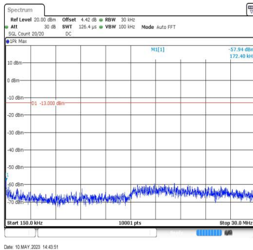
EGPRS850-128-8-0.15~30MHz-0.17
