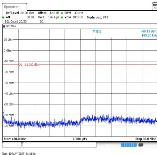
EGPRS850-190-8-0.15~30MHz-0.19
