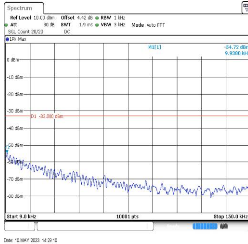
GSM850-190-5-0.009~0.15MHz-0.01
