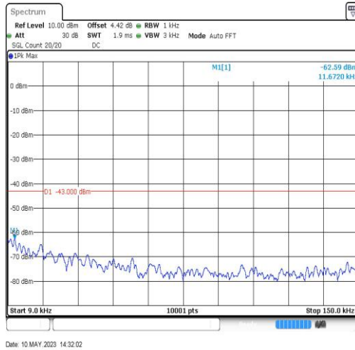
GSM1900-512-0-0.009~0.15MHz-0.01
