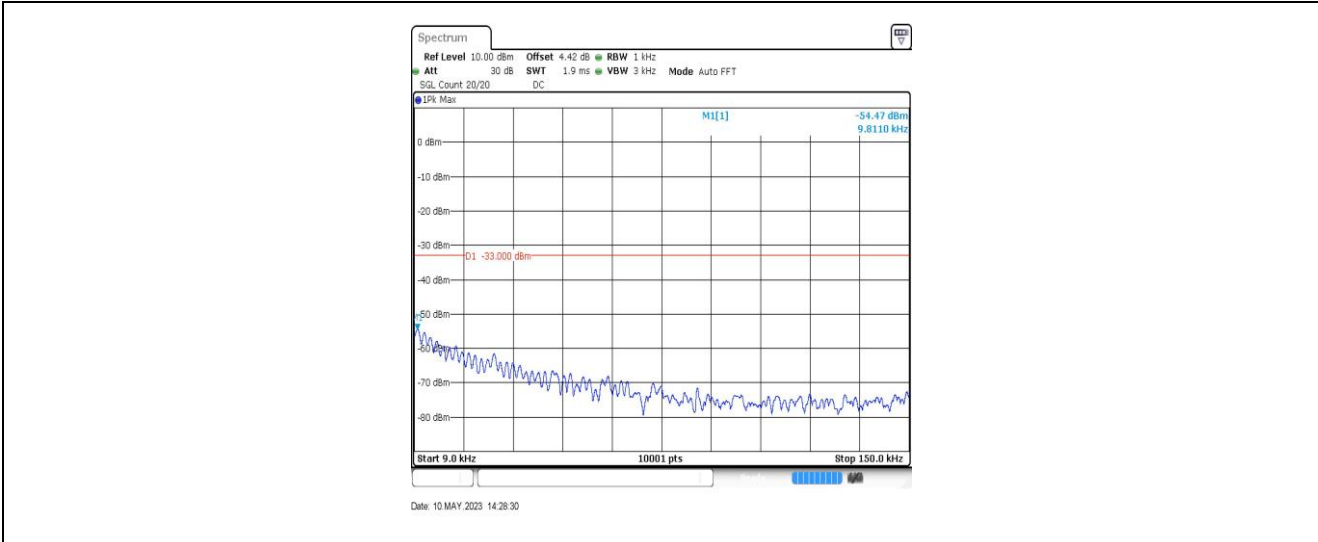
GSM850-128-5-0.009~0.15MHz-0.01
