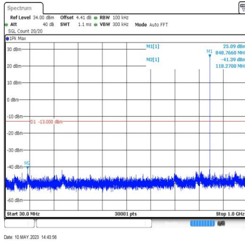
EGPRS850-128-8-30~1000MHz-118.27
