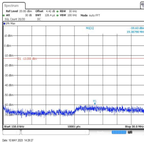
GSM850-251-5-0.15~30MHz-19.39
