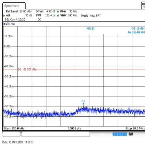
EGPRS1900-512-2-0.15~30MHz-16.86
