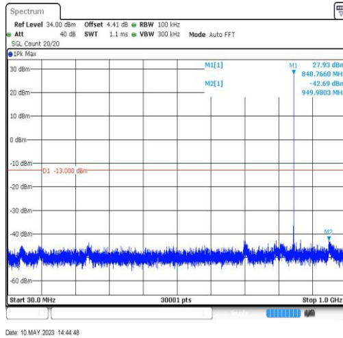
EGPRS850-251-8-30~1000MHz-949.98
