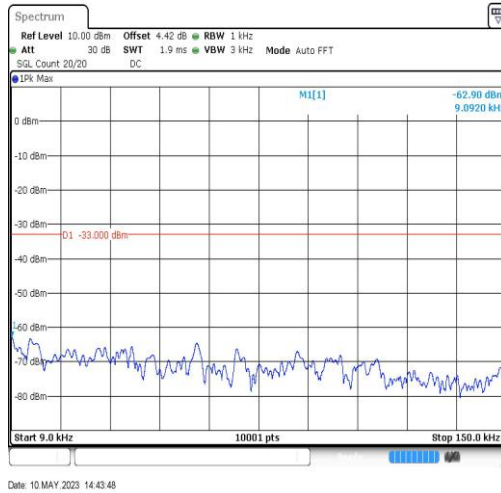
EGPRS850-128-8-0.009~0.15MHz-0.01
