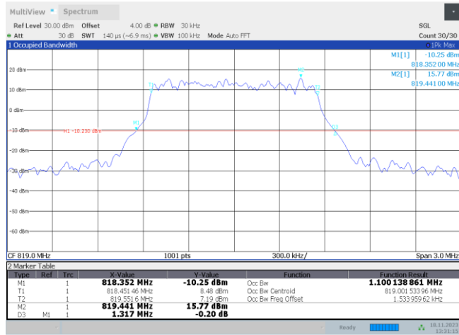
Band26-1.4MHz-16QAM-26740-6RB#0
