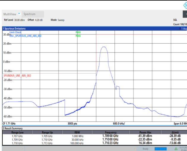
Band4-1.4MHz-QPSK-19957-1RB#0
