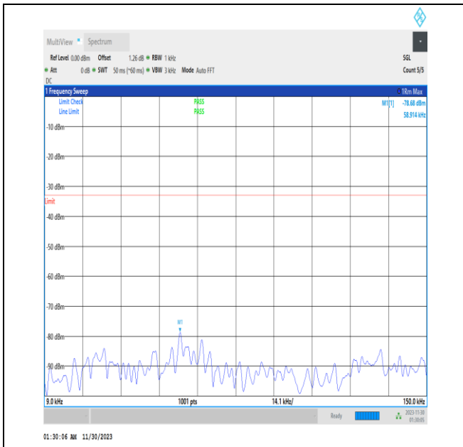
NTVN_N26-824-849_PC3_15_20_H_TID1_0.009_0.15_#1
