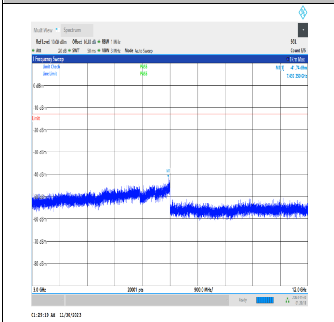
NTVN_N26-824-849_PC3_15_20_M_TID1_3000_12000_#1
