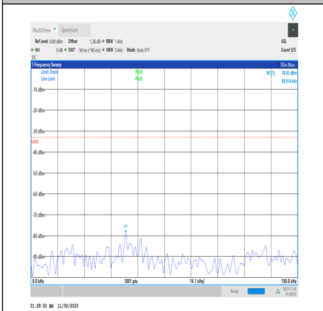
NTVN_N26-824-849_PC3_15_20_M_TID1_0.009_0.15_#
