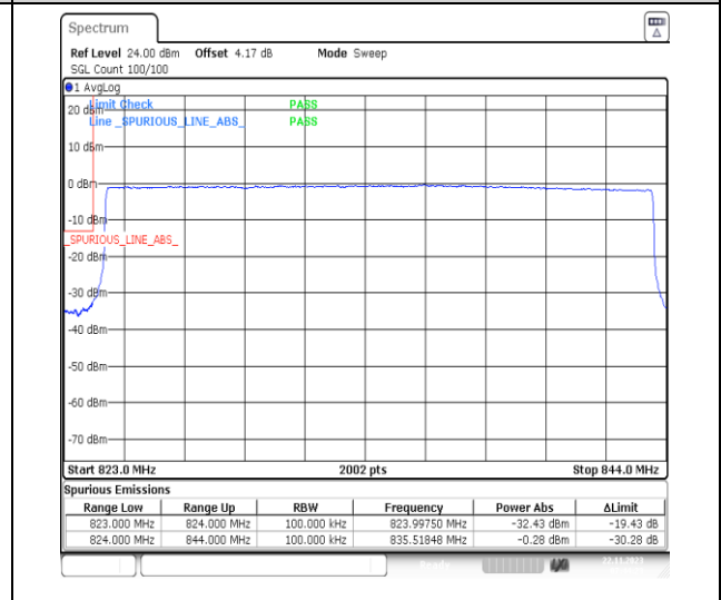
1-N26-824-849-PC3-15-20-L-6-CP-QPSK-Outer_Full-106@0-Ant41-1-seegraph-PASS-see graph
