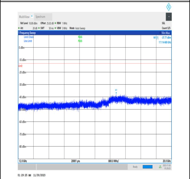
NTVN_N26-824-849_PC3_15_20_M_TID1_12000_20000_#1
