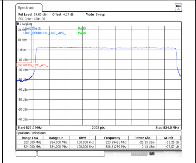
1-N26-824-849-PC3-15-10-L-6-CP-QPSK-Outer_Full-52@0-Ant41-1-seegraph-PASS-see graph
