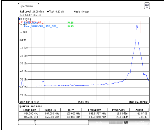
1-N26-824-849-PC3-15-15-H-5-CP-QPSK-Edge_1RB_Right-1@78-Ant41-1-seegraph-PASS-see graph
