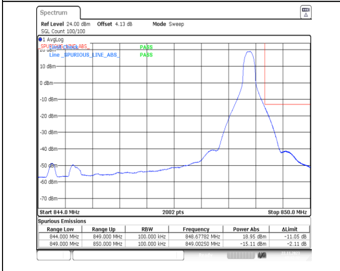
1-N26-824-849-PC3-15-5-H-5-CP-QPSK-Edge_1RB_Right-1@24-Ant41-1-seegraph-PASS-see graph
