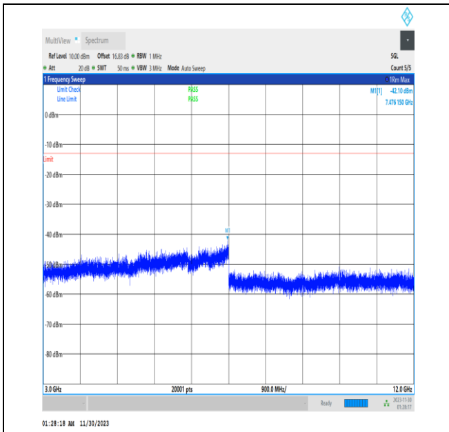
NTVN_N26-824-849_PC3_15_20_L_TID1_3000_12000_
