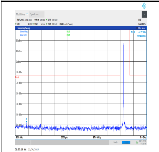
NTVN_N26-824-849_PC3_15_20_H_TID1_30_1000_#1
