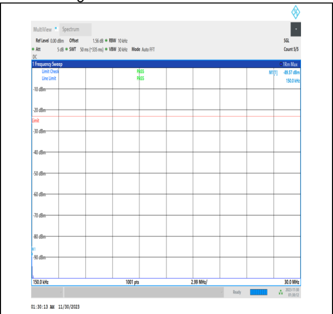
NTVN_N26-824-849_PC3_15_20_H_TID1_0.15_30_#1
