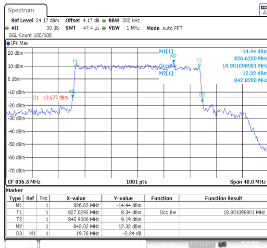
1-N26-824-849-PC3-15-20-M-7-CP-16QAM-Outer_F ull-106@0-Ant41-18.901-19.760-≤20-PASS
