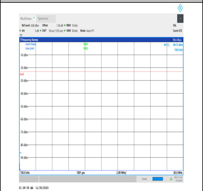
NTVN_N26-824-849_PC3_15_20_M_TID1_0.15_30_#1
