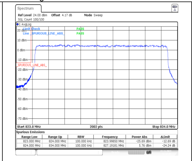
1-N26-824-849-PC3-15-10-L-3-DFT-PI2BPSK-Outer_Full-50@0-Ant41-1-seegraph-PASS-see graph
