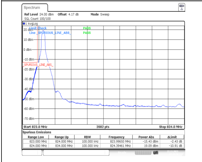
1-N26-824-849-PC3-15-10-L-4-CP-QPSK-Edge_1RB_Left-1@0-Ant41-1-seegraph-PASS-see graph
