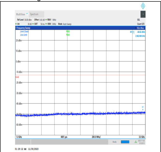
NTVN_N26-824-849_PC3_15_20_M_TID1_1000_3000_#1
