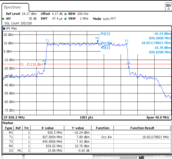
1-N26-824-849-PC3-15-20-M-8-CP-64QAM-Outer_F ull-106@0-Ant41-18.821-19.880-≤20-PASS
