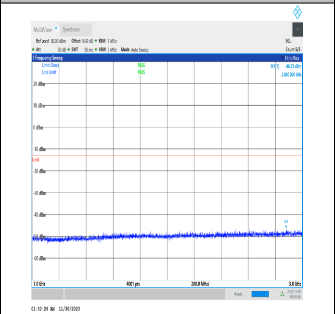
NTVN_N26-824-849_PC3_15_20_H_TID1_1000_3000_#1
