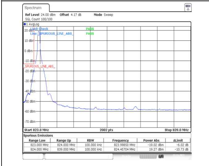
1-N26-824-849-PC3-15-15-L-4-CP-QPSK-Edge_1RB_Left-1@0-Ant41-1-seegraph-PASS-see graph
