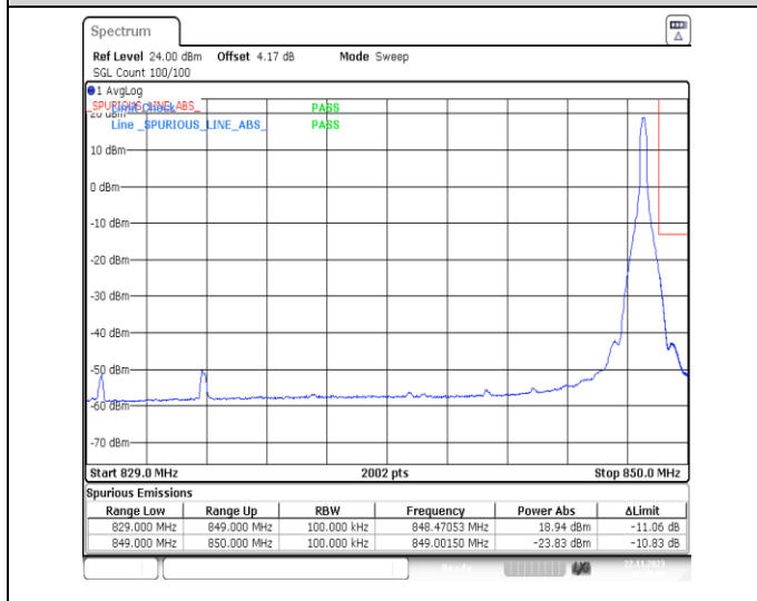
1-N26-824-849-PC3-15-20-H-5-CP-QPSK-Edge_1RB_Right-1@105-Ant41-1-seegraph-PASS-see graph
