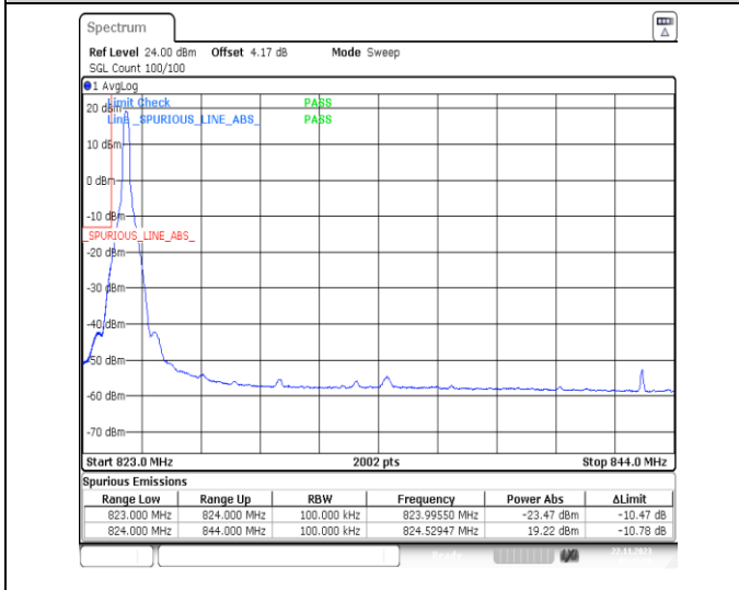
1-N26-824-849-PC3-15-20-L-4-CP-QPSK-Edge_1RB_Left-1@0-Ant41-1-seegraph-PASS-see graph
