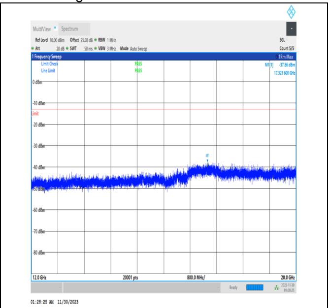
NTVN_N26-824-849_PC3_15_20_L_TID1_12000_20000_
