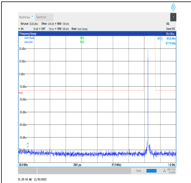
NTVN_N26-824-849_PC3_15_20_M_TID1_30_1000_#1
