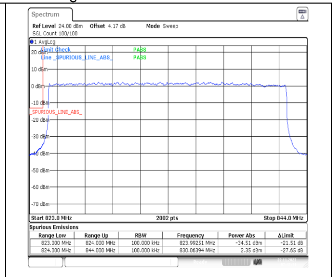
1-N26-824-849-PC3-15-20-L-3-DFT-PI2BPSK-Outer_Full-100@0-Ant41-1-seegraph-PASS-see graph
