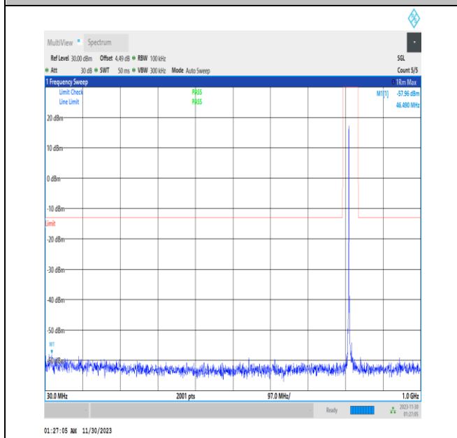
NTVN_N26-814-824_PC3_15_10_H_TID1_30_1000_#1
