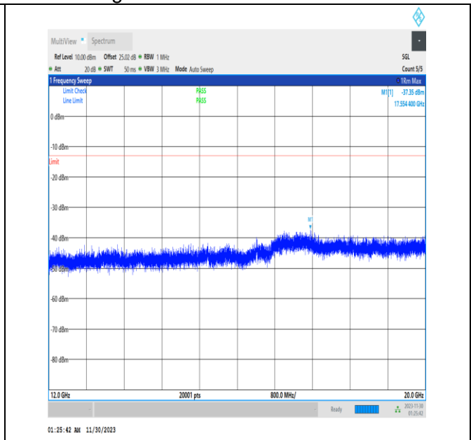
NTVN_N26-814-824_PC3_15_10_L_TID1_12000_20000_
