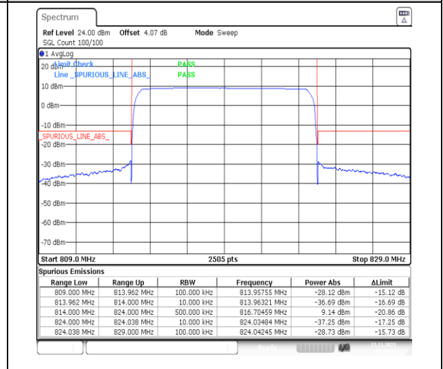
1-N26-814-824-PC3-15-10-H-6-CP-QPSK-Outer_Full-52@0-Ant41-1--PASS-see graph
