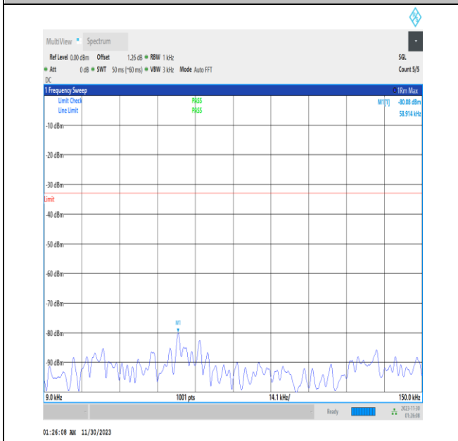
NTVN_N26-814-824_PC3_15_10_M_TID1_0.009_0.15_#
