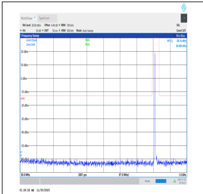
NTVN_N26-814-824_PC3_15_10_M_TID1_30_1000_#1
