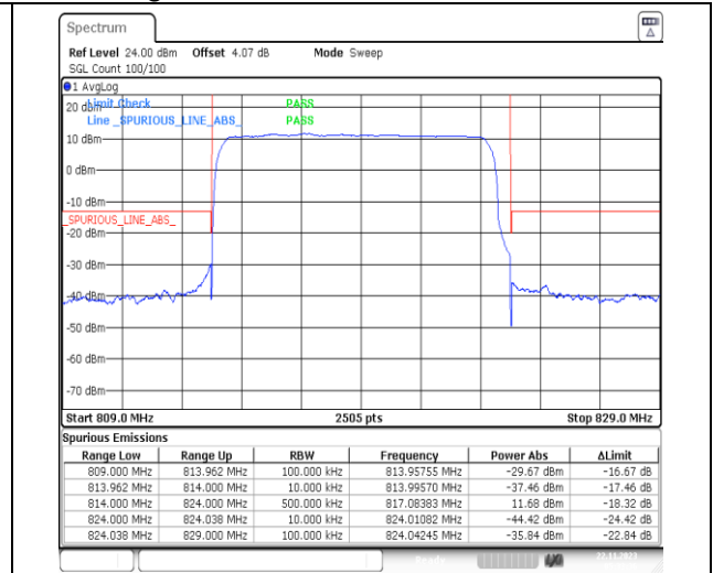
1-N26-814-824-PC3-15-10-H-3-DFT-PI2BPSK-Out er_Full-50@0-Ant41-1--PASS-see graph
