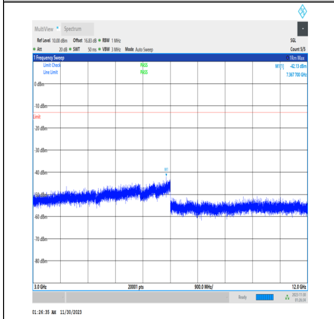
NTVN_N26-814-824_PC3_15_10_M_TID1_3000_12000_#1
