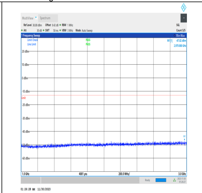
NTVN_N26-814-824_PC3_15_10_M_TID1_1000_3000_#1
