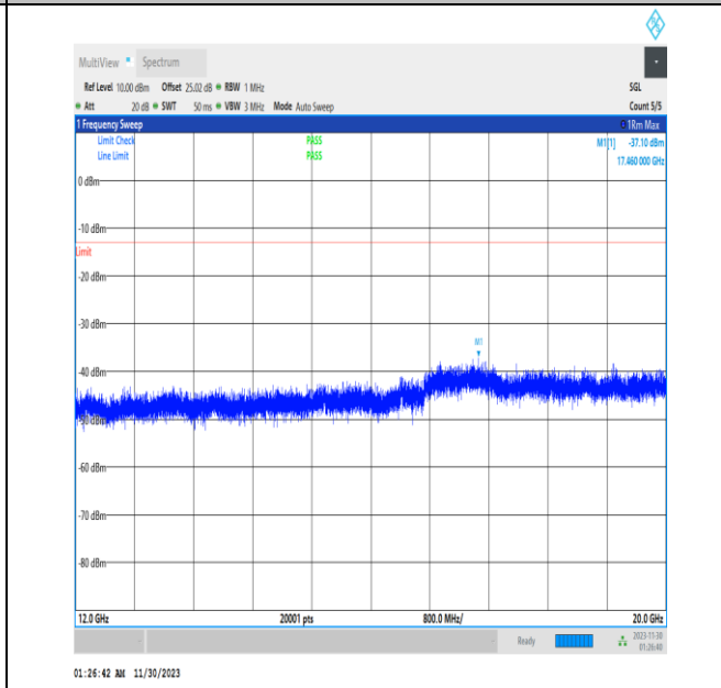
NTVN_N26-814-824_PC3_15_10_M_TID1_12000_20000_#1
