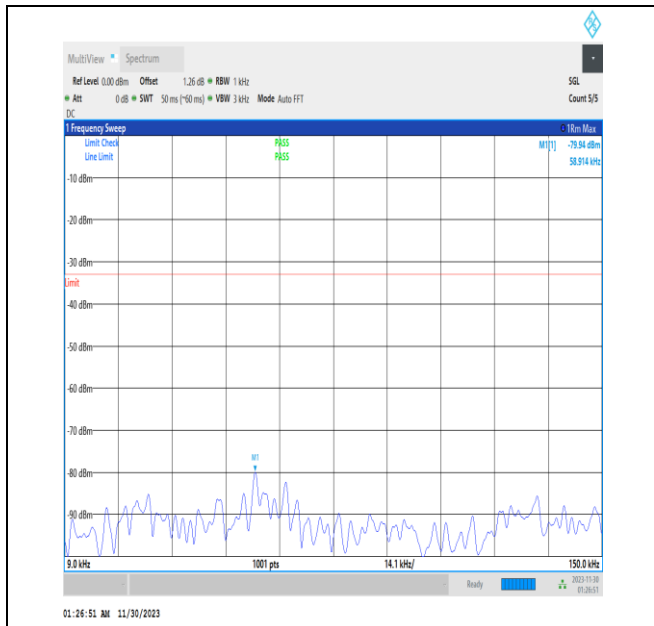
NTVN_N26-814-824_PC3_15_10_H_TID1_0.009_0.15_#1
