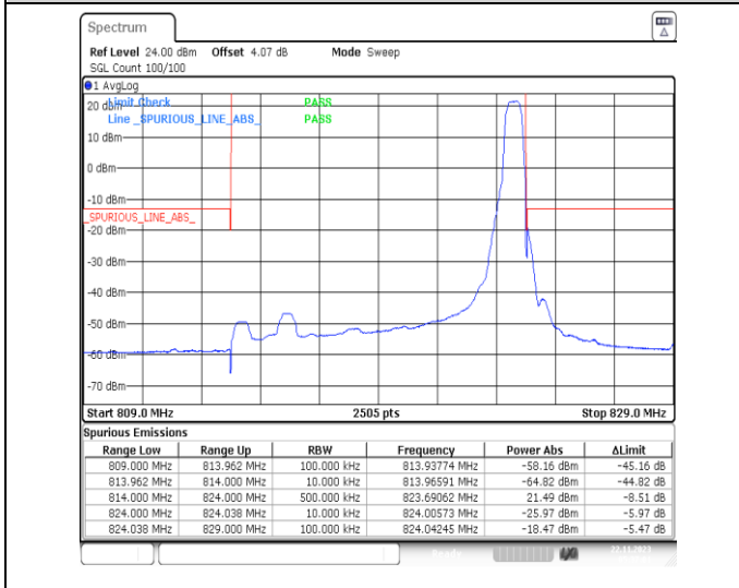
1-N26-814-824-PC3-15-10-H-5-CP-QPSK-Edge_1RB_Right-1@51-Ant41-1--PASS-see graph
