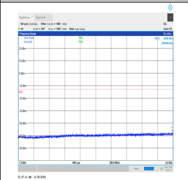
NTVN_N26-814-824_PC3_15_10_H_TID1_1000_3000_#1
