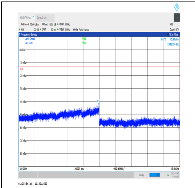
NTVN_N26-814-824_PC3_15_10_L_TID1_3000_12000_
