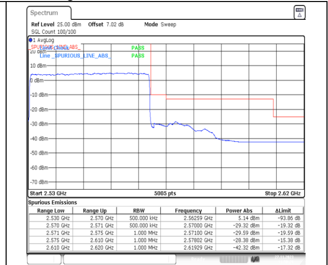
1-N7-PC3-15-40-H-3-DFT-PI2BPSK-Outer_Full-216@0-Ant31-1--PASS-see graph
