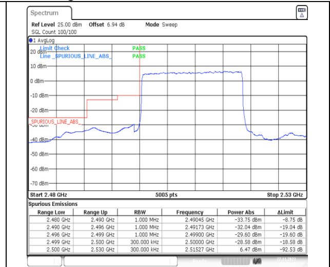
1-N7-PC3-15-20-L-3-DFT-PI2BPSK-Outer_Full-10 0@0-Ant31-1--PASS-see graph
