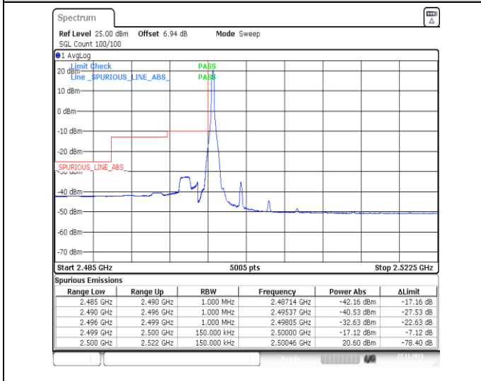
1-N7-PC3-15-15-L-4-CP-QPSK-Edge_1RB_Left-1 @0-Ant31-1--PASS-see graph
