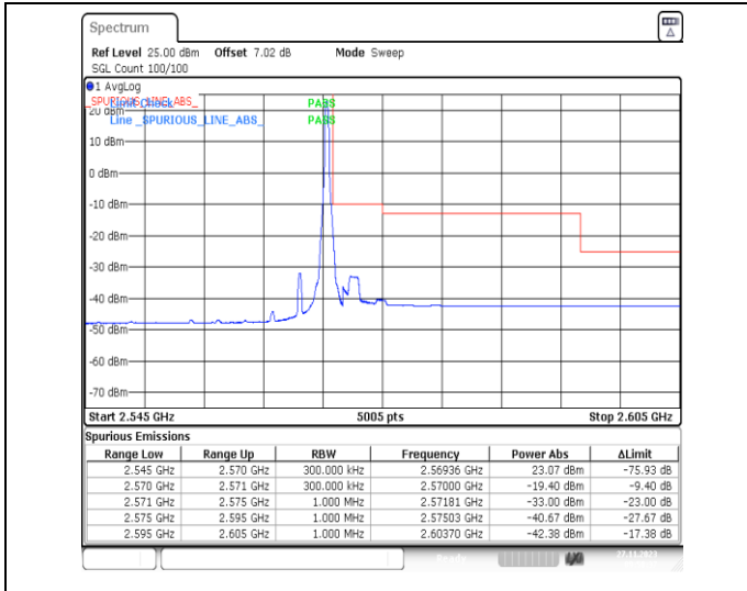
1-N7-PC3-15-25-H-2-DFT-PI2BPSK-Edge_1RB_Right-1@132-Ant31-1--PASS-see graph
