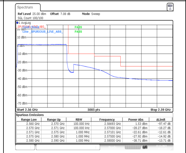
1-N7-PC3-15-10-H-6-CP-QPSK-Outer_Full-52@0-Ant31-1--PASS-see graph
