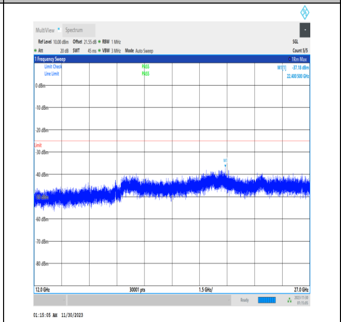
NTVN_N7_PC3_15_40_M_TID1_12000_27000_#1
