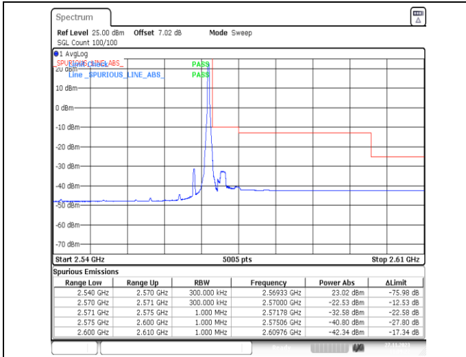
1-N7-PC3-15-30-H-2-DFT-PI2BPSK-Edge_1RB_Right-1@159-Ant31-1--PASS-see graph
