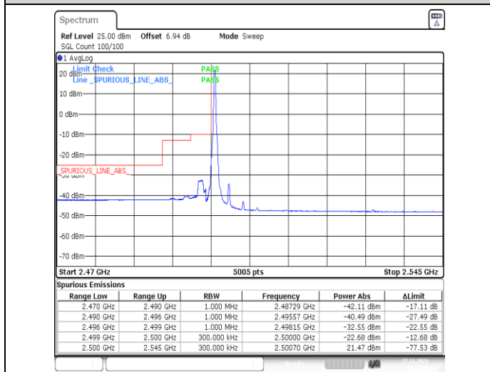
1-N7-PC3-15-30-L-4-CP-QPSK-Edge_1RB_Left-1 @0-Ant31-1--PASS-see graph
