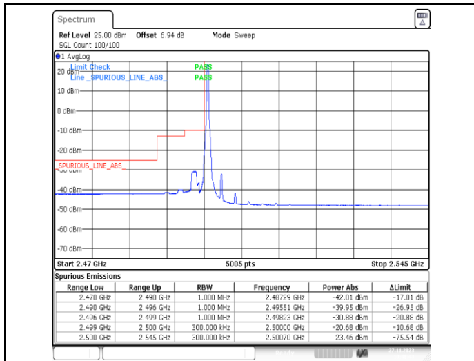
1-N7-PC3-15-30-L-1-DFT-PI2BPSK-Edge_1RB_Left-1 @0-Ant31-1--PASS-see graph
