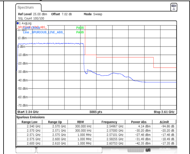
1-N7-PC3-15-30-H-3-DFT-PI2BPSK-Outer_Full-160@0-Ant31-1--PASS-see graph
