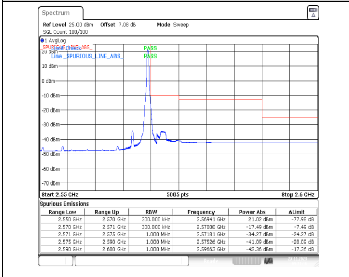
1-N7-PC3-15-20-H-5-CP-QPSK-Edge_1RB_Right-1@105-Ant31-1--PASS-see graph
