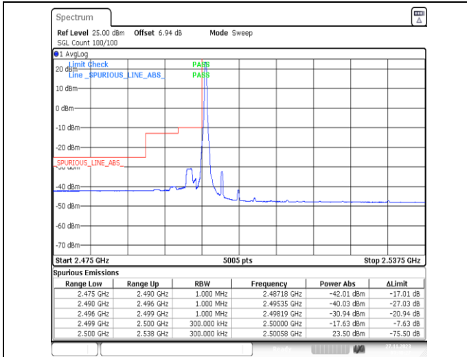
1-N7-PC3-15-25-L-1-DFT-PI2BPSK-Edge_1RB_Left-1 @0-Ant31-1--PASS-see graph
