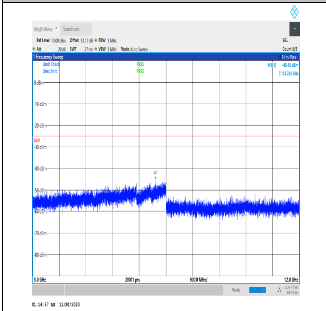
NTVN_N7_PC3_15_40_M_TID1_3000_12000_#1
