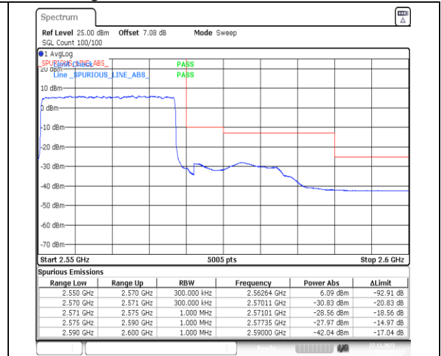
1-N7-PC3-15-20-H-3-DFT-PI2BPSK-Outer_Full-100@0-Ant31-1--PASS-see graph
