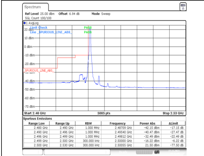
1-N7-PC3-15-20-L-4-CP-QPSK-Edge_1RB_Left-1 @0-Ant31-1--PASS-see graph
