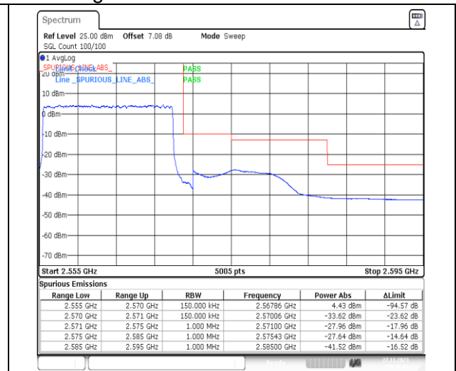
1-N7-PC3-15-15-H-3-DFT-PI2BPSK-Outer_Full-75@0-Ant31-1--PASS-see graph
