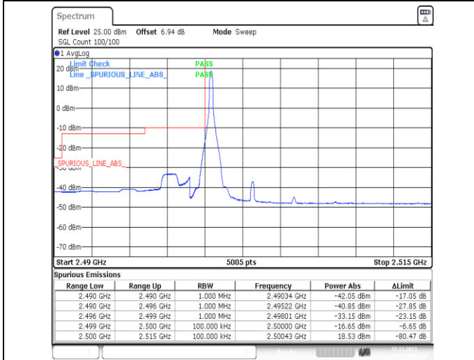
1-N7-PC3-15-10-L-4-CP-QPSK-Edge_1RB_Left-1 @0-Ant31-1--PASS-see graph
