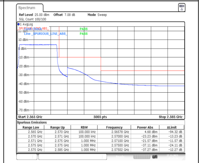
1-N7-PC3-15-5-H-6-CP-QPSK-Outer_Full-25 @0-Ant31-1--PASS-see graph
