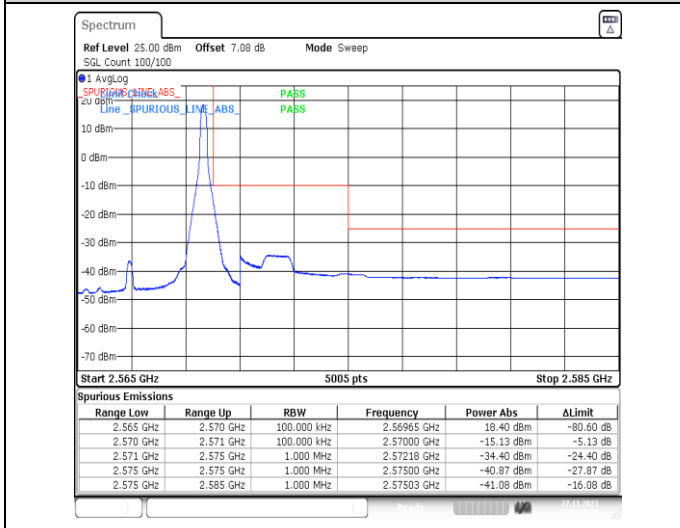
1-N7-PC3-15-5-H-5-CP-QPSK-Edge_1RB_Right-1 @24-Ant31-1--PASS-see graph
