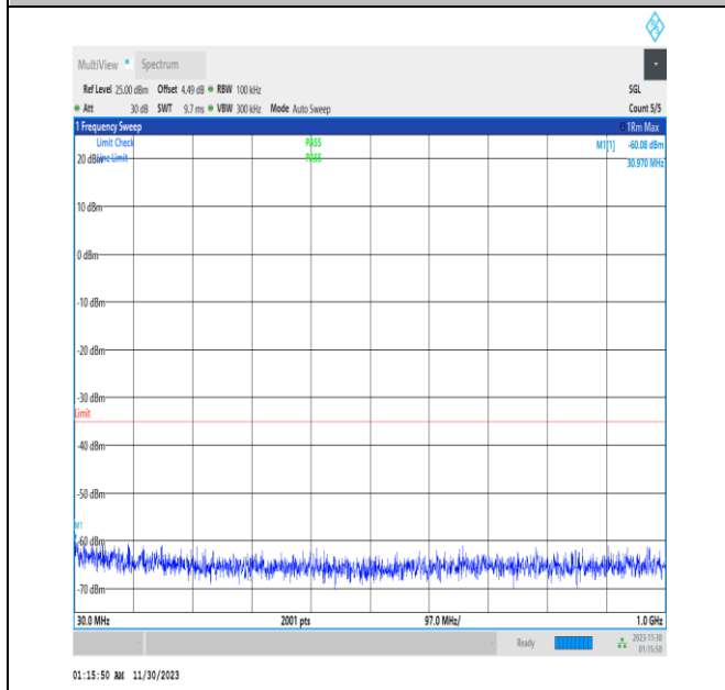
NTNV_N7_PC3_15_40_H_TID1_30_1000_#1
