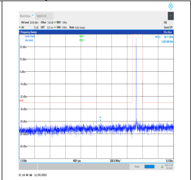
NTVN_N7_PC3_15_40_M_TID1_1000_3000_#1
