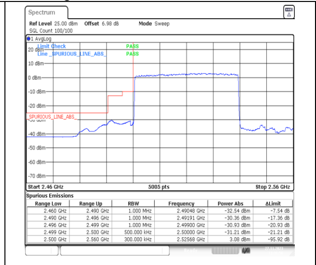
1-N7-PC3-15-40-L-3-DFT-PI2BPSK-Outer_Full-21 6@0-Ant31-1--PASS-see graph
