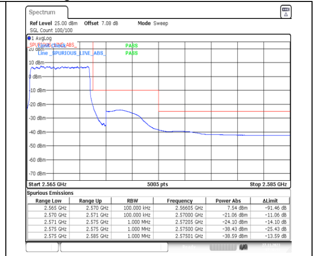
1-N7-PC3-15-5-H-3-DFT-PI2BPSK-Outer_Full-25 @0-Ant31-1--PASS-see graph
