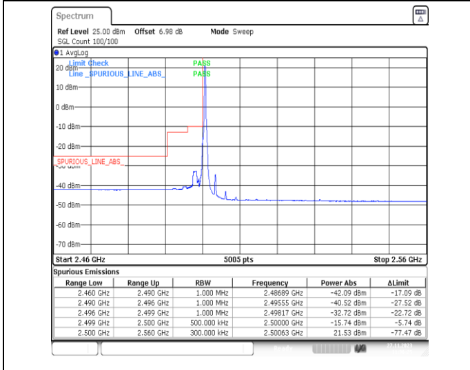
1-N7-PC3-15-40-L-4-CP-QPSK-Edge_1RB_Left-1@0-Ant31-1--PASS-see graph
