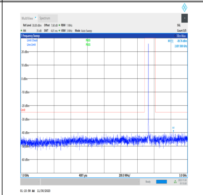
NTNV_N7_PC3_15_40_H_TID1_1000_3000_#1
