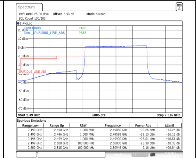
1-N7-PC3-15-10-L-6-CP-QPSK-Outer_Full-52 @0-Ant31-1--PASS-see graph
