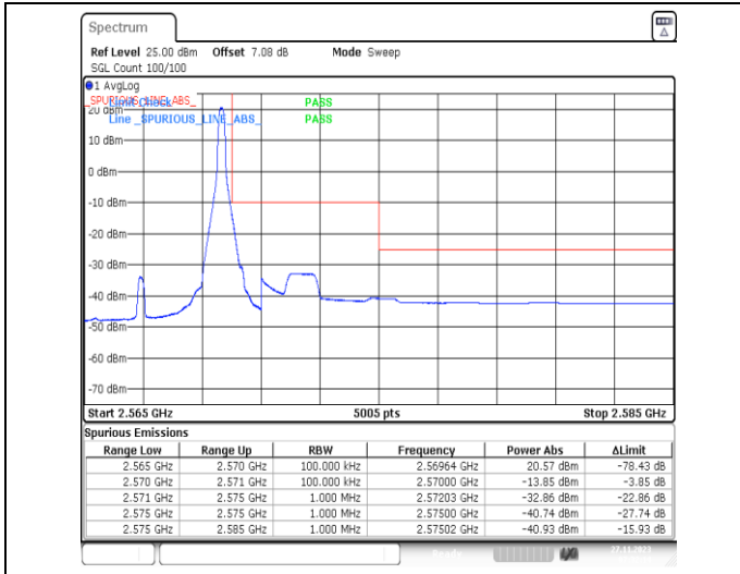
1-N7-PC3-15-5-H-2-DFT-PI2BPSK-Edge_1RB_Right-1 @24-Ant31-1--PASS-see graph
