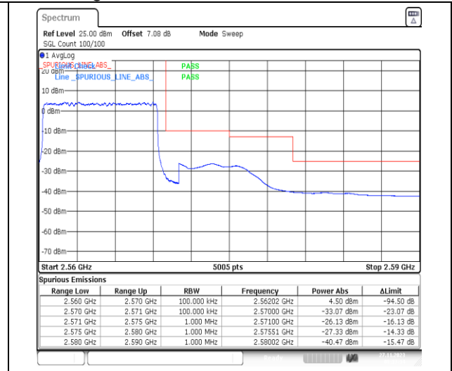
1-N7-PC3-15-10-H-3-DFT-PI2BPSK-Outer_Full-50@0-Ant31-1--PASS-see graph
