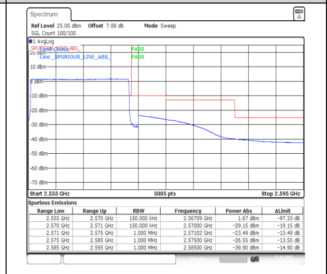
1-N7-PC3-15-15-H-6-CP-QPSK-Outer_Full-79@0-Ant31-1--PASS-see graph
