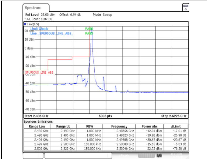
1-N7-PC3-15-15-L-1-DFT-PI2BPSK-Edge_1RB_Left-1 @0-Ant31-1--PASS-see graph
