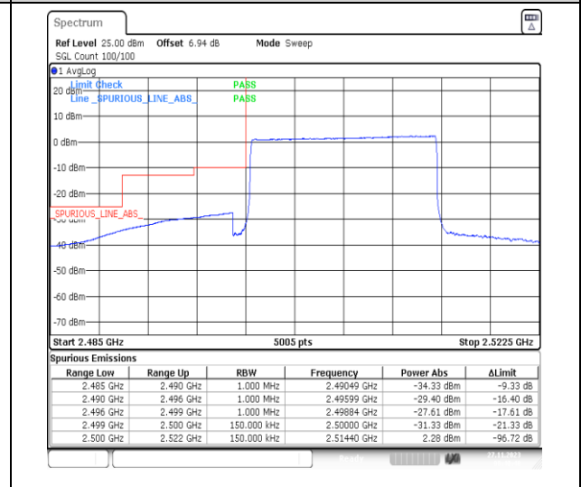
1-N7-PC3-15-15-L-6-CP-QPSK-Outer_Full-79 @0-Ant31-1--PASS-see graph
