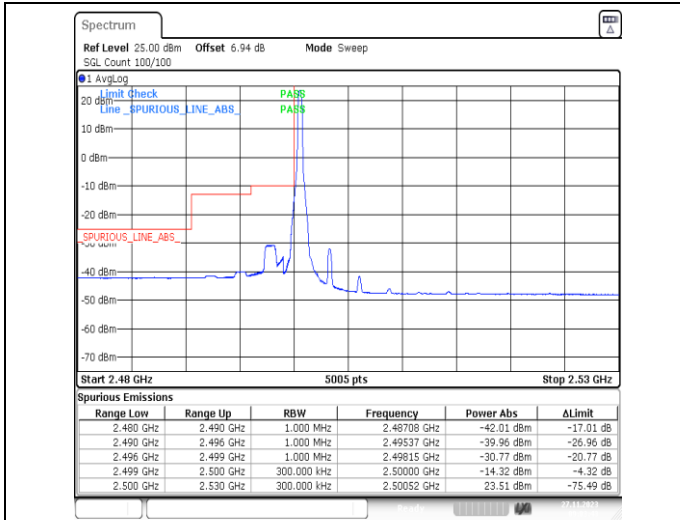
1-N7-PC3-15-20-L-1-DFT-PI2BPSK-Edge_1RB_Left-1 @0-Ant31-1--PASS-see graph
