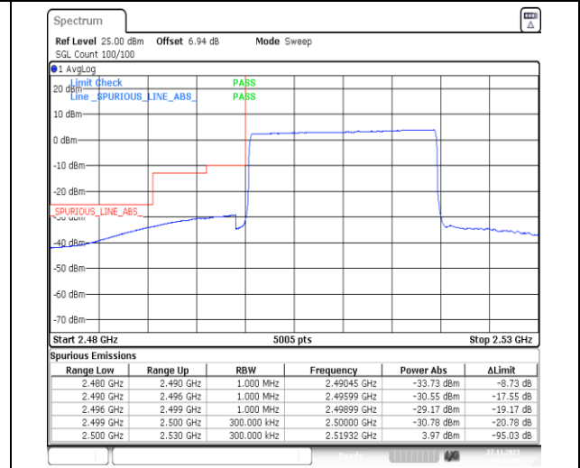
1-N7-PC3-15-20-L-6-CP-QPSK-Outer_Full-106 @0-Ant31-1--PASS-see graph
