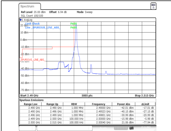
1-N7-PC3-15-10-L-1-DFT-PI2BPSK-Edge_1RB_Left-1 @0-Ant31-1--PASS-see graph
