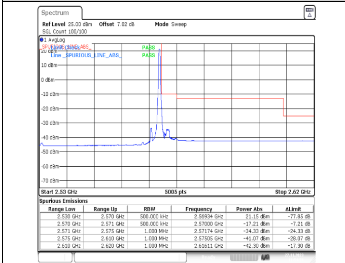
1-N7-PC3-15-40-H-2-DFT-PI2BPSK-Edge_1RB_Right-1@215-Ant31-1--PASS-see graph
