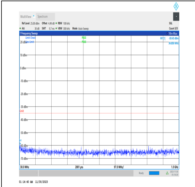
NTVN_N7_PC3_15_40_M_TID1_30_1000_#1
