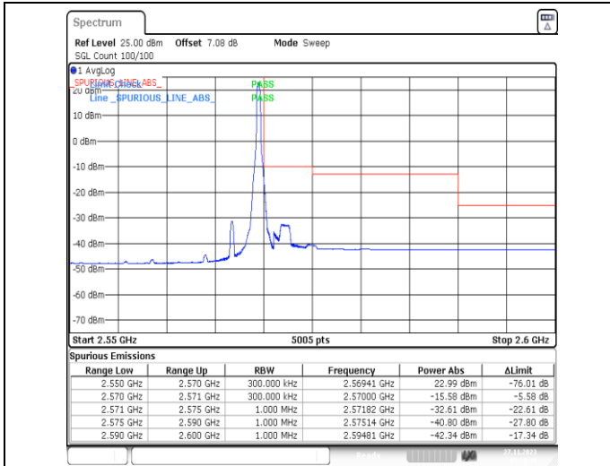
1-N7-PC3-15-20-H-2-DFT-PI2BPSK-Edge_1RB_Right-1@105-Ant31-1--PASS-see graph
