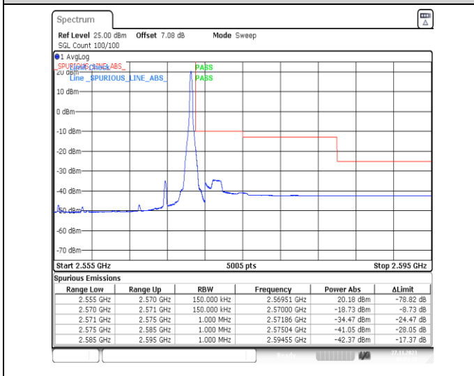
1-N7-PC3-15-15-H-5-CP-QPSK-Edge_1RB_Right-1@78-Ant31-1--PASS-see graph
