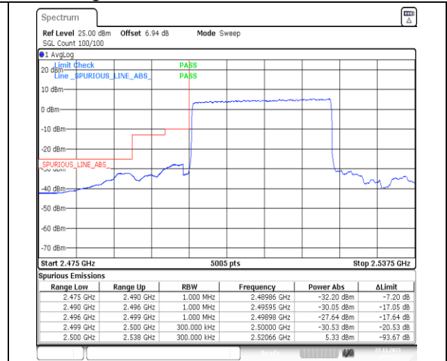
1-N7-PC3-15-25-L-3-DFT-PI2BPSK-Outer_Full-12 8@0-Ant31-1--PASS-see graph
