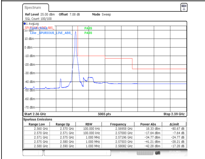
1-N7-PC3-15-10-H-5-CP-QPSK-Edge_1RB_Right-1@51-Ant31-1--PASS-see graph
