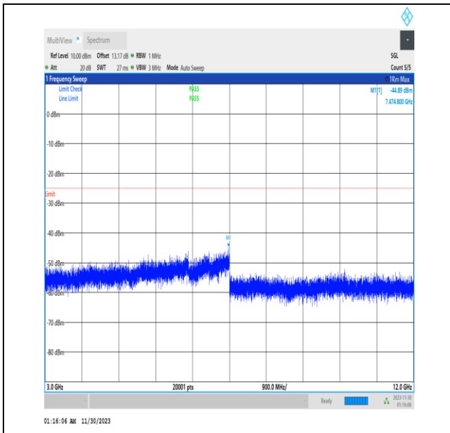
NTNV_N7_PC3_15_40_H_TID1_3000_12000_#1
