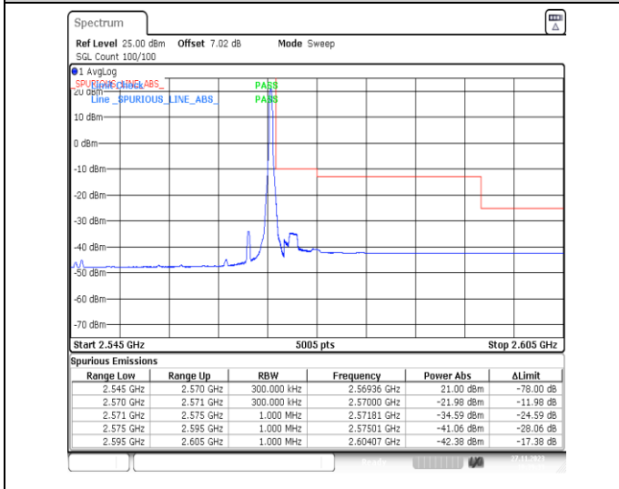
1-N7-PC3-15-25-H-5-CP-QPSK-Edge_1RB_Right-1@132-Ant31-1--PASS-see graph
