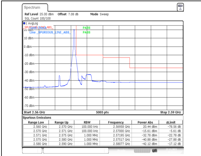
1-N7-PC3-15-10-H-2-DFT-PI2BPSK-Edge_1RB_Right-1@51-Ant31-1--PASS-see graph
