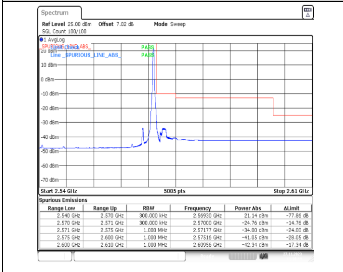
1-N7-PC3-15-30-H-5-CP-QPSK-Edge_1RB_Right-1@159-Ant31-1--PASS-see graph
