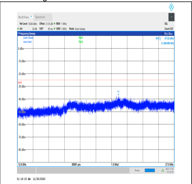
NTNV_N7_PC3_15_40_H_TID1_12000_27000_#1
