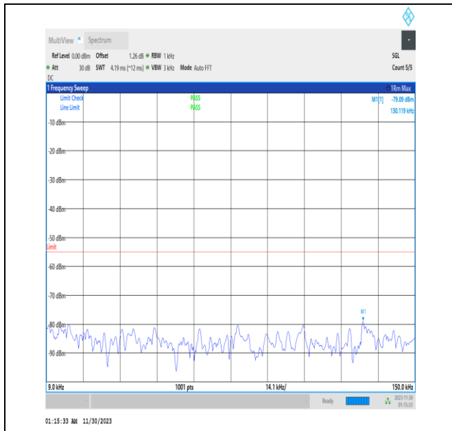
NTNV_N7_PC3_15_40_H_TID1_0.009_0.15_#1
