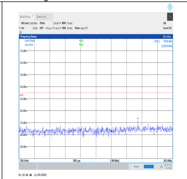
NTNV_N7_PC3_15_40_H_TID1_0.15_30_#1
