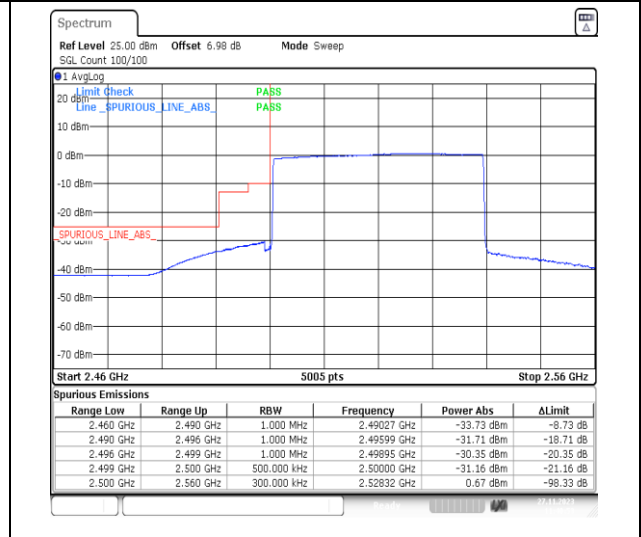
1-N7-PC3-15-40-L-6-CP-QPSK-Outer_Full-216@0-Ant31-1--PASS-see graph
