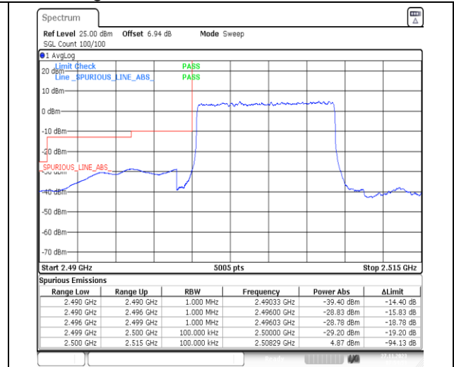
1-N7-PC3-15-10-L-3-DFT-PI2BPSK-Outer_Full-50 @0-Ant31-1--PASS-see graph
